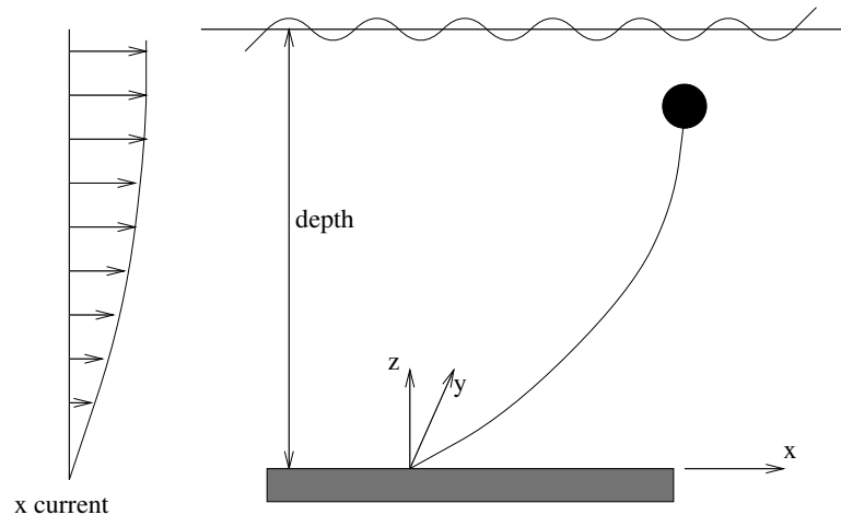
Figure 2.1: Geometric definitions for cablc .
