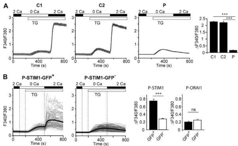
Figure 3. Abolished Ca^{2+} influx in the patient's EBV-B cells is restored by expression of STIM1. (A) EBV-B cells of the patient (P) and two controls (C1 and C2) were stimulated with 1 \mu M thapsigargin (TG) in Ca^{2+} -free Ringer solution (open bars) followed by perfusion with 2 mM Ca^{2+} (filled bars) to induce Ca^{2+} influx. Traces represent mean F340/F380 emission ratios of one representative experiment. Averages on the right are from n = 6 (C1), n = 4 (C2), n = 5 (P) experiments. \Delta F340/F380 represents peak [Ca^{2+}]_i , 25 s after readdition of Ca^{2+} minus baseline [Ca^{2+}]_i at the beginning of the recording. Error bars represent the SEM. ***, P < 0.0001 . (B) EBV-B cells from the patient were retrovirally transduced with STIM1-IRES-GFP expression vector (P-STIM1) or ORAI1-IRES-GFP vector (P-ORAI1). Ca^{2+} levels were measured as described in A. Traces of individual cells (thin gray lines) and averages of all cells (thick black lines) are shown for 90 GFP + and 90 GFP - cells. Averages of peak \Delta F340/F380 from total 368 cells (P-STIM1; n = 6 experiments) or 482 cells (P-ORAI1; n = 10 experiments) are shown in the bar graph. Error bars represent the SEM. ***, P < 0.0001 ; ns, P > 0.05 .
