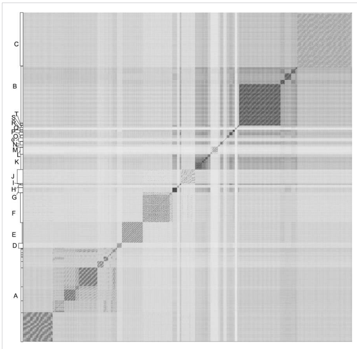
Figure 2. Nucleotide sequence comparison of 627 mycobacteriophages displayed as a dotplot. Complete genome sequences of 627 mycobacteriophages were concatenated into a single file which was compared with itself using Gepard (Krumstiek et al. , 2007) and displayed as a dotplot using default parameters (word length, 10). The order of the genomes is as listed in Supplementary file 1 . Nucleotide similarity is a primary component in assembling phages into clusters, which typically requires evident DNA similarity spanning more than 50% of the genome lengths.
