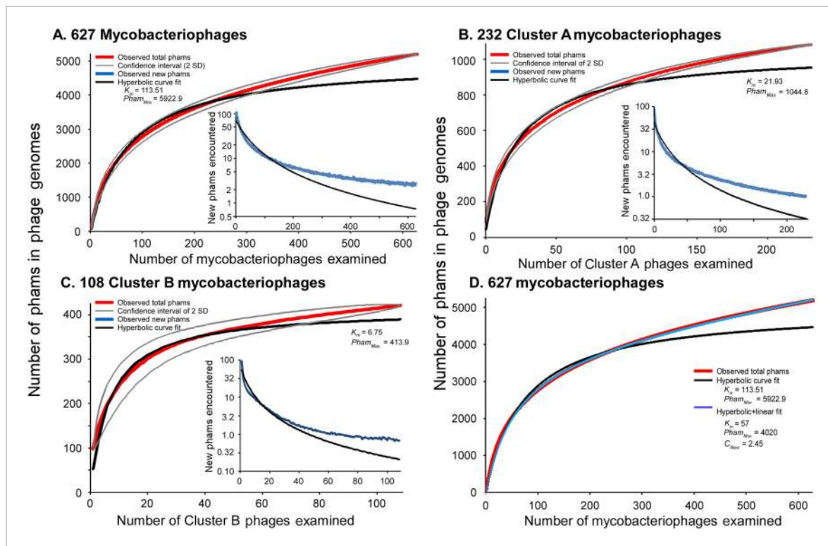
Figure 7. Rarefaction analysis of mycobacteriophage genomes. (A) The numbers of phamilies are reported for between 1 and 627 phage genomes sampled at random without replacement; the mean of 10,000 iterations is shown in red; gray lines indicate a confidence interval of two standard deviations. The black line shows a hyperbolic curve fit to the data from phage counts 1 to 314. The inset shows the number of new phams encountered upon the inclusion of each phage, with the mean number for the 10,000 iterations shown in blue and the predicted value from the hyperbolic curve shown in black. (B) Rarefaction analysis of 232 Cluster A phages. The total numbers of phamilies are reported for between 1 and 232 phages sampled at random without replacement from Cluster A; the mean of 10,000 iterations is shown in red; gray lines indicate a confidence interval of two standard deviations. The black line shows a hyperbolic curve fit to the data from phage counts 1 to 117. The inset shows the number of new phams encountered upon the inclusion of each phage, with the mean number for 10,000 iterations shown in blue and the predicted value from the hyperbolic curve shown in black. (C) Rarefaction analysis of 108 Cluster B phages; the hyperbolic curve was fit to the data from phage counts 1 to 54. (D) Fits of the hyperbolic ( Equation 1 ) and hyperbolic with linear ( Equation 2 ) models for phamily identification within genome samples.
