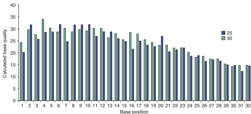
Figure 3 | Position dependency of base calling accuracy for N2 Bristol Solexa single-end reads. The calculated based quality is shown as a distribution at phred base quality 25 or at base quality 30.
