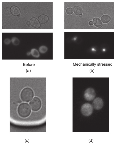
Fig. S3. (A) Cells between a glass slide and layer of PDMS (with a 40- \mu\text{m} distance); here Msn2 is localized in the cytoplasm. (B) The same cells after applying severe external pressure on the PDMS layer; here Msn2 localizes to the nucleus indicating that Msn2 localization can indeed indicate physical stress. (C) Bright-field and (D) fluorescent images of cells under a PDMS elastic pad of our microfluidic chip, where Msn2 is localized in the cytoplasm. A potential issue with our setup could have been stress imposed on the cells by the mechanical force applied by the micropad. Generally, we did not expect the cells to be stressed because a similar type of micropad has already been used for budding yeast cells without this complication (1–3); however, we aimed to show experimentally that the setup indeed does not stress the cells. For this purpose, we used a yeast strain that had a GFP fused to the general stress-responsive transcriptional activator Msn2. Msn2 localizes to the nucleus under stress conditions (4). We found that the Msn2-GFP protein is localized in the cytoplasm of cells underneath the micropad. In a control experiment in which we manually squeezed the PDMS pad and thus the cell, the fusion protein localized to the nucleus, indicating that during regular operation of the chip, the cells are not stressed.
