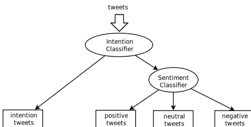
Figure 1: Tweet Classification
