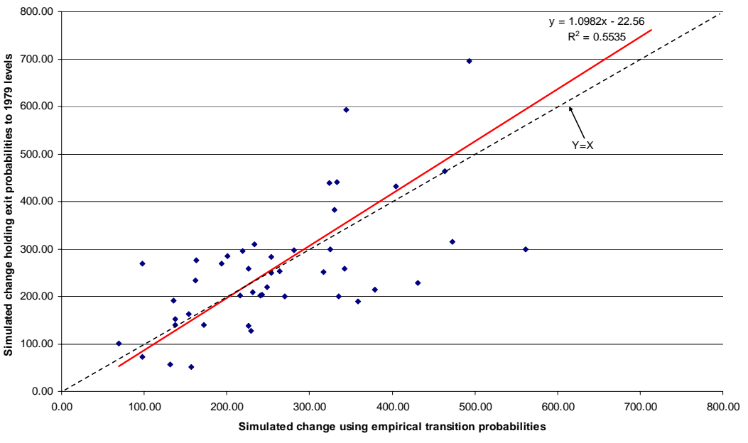
Scatter plot of simulated changes in state-level incarceration rates (1979 to 1998) holding exit probabilities constant against simulated changes using empirical transition probabilities
