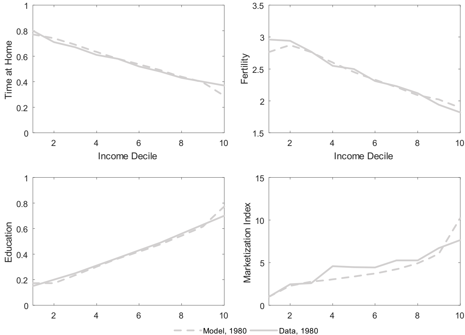
Figure 6: Model Fit
