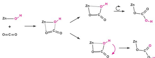
Scheme 8 Proposed pathways for the activation of \text{CO}_2 by carbonic anhydrase. Upper sequence: Lindskog mechanism. Lower sequence: Lipscomb mechanism.
