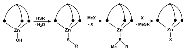
Scheme 7 Stepwise reaction sequence for the alkylation of a thiol with \text{Tp}^*\text{Zn-OH} .
