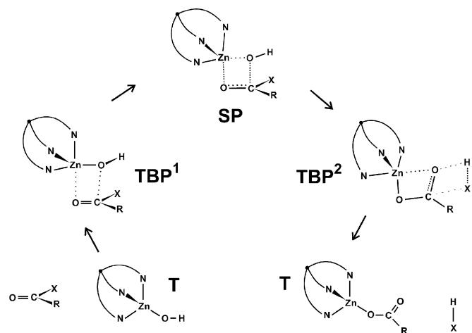
Scheme 11 Mechanistic pathway, as derived from structure correlation analysis, for the cleavage of an ester or peptide by \text{Tp}^*\text{Zn-OH} . Abbreviations: T tetrahedral, TBP trigonal bipyramidal, SP square pyramidal.
