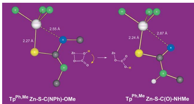
Fig. 5 Central parts of the structures of \text{Tp}^*\text{Zn} complexes resulting from the insertion of isothiocyanates into the Zn–OMe (left) and Zn–OH (right) as models for the Lipscomb interconversion (inset).
