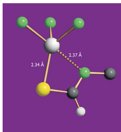
Fig. 3 Central part of the structure of \text{Tp}^{\text{Ph,Me}}\text{Zn-S-CH=NC}_6\text{H}_4\text{NO}_2 , resulting from the insertion of \text{RNCS} into \text{Tp}^{\text{Ph,Me}}\text{Zn-H} .
