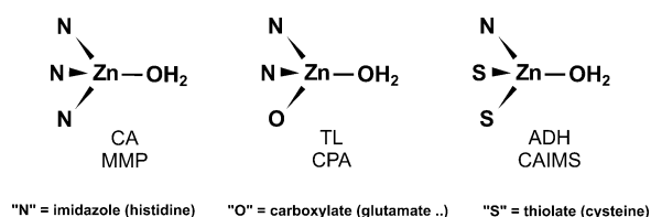
Scheme 3 Coordination motifs in the resting states of zinc enzymes. Abbreviations: CA carbonic anhydrase, MMP matrix metalloproteases, TL thermolysin, CPA carboxypeptidase A, ADH alcoholdehydrogenase, CAIMS cobalamine independent methionine synthase. As a result of the charge of the amino acid ligands the overall charge of the “zinc complexes” is +2 for the first group, +1 for the second and 0 for the third group.
