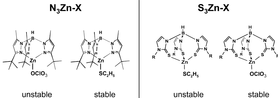
Scheme 2 Hard–hard, soft–soft, and hard–soft ligand combinations in tripod zinc complexes.
