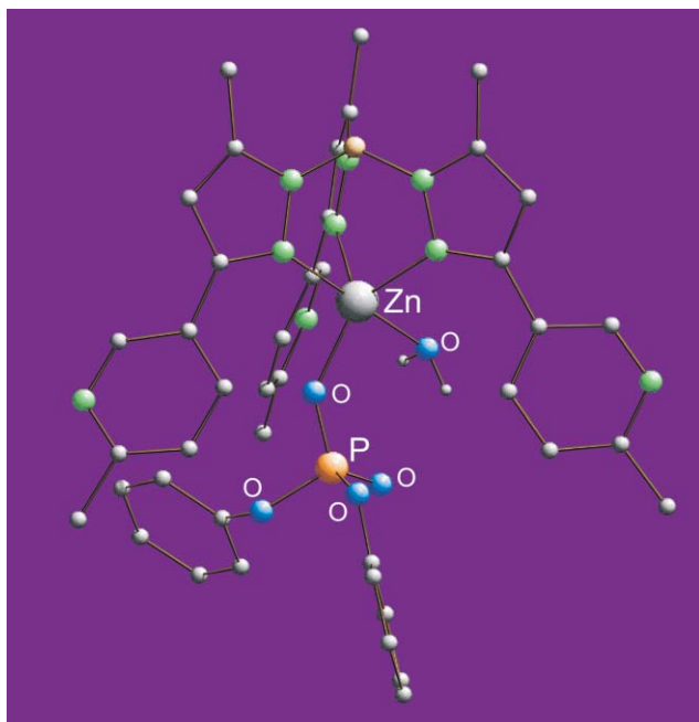
Fig. 2 Ball and stick representation of the enzyme-substrate model \text{Tp}^{\text{Py,Me}}\text{Zn}(\text{OH}_2)\text{OPO}(\text{OPh})_2 .
