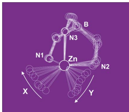
Fig. 6 Structure correlation by the superposition of the immediate zinc coordinations of eight \text{Tp}^*\text{Zn}(\text{X})(\text{Y}) complexes.
