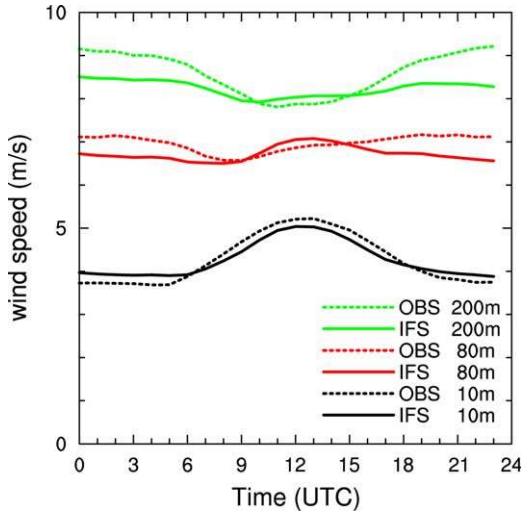
Figure 3. Annually averaged diurnal cycle of wind in Cabauw (Netherlands) at 10, 80, and 200 m of height for 2011. The operational ECMWF IFS (deterministic high resolution T1279 L91 run, cycles 37r2 and 37r3) daily 0000 UTC forecasts (lead times 24–42 h) are compared to observations.
