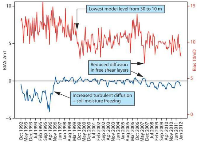
Figure 2. Historic evolution of 2 m temperature (blue curve) and 10 m wind direction errors (red curve) of the operational ECMWF IFS. These are monthly values of mean errors at a lead time of 60 h of the daily forecasts initialized at 1200 UTC (verifying time 0000 UTC). The verification includes 800 SYNOP stations over Europe (30–72°N, 22°W–42°E).
