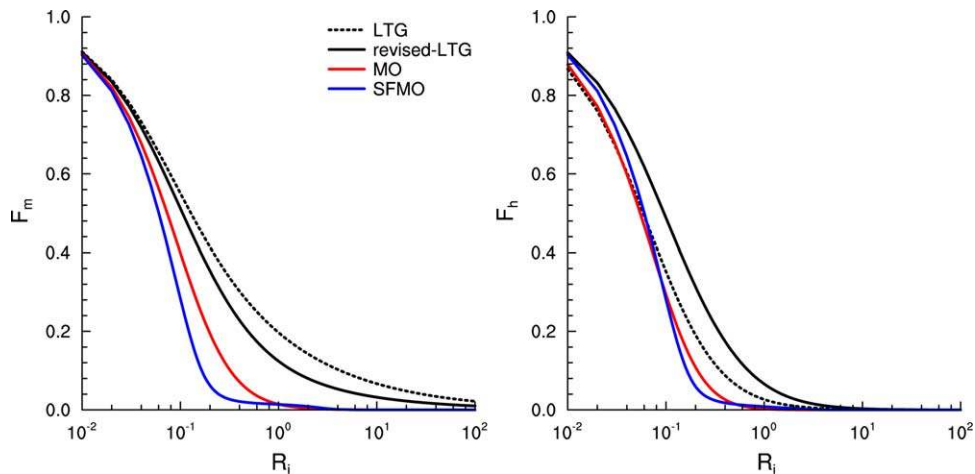
Figure 1. Stability functions for momentum and heat: original Louis functions (black dotted line), Monin-Obukhov functions used in the surface layer (blue line), revised Louis functions used close to the surface (black line) and Monin-Obukhov functions used further away from the surface (red line).
