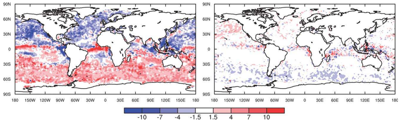
Figure 7. (left) Mean first-guess departure (observations — model) of wind direction at the surface (degrees) with respect to ASCAT observations in a CTL analysis run performed for January 2011 and (right) the mean change in these first-guess departures when the LT30 formulation for turbulent diffusion in stable conditions is used instead of the CTL formulation. These quantities represent the average over the 0000 and 1200 UTC analyses.
