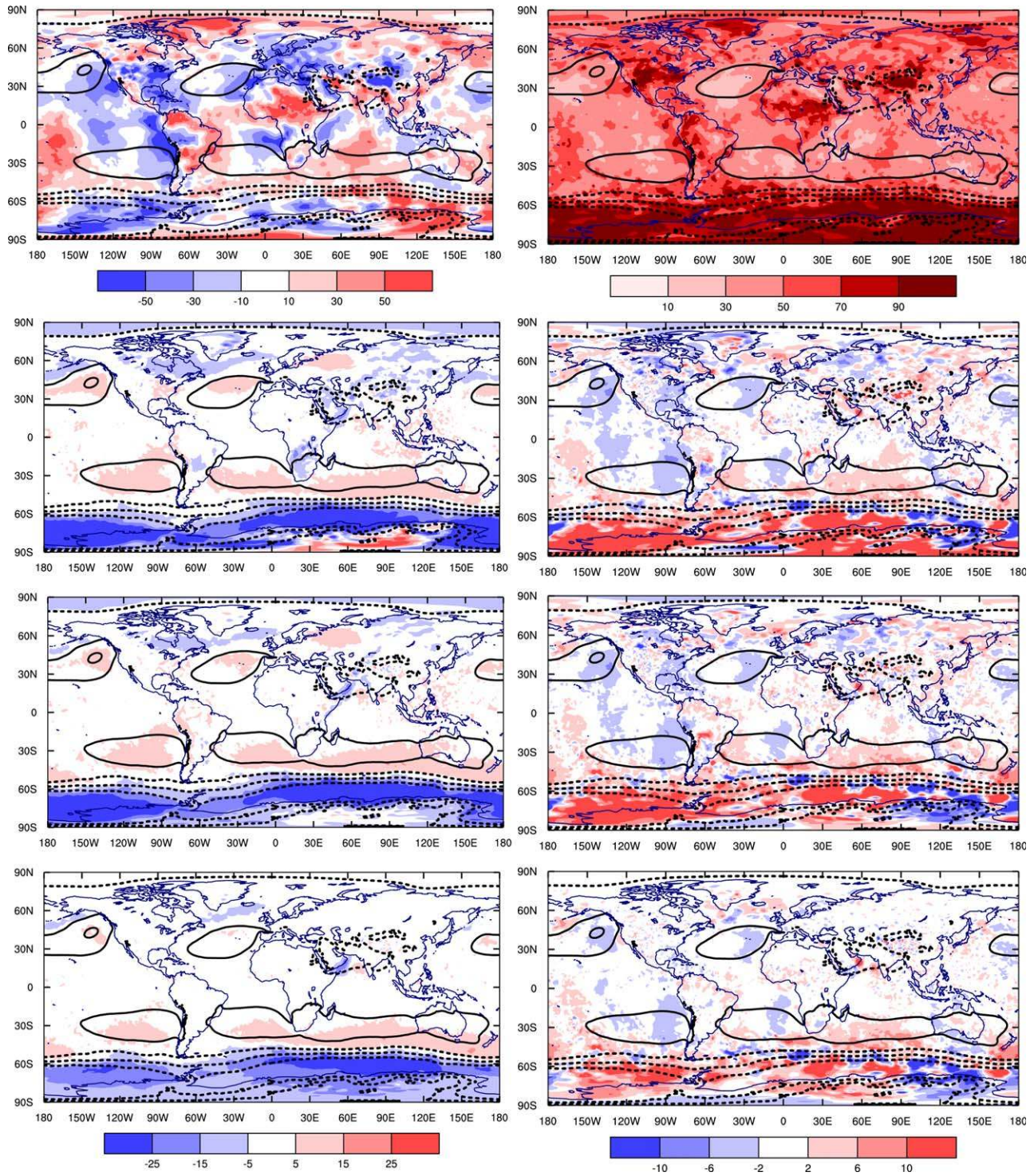
Figure 10. Mean 1000 hPa geopotential (top left) height bias and (top right) RMSE of the CTL experiment for July 2010, with respect to the analyses from which the forecasts were initialized, at forecast step 24 (verifying at 0000 UTC). Second to fourth row: Change in (left) mean and (right) RMSE of the 1000 hPa geopotential height in the runs ST, LT30, LT30-SEA with respect to the CTL run (all in meters). A decrease in bias and RMSE indicates an improvement of the model performance.
