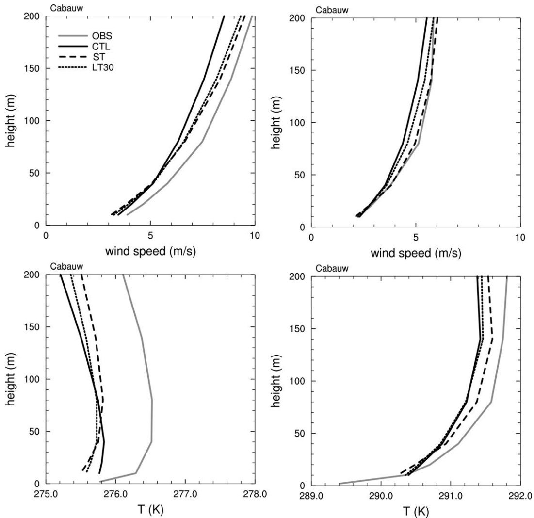
Figure 5. Mean (top) wind speed and (bottom) temperature obtained from the ST (dashed), LT30 (dotted) and CTL (full) experiments performed for (left) January 2011 and (right) July 2010 and from the observations realized at the Cabauw tower (gray). The modeled profiles correspond to lead time 24 h of the daily 0000 UTC forecasts (verifying at 0000 UTC).
