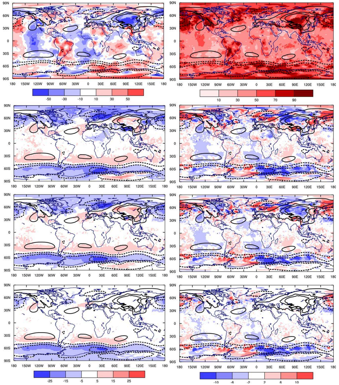
Figure 9. Mean 1000 hPa geopotential (top left) height bias and (top right) RMSE of the CTL experiment for January 2011, with respect to the analyses from which the forecasts were initialized, at forecast lead time 24 h (verifying at 0000 UTC). Second to fourth row: Change in (left) mean and (right) RMSE of the 1000 hPa geopotential height in the runs ST, LT30, LT30-SEA with respect to the CTL run (all in meters). A decrease in bias and RMSE indicates an improvement of the model performance.
