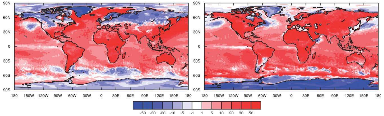
Figure 6. Mean sensible heat flux for the CTL experiments performed for (left) January 2011 and (right) July 2010, derived from the average over the first 24 h of the daily 0000 UTC forecasts.
