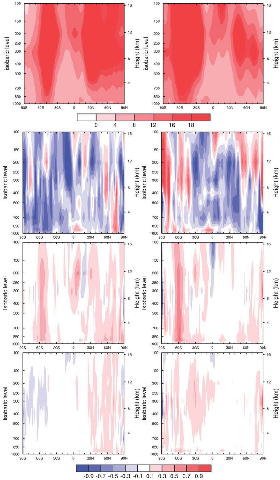
Figure 8. (top to bottom) Zonal mean wind speed in the CTL run; zonal mean wind speed bias in the CTL run with respect to the analyses from which the forecasts were initialized; changes in the zonal mean wind speed in the LT30 compared to the CTL run; and changes in the wind speed RMSE in the LT30 compared to the CTL run, with respect to the analyses from which the forecasts were initialized (all in meters per second). All the plots correspond to lead time 120 h (day 5) of the 0000 UTC forecasts performed for (left) January 2011 and (right) July 2010.
