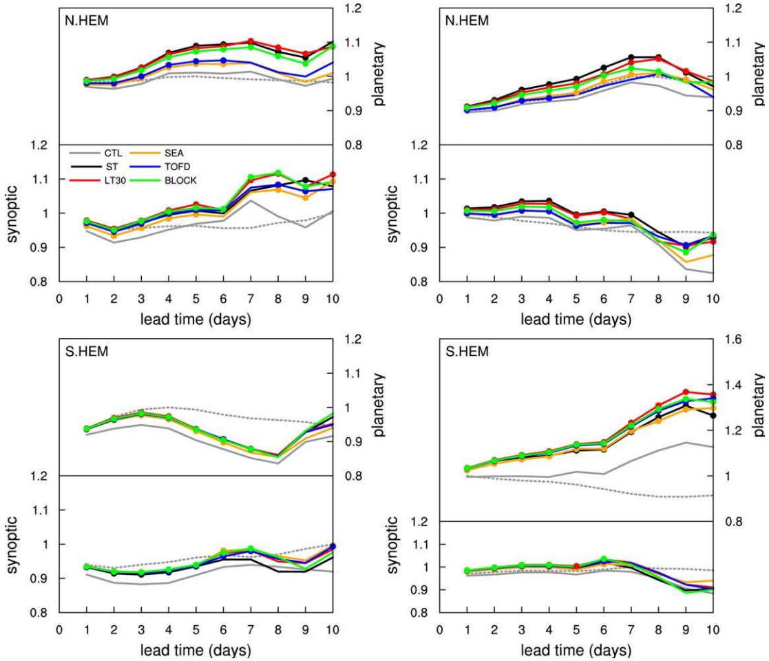
Figure 11. Model activity in terms of geopotential height at 1000 hPa at (lower) synoptic and (upper) planetary scales for the (top) Northern and (bottom) Southern Hemispheres for the various runs performed for (left) January 2011 and (right) July 2010. The dashed gray line indicates in each case the activity in the analyses from which all the forecasts are initialized. The activity is computed with respect to a climatology, i.e., 2(a - c)^2 , or 2(f - c)^2 , and in the panels is normalized for all runs by the maximum during the 10 days of the activity in the analyses (at synoptic and planetary scale, respectively). When present, the dots indicate that the respective experiment is significantly (95 % confidence interval) better or worse than the CTL, that is the activity in the forecast is closer or further to the one in the analyses than in the CTL run.
