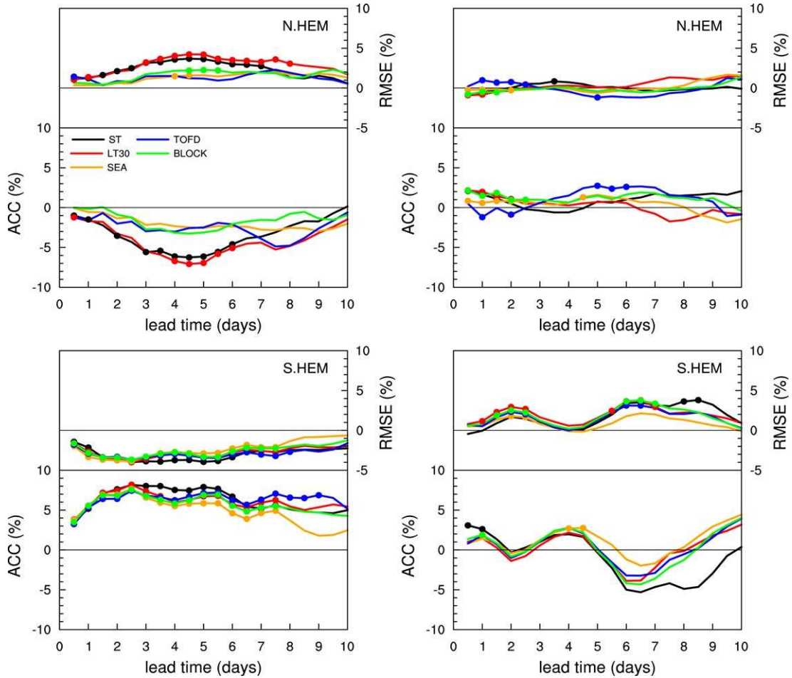
Figure 12. Relative difference of forecast anomaly correlation (ACC) and RMSE of 500 hPa geopotential height, between the different experiments and the CTL forecasts performed for (left) January 2011 and (right) July 2010, for the (top) Northern and (bottom) Southern Hemispheres. When present, the dots indicate that the respective experiment is significantly better/worse (95% interval) than the CTL. A negative/positive difference in ACC/RMSE indicates a deterioration of the model performance in the experiment with respect to the CTL.
