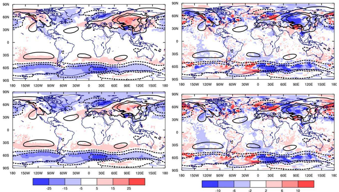
Figure 13. Change in (left) mean and (right) RMSE of the 1000 hPa geopotential height at forecast step 24 h (verifying at 0000 UTC) in the runs LT30-TOFD, LT30-BLOCK compared to the CTL run performed for January 2011 (in meters).
