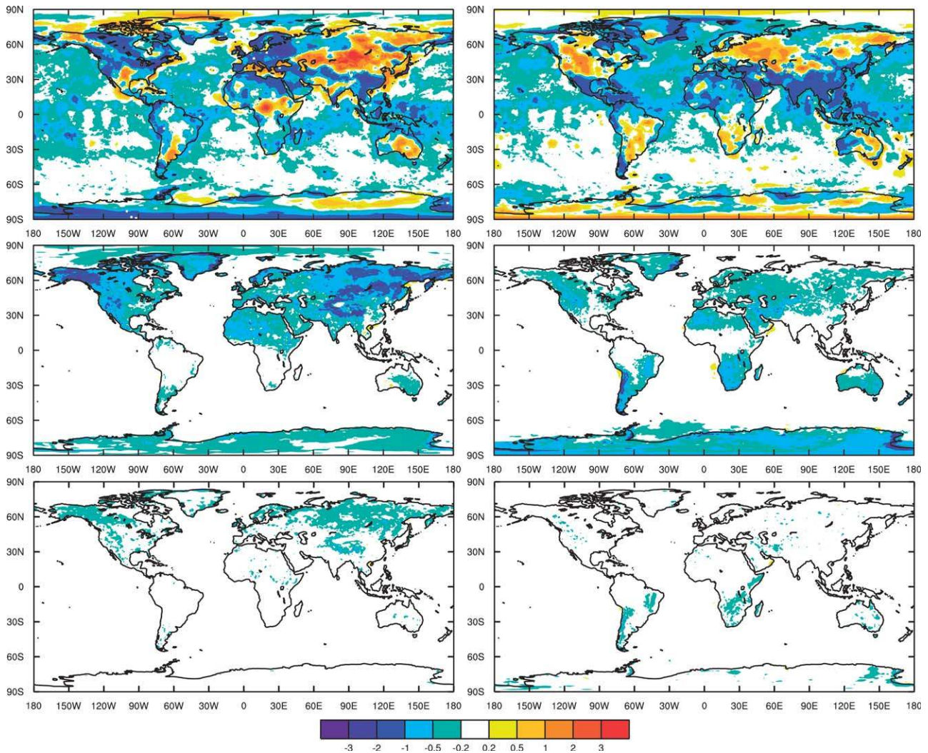
Figure 4. Mean 2 m temperature error ( K ) for the CTL daily forecasts performed for (top left) January 2011 and (top right) July 2010, with respect to the analyses from which the forecasts were initialized. Mean change in 2 m temperature in the experiments ST with respect to the CTL experiments for (middle left) January 2011 and (middle right) July 2010. (Bottom) Same as for middle but for experiment LT30. All quantities are plotted at the time of the minimum of the diurnal cycle in 2 m temperature derived from the lead times 24–42 h of the daily 0000 UTC forecasts.
