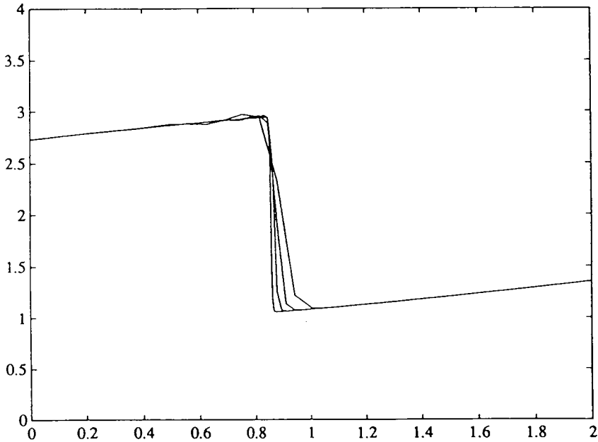
FIGURE 5b. Hybrid Lax-Wendroff scheme with van Leer scheme, t = 2, m = 100, 200, 400
