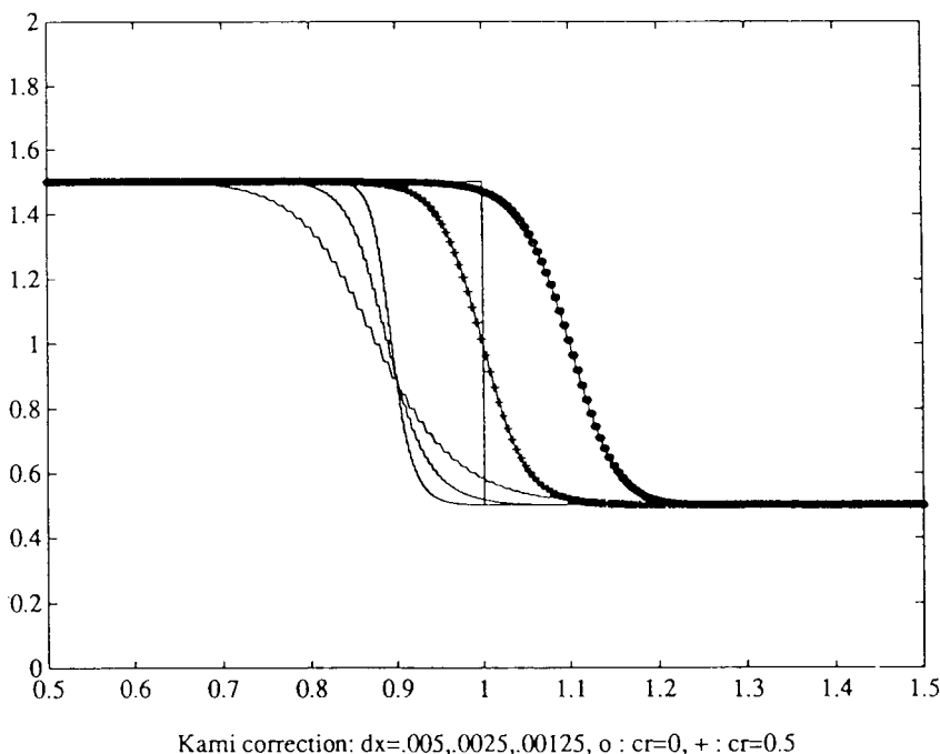
FIGURE 3. Lax-Friedrichs scheme in nonconservative form, t = 1
