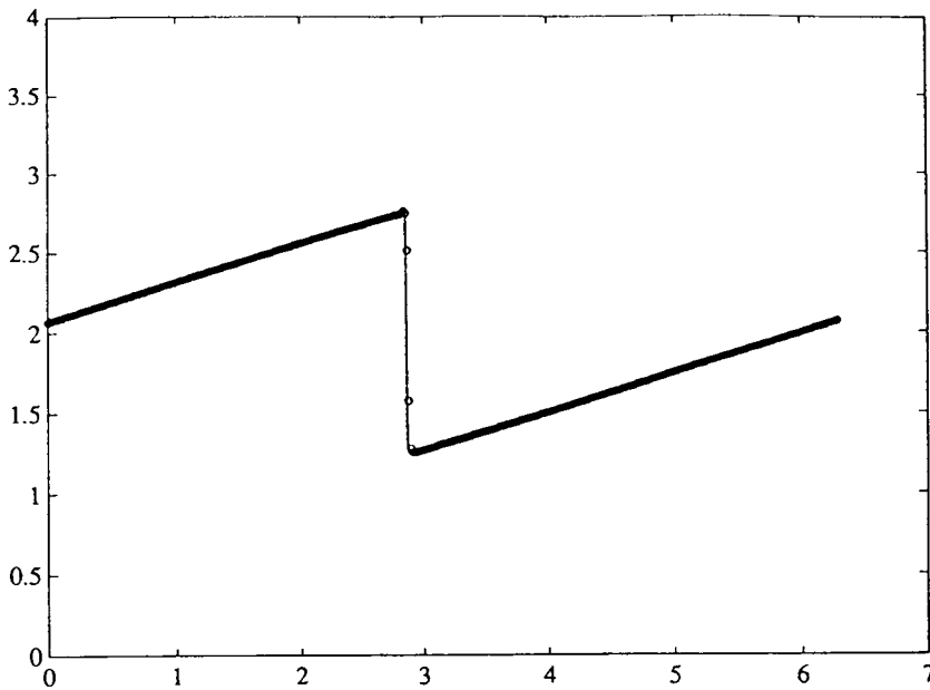
FIGURE 5c. Hybrid Lax-Wendroff scheme with van Leer scheme, t = 3, m = 400
