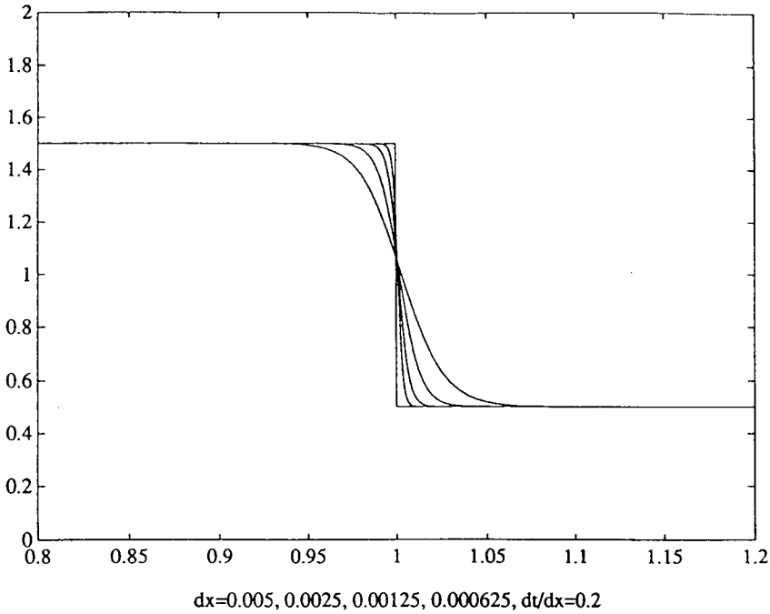
FIGURE 4a. Modified Lax-Friedrichs scheme in nonconservative form, t = 1
