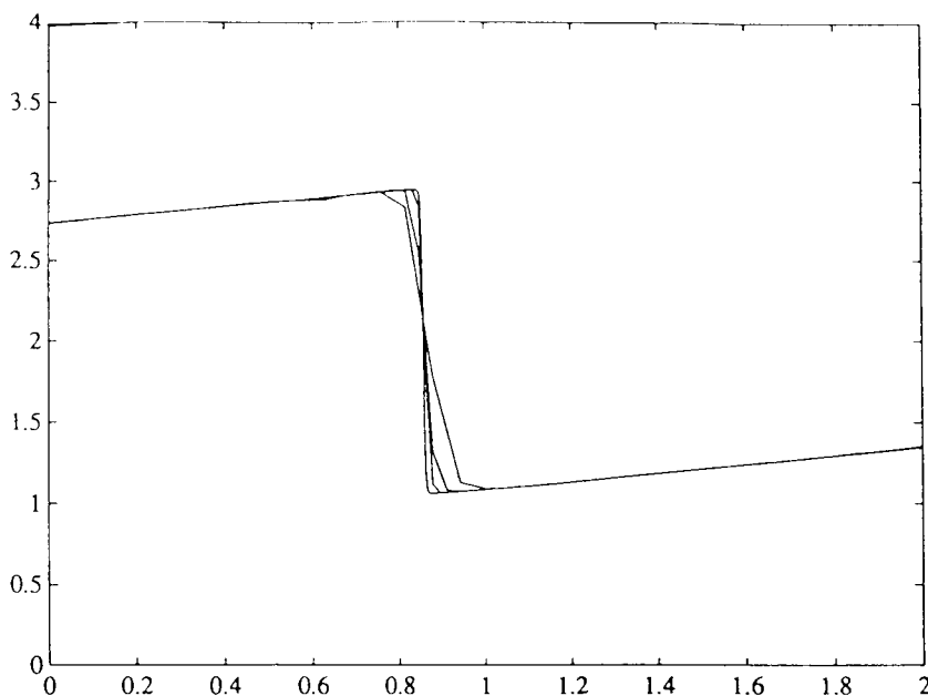
FIGURE 5a. Hybrid Lax-Wendroff scheme with van Leer scheme, t = 2 , m = 100, 200, 400
