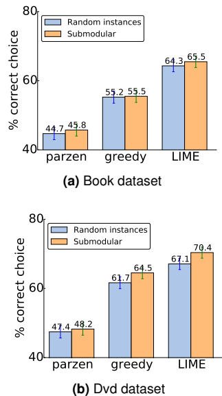
Figure 4: Choosing between two classifiers based on trust, after seeing k = 10 examples.
