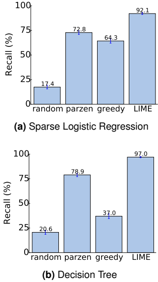
Figure 3: Recall on true explanations for transparent classifiers on the book dataset.
