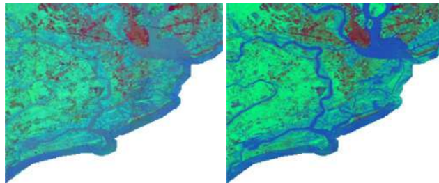
Figure 8: (left) A false-color image generated by applying the Places network to aerial imagery. In both images the colors are semantically meaningful (red=urban, green=rural, blue=water-related). (right) The same as (left) but with our CVPlaces network (trained on the entire USA dataset, with no Charleston-specific fine tuning).
