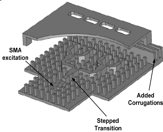
Fig.4 Complete linear array geometry. the upper plate is shown lifted and partly removed for clarity.
