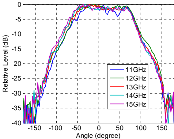
Fig.16 (b) Measured E plane radiation patterns for the linear array.
