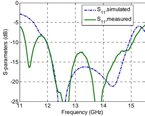
Fig.15 Measured and simulated S_{11} for the 2 \times 2 element planar array antenna.
