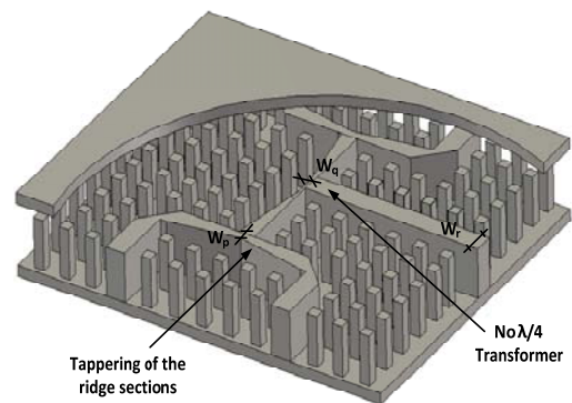
Fig. 8 (a) Schematic of the modified T-junctions and 4-way power divider, W_r = 2\text{mm} , W_p = 0.7\text{mm} and W_n = 1.15\text{mm} .
