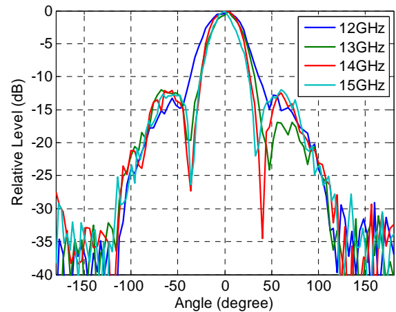
Fig.17 (a) Measured H plane radiation patterns for the planar array.
