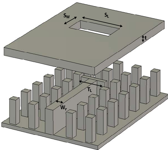
Fig. 7 (a) Schematic of the modified slot element; S_L = 11.45\text{mm} , S_W = 6.25\text{mm} , T_L = 6.75\text{mm} , W_r = 2\text{mm} and t = 2\text{mm} . The upper plate is shown lifted.
