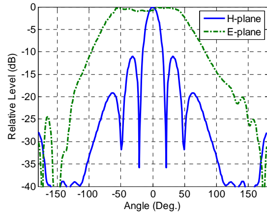
Fig.6 Simulated radiation patterns for the linear array at 13GHz.
