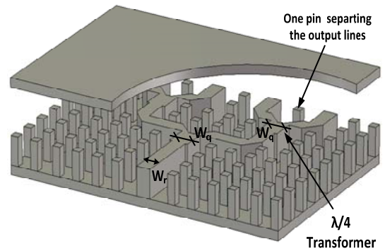
Fig.3 (b) 4-way power divider with the T-junctions; W_r = 3\text{mm} , W_g = 4.2\text{mm} . The upper plate is shown lifted up and partly removed for clarity.
