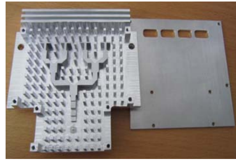
Fig.12 Manufactured prototype of 4 \times 1 element linear array antenna.
