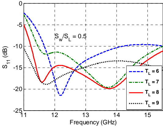
Fig.2 (c) Variation in parameter T_L of the T-shape section, S_w/S_L is kept 0.5.
