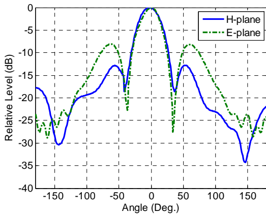
Fig.11 Simulated E-plane and H-plane radiation patterns for the planar array at 15GHz.
