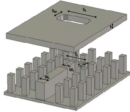
Fig.2 (a) Drawing of the slot element with T-section; S_L = 11.825 mm, S_W = 5.8 mm, T_L = 8.15 mm, T_S = 1 mm, W_r = 3 mm, W_t = 2 mm and t = 2 mm. The air gap between pins and the top plate is 1 mm, even though it is shown bigger in the drawing.
