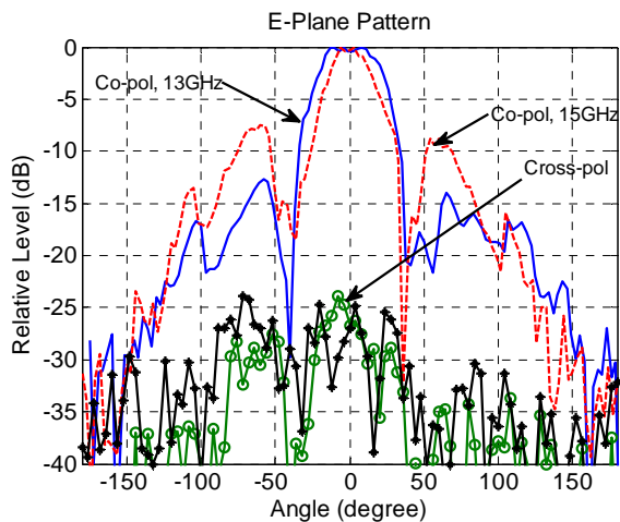
Fig.17 (c) Measured cross-polarization level for the planar array.
