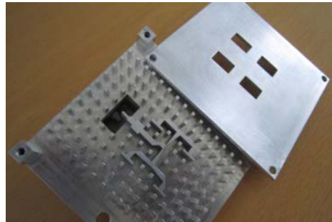
Fig.13 Manufactured prototype of 2 \times 2 element planar array antenna.
