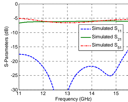
Fig. 8 (b) Simulated S-parameters for the compact 4-way power divider.
