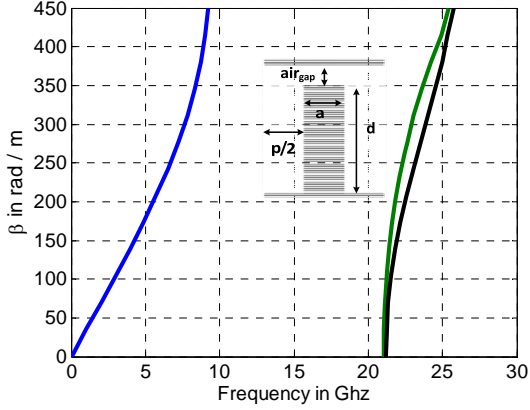
Fig.1 (b) Dispersion diagram of the unit cell of the periodic pins used in the linear array design, a = 2 mm, p/2 = 1.25 mm, d = 6 mm and air_{gap} = 1 mm.
