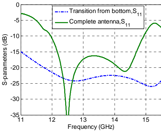
Fig.10 (b) Simulated S_{11} for the bottom transition from ridge gap waveguide to rectangular waveguide and the complete planar antenna.
