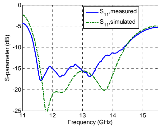
Fig.14 Measured and simulated S_{11} for the 4 \times 1 element linear array antenna.
