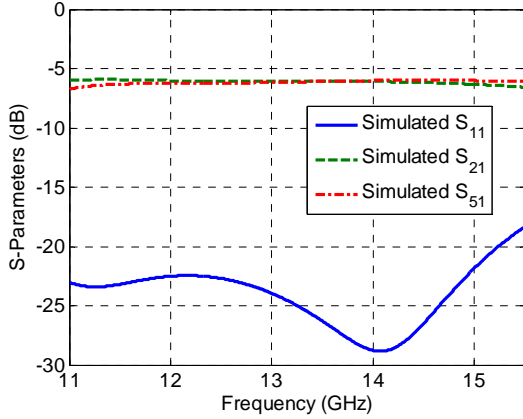
Fig.3 (c) Simulated results for the 4-way power divider.
