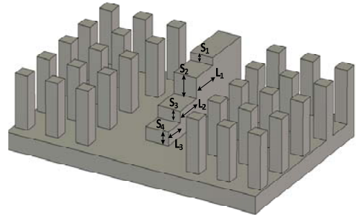
Fig.5 (a) Stepped transition from ridge gap waveguide to groove gap waveguide, S_1=0.85\text{mm} , S_2=2.45\text{mm} , S_3=1.35\text{mm} , S_4=1.6\text{mm} , L_1=4.6\text{mm} ; L_2=4.5\text{mm} , L_3=3.35\text{mm} (top metal plate not shown).
