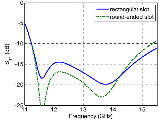
Fig.3 (a) Simulated S_{11} for the rounded edge slot element.
