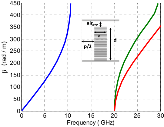
Fig.1 (c) Dispersion diagram of the unit cell of the periodic pins used in the planar array design, a = 1.75 mm, p/2 = 0.85 mm, d = 6.15 mm and air_{gap} = 1 mm.
