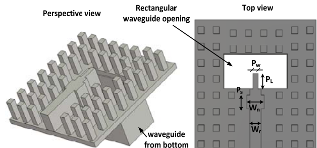
Fig. 9 Rectangular waveguide to ridge gap waveguide transition, P_L = 3.65\text{mm} , P_w = 1.25\text{mm} , P_s = 4.25\text{mm} , W_n = 4\text{mm} , W_r = 2\text{mm} .
