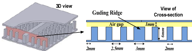
Fig.1 (a) Detailed dimensions of the periodic metal pin and ridge gap waveguide geometry used in this paper.
