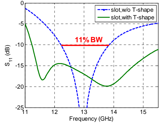
Fig.2 (b) Simulated S_{11} for the slot element with and without the T-shape in the feeding ridge section.
