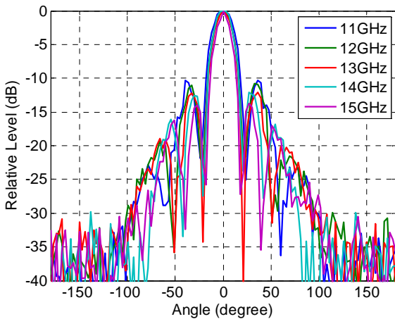
Fig.16 (a) Measured H plane radiation patterns for the linear array.
