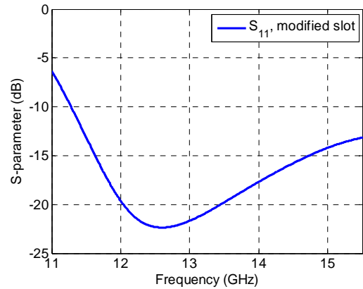
Fig. 7 (b) Simulated reflection coefficient for the modified slot element.
