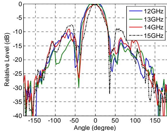
Fig.17 (b) Measured E plane radiation patterns for the planar array.
