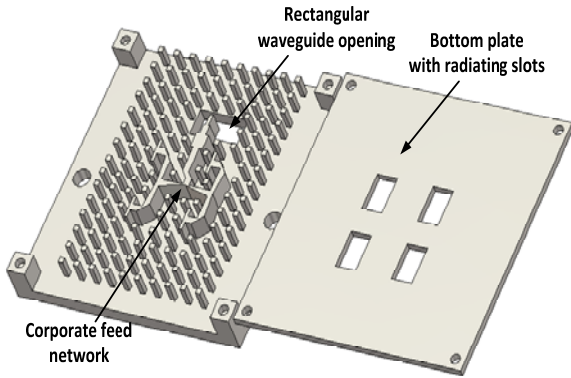
Fig.10 (a) Complete 2 \times 2 element array geometry; element spacing is 17.5mm.
