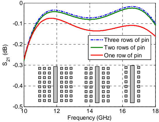
Fig. 1(d) Simulated S_{21} for different rows of pins around the guiding ridge.
