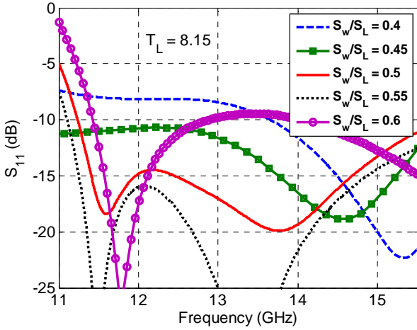
Fig.2 (d) Variation in parameter S_w/S_L of the slot element, T_L is kept 8.15mm.
