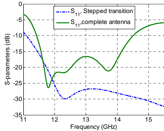
Fig.5 (b) Simulated S_{11} for the stepped transition from ridge gap waveguide to groove gap waveguide and the complete linear array antenna.
