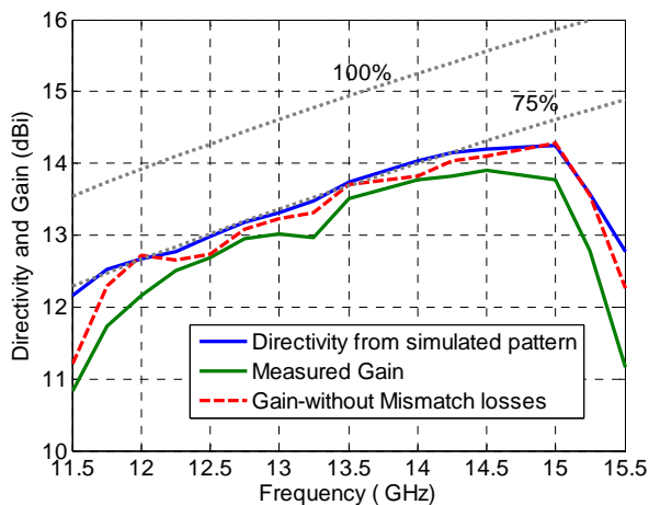
Fig.18 Simulated directivity and measured gain for the planar array.
