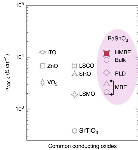
Figure 6 | Comparison of conductivity values for common conducting oxides. Compilation of highest room temperature conductivity \sigma_{300K} of \text{BaSnO}_3 bulk single crystal and films grown by various deposition techniques (taken from refs 9,16,22) including hybrid molecular beam epitaxy. The highest known \sigma_{300K} for common transparent conducting oxides (ITO = indium tin oxide, ZnO) and other metallic oxides as conductive electrodes for high frequency applications ( \text{VO}_2 , \text{LSCO} = \text{La}_{0.5}\text{Sr}_{0.5}\text{CoO}_3 , \text{SrTiO}_3 , \text{LSMO} = \text{La}_{0.7}\text{Sr}_{0.3}\text{MnO}_3 , \text{SRO} = \text{SrRuO}_3 ) are shown for comparison (refs 49–55).
