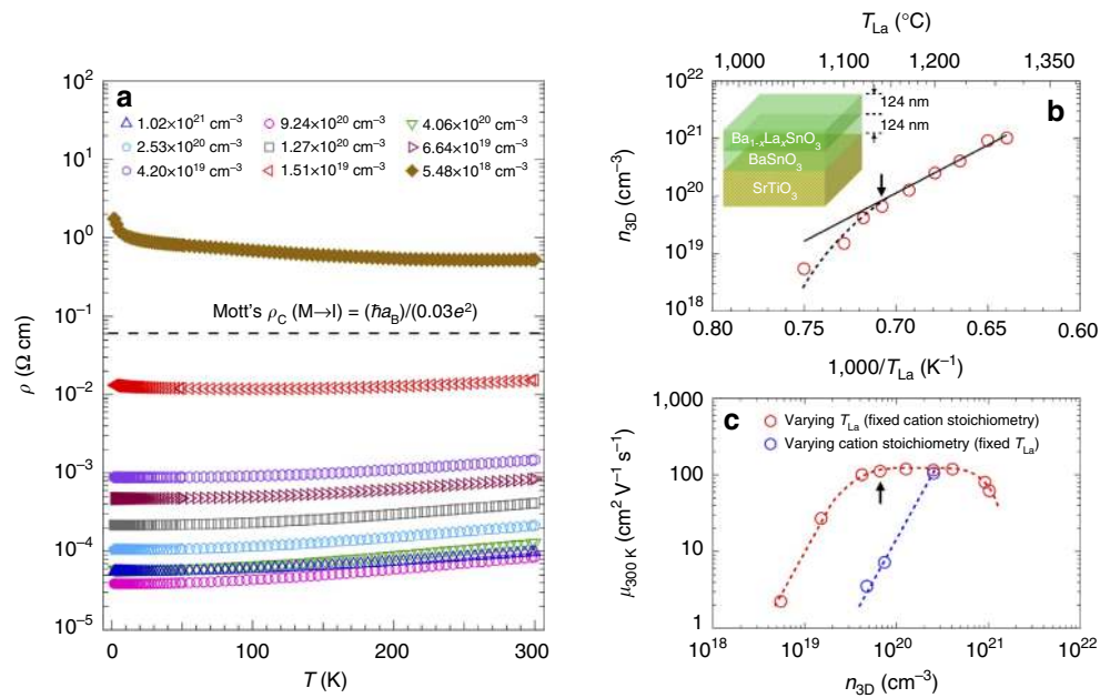
Figure 2 | Temperature dependence of resistivity and the influence of charge compensation on room temperature carrier density and mobility. (a) Resistivity ( \rho ) of doped \text{BaSnO}_3 films as a function of temperature ( T ) for different free carrier concentration measured at 300 K. (b) Free carrier concentration ( n_{3D} ) at 300 K as a function of La cell temperature ( T_{La} ) representing dopant concentration. Inset shows the schematic of the structure used, and (c) \mu_{300\text{K}} versus n_{3D} for stoichiometric (red open circles) and Ba-deficient films (blue open circles). Non-stoichiometric films had 31 nm of buffer and active layer thicknesses. Black arrows mark the onset of charge compensation.
