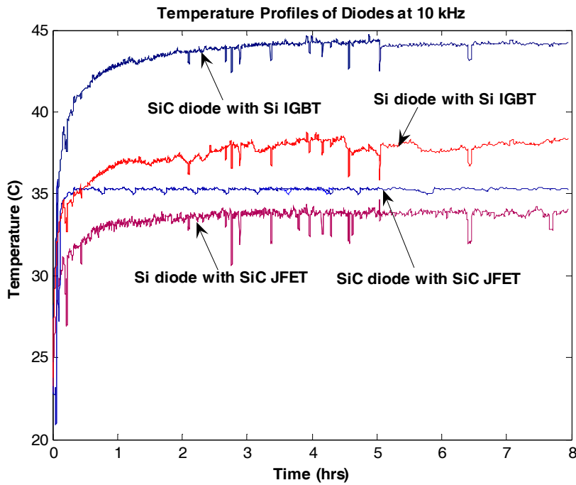
(b) Diodes.
