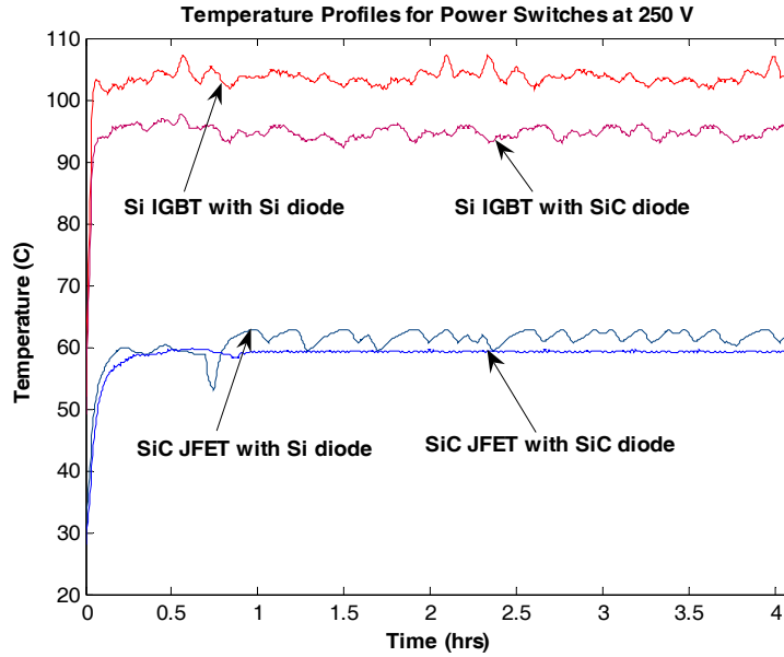
Fig. 5.6. Temperature profile for power switches at 250-V, 10-kHz operation.
