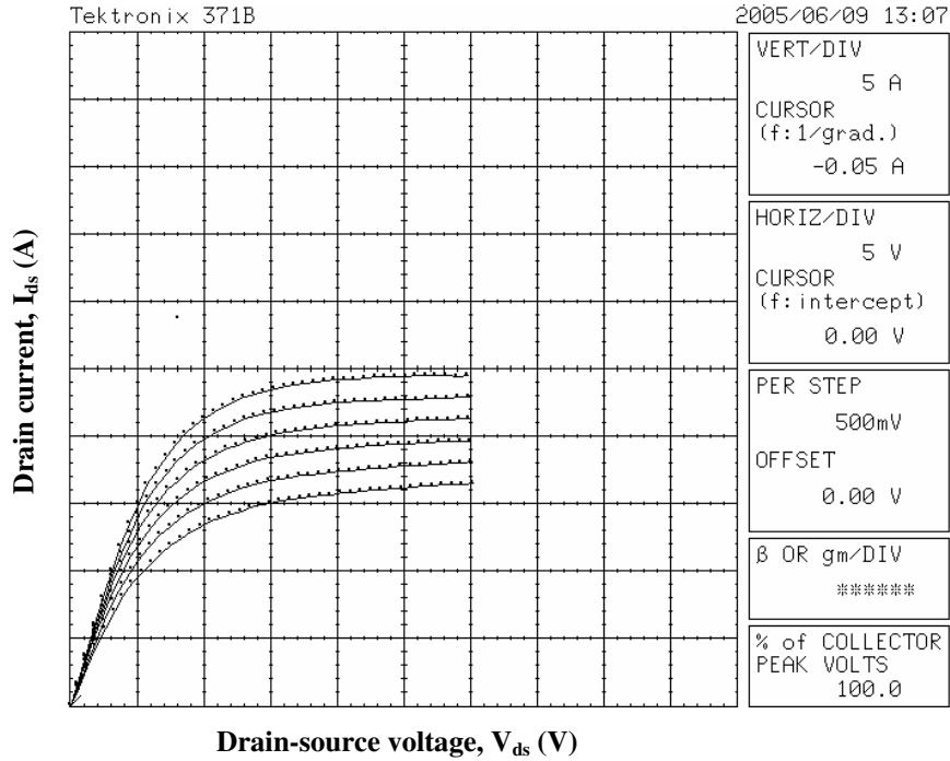
Fig. 4.2. Unipolar operation of the Rockwell SiC JFET.
