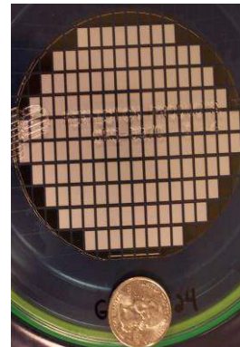
Fig. 3.14. 75-A Schottky diodes developed by Cree.
