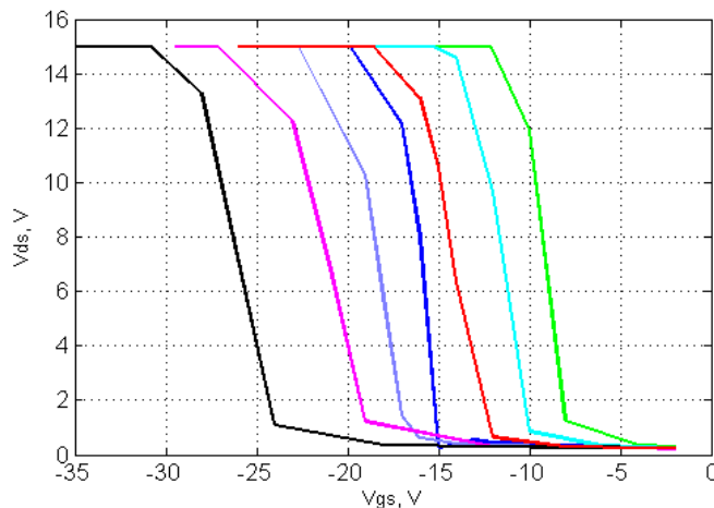
Fig. 2.16. Transfer characteristics of several SiC JFET samples.
