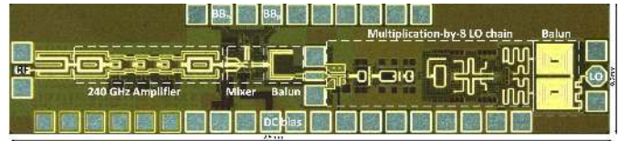
Fig. 5. Transmitter die photo for on-wafer characterization.
