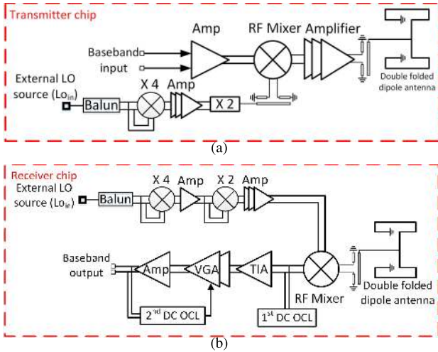
Fig. 1. (a) Transmitter and (b) receiver block diagrams.
