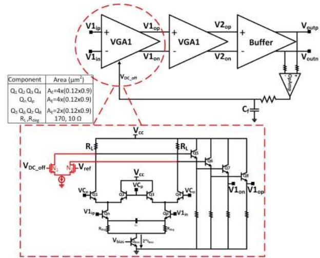
Fig. 11. Schematic of cascaded VGAs and output buffer with second dc OCL.
