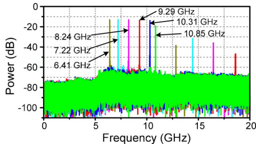
Fig. 5. (Color online) Spectra of the generated electrical signal with the frequency tuned from 6.41 to 10.85 GHz; RBW = 1 MHz.
