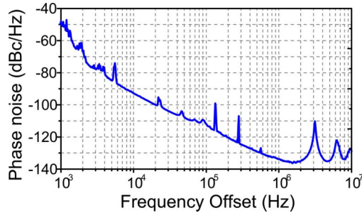
Fig. 4. (Color online) Phase noise measurement for the generated 10 GHz microwave signal.
