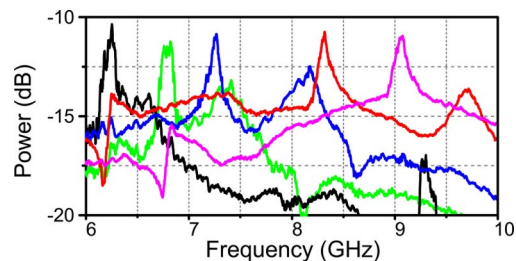
Fig. 2. (Color online) Frequency responses of the FP-LD-based photonic microwave filter.
