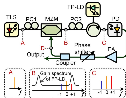
Fig. 1. (Color online) Schematic of the proposed frequency-tunable optoelectronic oscillator.
