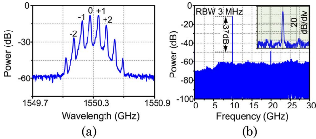
Fig. 3. (Color online) Generation of 10 GHz signal using the proposed OEO. (a) Optical spectrum. (b) Electrical spectrum. Inset, span = 10 MHz, and resolution bandwidth (RBW) = 91 kHz.
