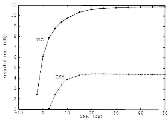
Fig. 2. Resolution comparison between the two algorithms (TCT and CSM).
