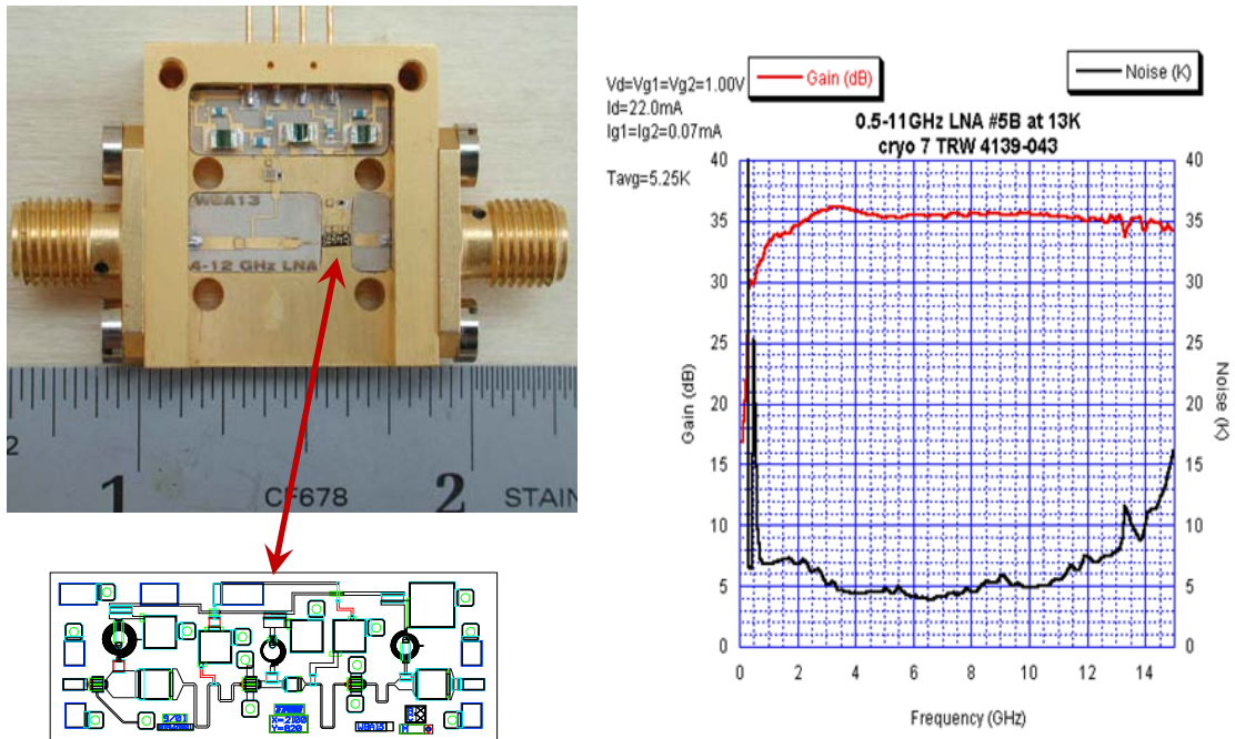
Figure 2 - InP HEMT 3-stage amplifier chip, 2mm wide, is bonded into the coaxial chassis shown at upper left to produce ~5K noise and 35dB gain at 13K from 1 to 12 GHz shown at right.
