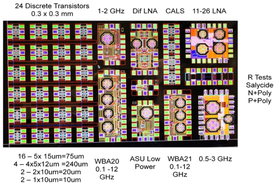
Figure 3 - Wafer segment of 24 discrete transistors, 7 MMIC LNA's, and calibration structure fabricated at ST Microelectronics and under test at Caltech.
