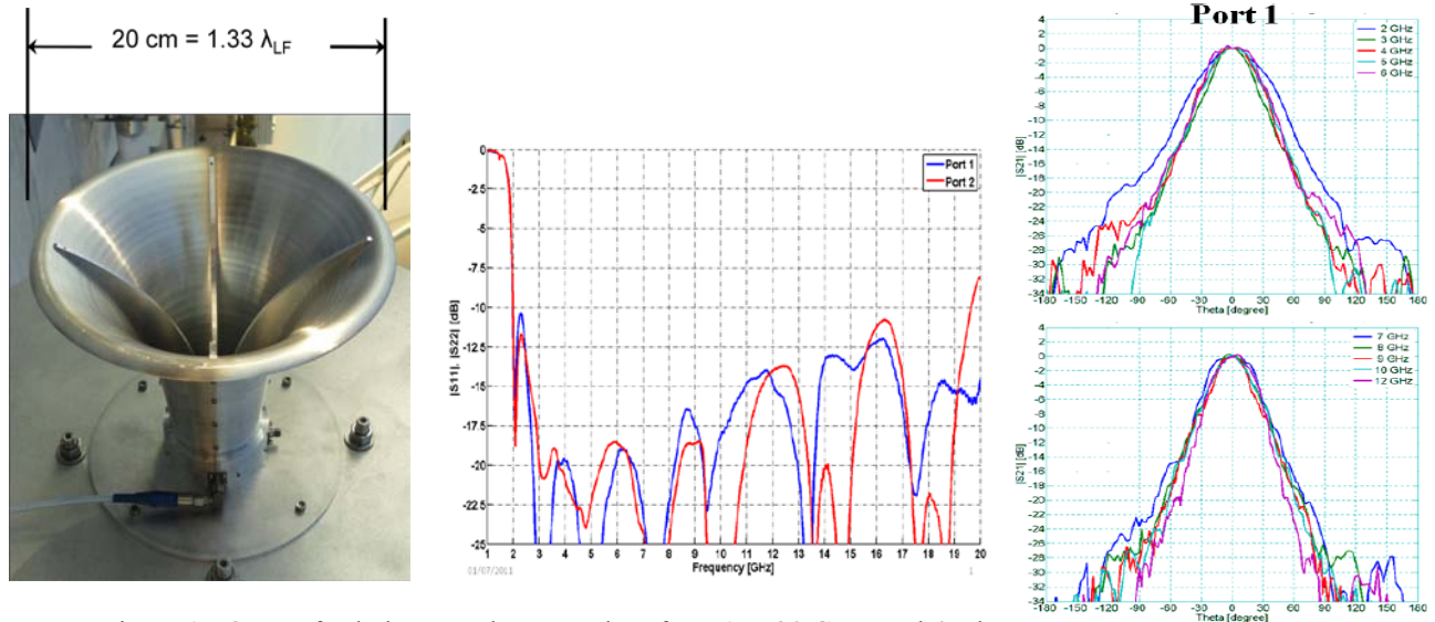
Figure 1 - QRFH feed photograph, return loss from 1 to 20 GHz, and 45 degree patterns, 2-12 GHz.
