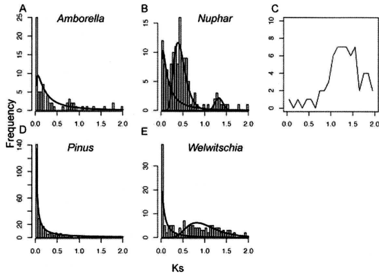
Figure 5. K_s distributions suggest possible genome duplications in basal angiosperms, and no evidence for genome duplication events in Amborella and some gymnosperm species. (A) K_s distribution in Amborella , a basal-most angiosperm. No significant large-scale duplication is detected. (B) Three distinct components in the K_s distribution for Nuphar , also a basal-most angiosperm, suggest at least two large-scale genome duplications. (C) K_s distribution for putative orthologs between Amborella and Nuphar . (D) Pinus taeda (loblolly pine) paralogous pairs follow the null model (see Methods). (E) K_s distribution for paralogs in a gymnosperm, Welwitschia .
