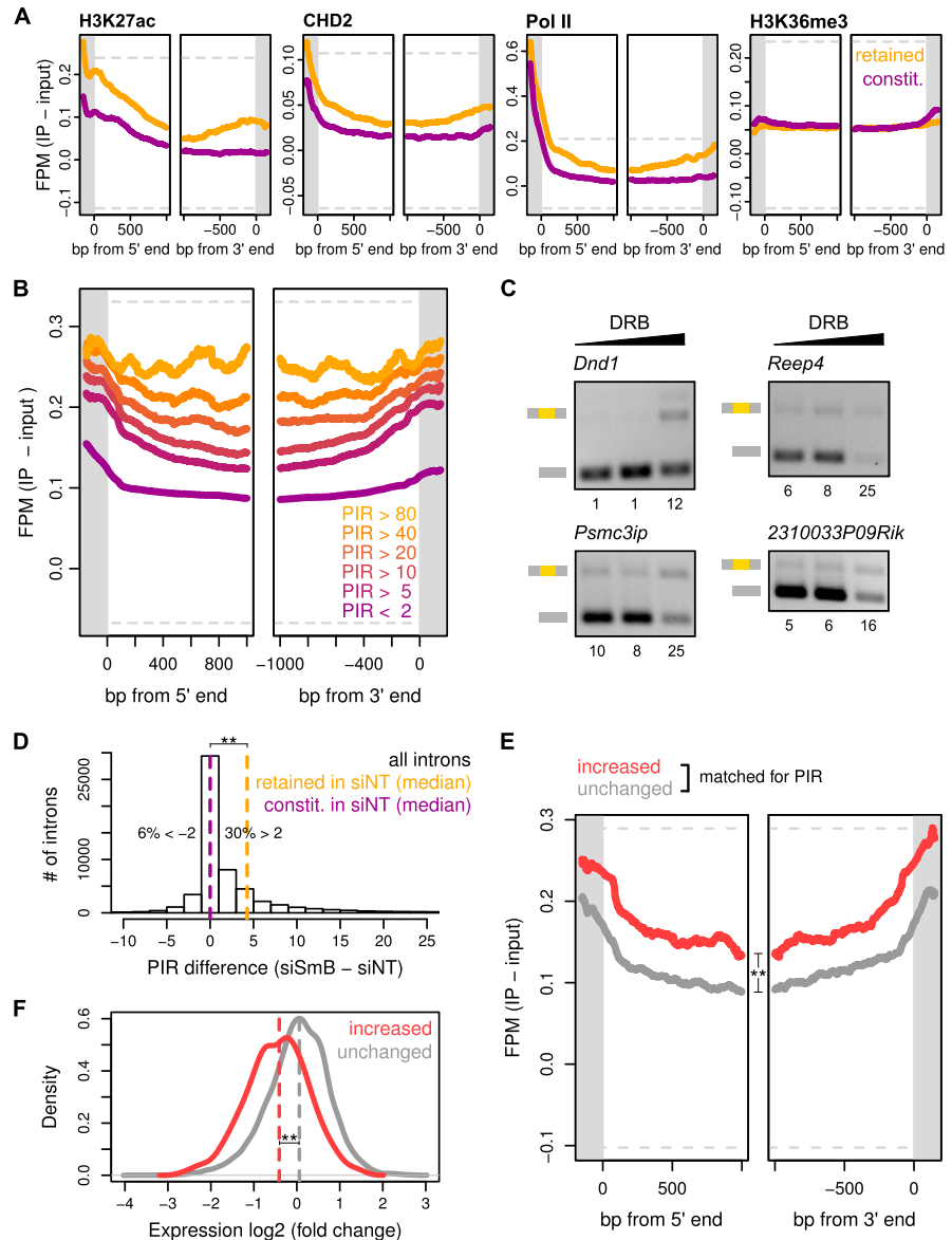
Figure 6. Coupling between IR and RNA Pol II elongation. (A) Average ChIP-seq signals across introns that are retained (orange, PIR \geq 10 ) or not retained (purple, PIR < 2 ) in K562 cells, for four of 129 analyzed human chromatin features. Retained and not retained introns analyzed are in genes with matched expression levels. (Gray bars) Flanking exons; (y-axes) input-subtracted average ChIP fragment density per million reads (FPM-input) at each aligned bp; (gray dashed lines) 2nd and 98th percentiles of all values in the plot region before averaging to give an indication of the dynamic range. See Supplemental Figure S9A for similar analysis in mouse CH12 cells. (B) Average ChIP-seq signal of Ser2-phosphorylated RNA Pol II over introns with different PIR thresholds in K562 cells. Labels and plots as in A. See Supplemental Figure S9B for similar analysis in mouse CH12 cells. (C) RT-PCR assays of IR events in CGR8 mouse ES cells with and without treatment with the RNA Pol II elongation inhibitor DRB. Retained introns with low PIR in ES cells relative to other cell types were analyzed. (Lane 1) 0 \mu\text{g}/\text{mL} DRB; (lane 2) 10 \mu\text{g}/\text{mL} ; (lane 3) 25 \mu\text{g}/\text{mL} . Quantifications are shown beneath each panel. See Supplemental Figure S10 for the full set of tested introns. (D) Number of introns with PIR changes in HeLa cells transfected with siRNAs targeting SNRNPB , which codes for SmB/B', relative to cells transfected with a control, nontargeting siRNA (Saltzman et al. 2011). (Dashed lines) Medians of retained ( PIR \geq 10 ) and constitutive ( PIR < 2 ) introns in control treated cells; (asterisks) P < 0.001 between these groups (one-sided Mann-Whitney U test). (E) RNA Pol II occupancy over introns (in untreated HeLa cells) that become more retained (PIR difference > 15 , red) or that do not change (PIR difference between -2 and +2 , gray) after SNRNPB knockdown. Because RNA Pol II occupancy is dependent on absolute PIR, groups of introns with matching PIR distributions in control treated cells and > 2 kb away from the transcription start site are shown. (Asterisks) P < 0.001 for difference in median Pol II-Ser2p occupancy (see Methods for test details). (F) Expression change between SNRNPB and control knockdown for genes containing introns that become more retained (PIR difference > 15 , red) or that do not change (PIR difference between -2 and +2 , gray). (Asterisks) P < 0.001 between these groups (one-sided Mann-Whitney U test).
