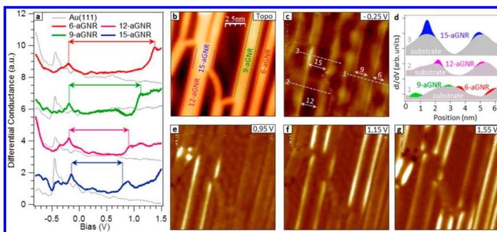
Figure 2. (a) Spectra recorded on 6-aGNR (red), 9-aGNR (green), 12-aGNR (pink), and 15-aGNR (blue), where the Au(111) signal (black) is added to every spectrum as background reference (open-feedback parameters: V_s = 1.55 V, I_t = 1.4 – 10 nA; modulation voltage V_{rms} = 10 mV). (b) STM topography image ( 12.4 nm \times 12.4 nm; V_s = -1.1 V; I_t = 0.61 nA). (c) Conductance map near the valence band onset ( V_s = -0.25 V), with white arrows as a guide for the eye to the intensity along each aGNR edge. (d) Profiles across the conductance map in (c), highlighting the contribution from the VB of differently wide GNRs on top of the dominating Au(111) surface state contribution. Conductance maps near the conduction band onsets for (e) 15-aGNRs and 12-aGNRs ( V_s = 0.95 V), (f) 9-aGNR ( V_s = 1.15 V), and (g) 6-aGNR ( V_s = 1.55 V). The displayed spectra have been taken from ribbons on different sample locations (not necessarily on those of panels b–g). Differences in the reference spectra relate to different tips and positions. The comparable intensity in 12- and 15-aGNRs' edges in image (d) probably relates to the limited length of the 15-aGNR segment. Its reduced length causes an increased band gap and thus leads to an upshift in the energy of the conduction band onset, making it overlap with that of the longer 12-aGNR. Size and set point for all conductance images were 12.4 nm \times 12.4 nm and I_t = 0.61 nA, respectively.
