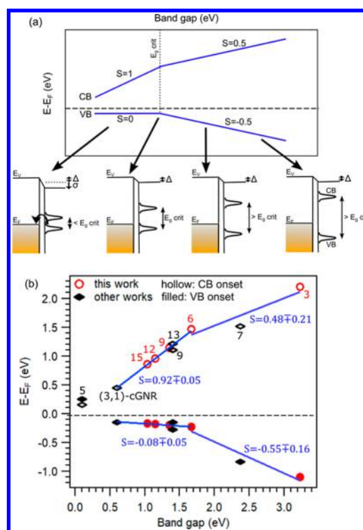
Figure 5. (a) Schematic evolution of the energy level alignment of valence and conduction band for varying adsorbate band gap. The energy level diagrams depict the interface dipole \Delta from the molecular adsorption, as well as the additional dipole \sigma responsible for Fermi level pinning as the band gap gets narrower and one of the bands approaches the Fermi level (the valence band in this figure). It also displays the changing slopes of valence and conduction band onset vs band gap as Fermi level pinning sets in. (b) Valence and conduction band onsets of GNRs studied in this work and in other reports of Au(111)-supported ribbons vs their respective band gap (width given by numbers next to the CB symbols). Linear fits in selected regions display the changes in slope, evidencing notable similarity with the model scenario of panel (a).
