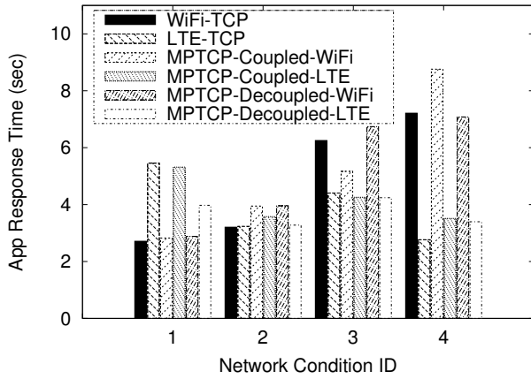
Figure 18: CNN app-response time under different network conditions.
