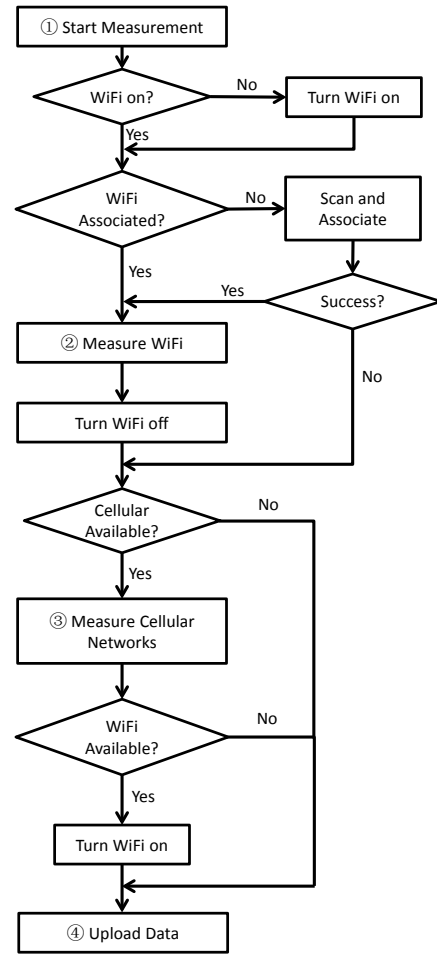
Figure 2: Cell vs WiFi: single measurement collection run.
