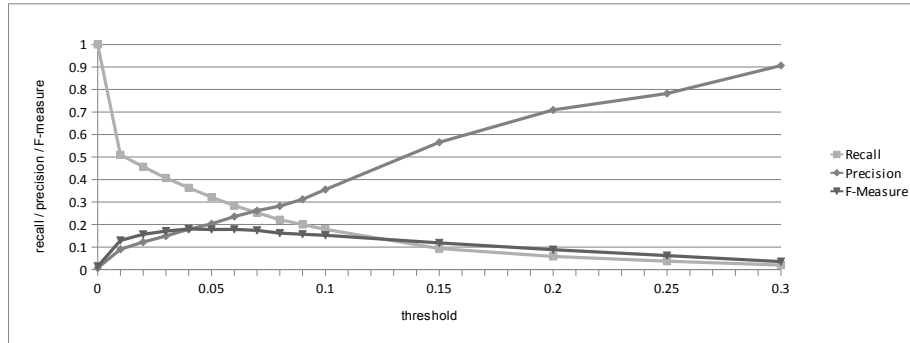
Fig. 6. Average F-measure, precision and recall for OEAI multifarm track with Individual Token Search Approach .
