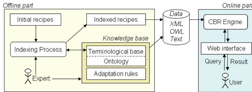
Fig. 3. Architecture of the TAAABLE system.
