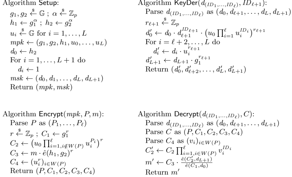
Fig. 5. The Boneh-Boyen-Goh WIBE scheme.
