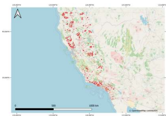
Fig. 2: Perimeters of fires in CAL FIRE between 01.01.2017 and 31.12.2019. Fire perimeters are delineated in red.
