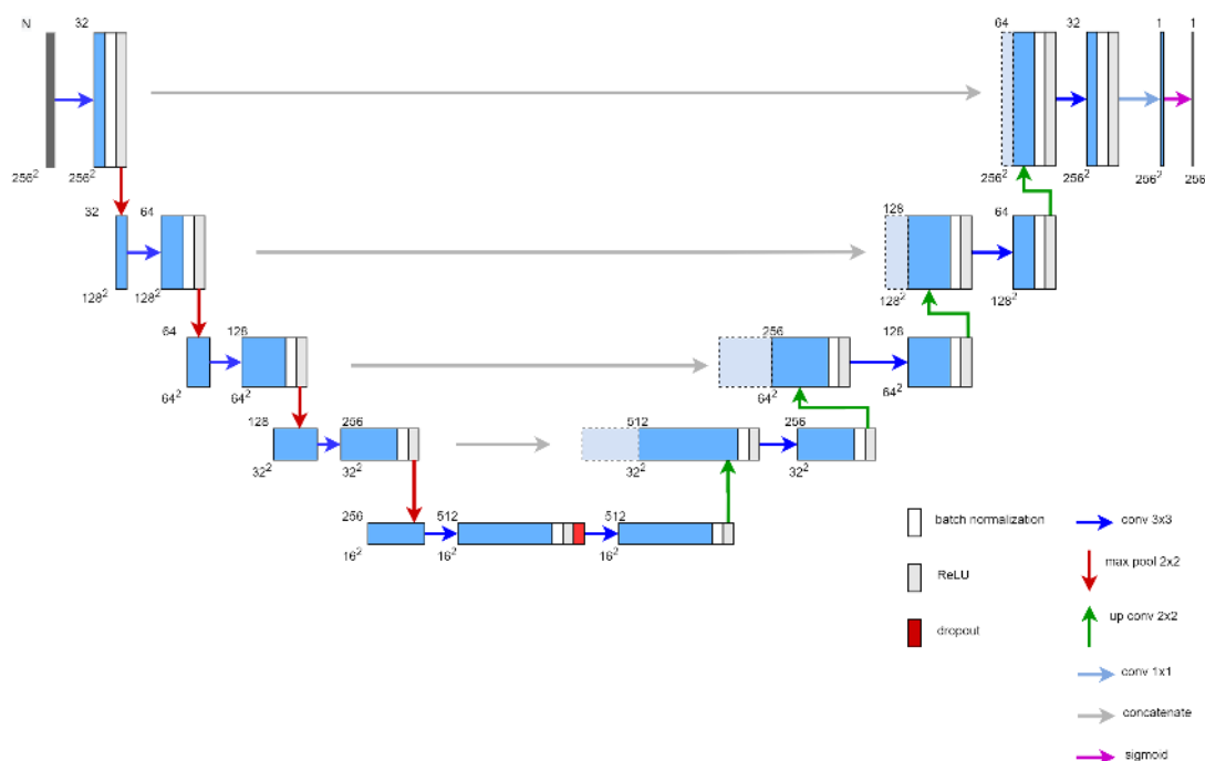
Fig. 5: Modified U-Net architecture used in this work. Each blue box corresponds to a multi-channel feature layer. Dark gray box represents the input image with N channels (2 for Sentinel-1, 3 for all other instruments). The number of channels is denoted on top of the box. The spatial dimensions of the feature are provided at the lower left edge of the box. Pale blue boxes represent copied feature information. The arrows denote the convolution, pooling and concatenating operations. The final output is a probability raster with values between 0.0 and 1.0 (Modified from [34]).
