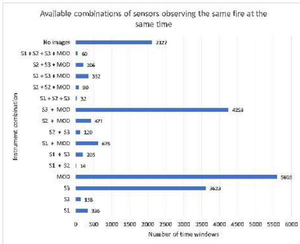
Fig. 4: Number of time windows with different combinations of instruments observing the same fire. The duration of every fire is split into twelve-hour-long time windows. The chart shows the number of time windows that were observed by different combinations of instruments. The horizontal axis represents the number of time windows and the vertical axis represents the possible combinations of instruments.
