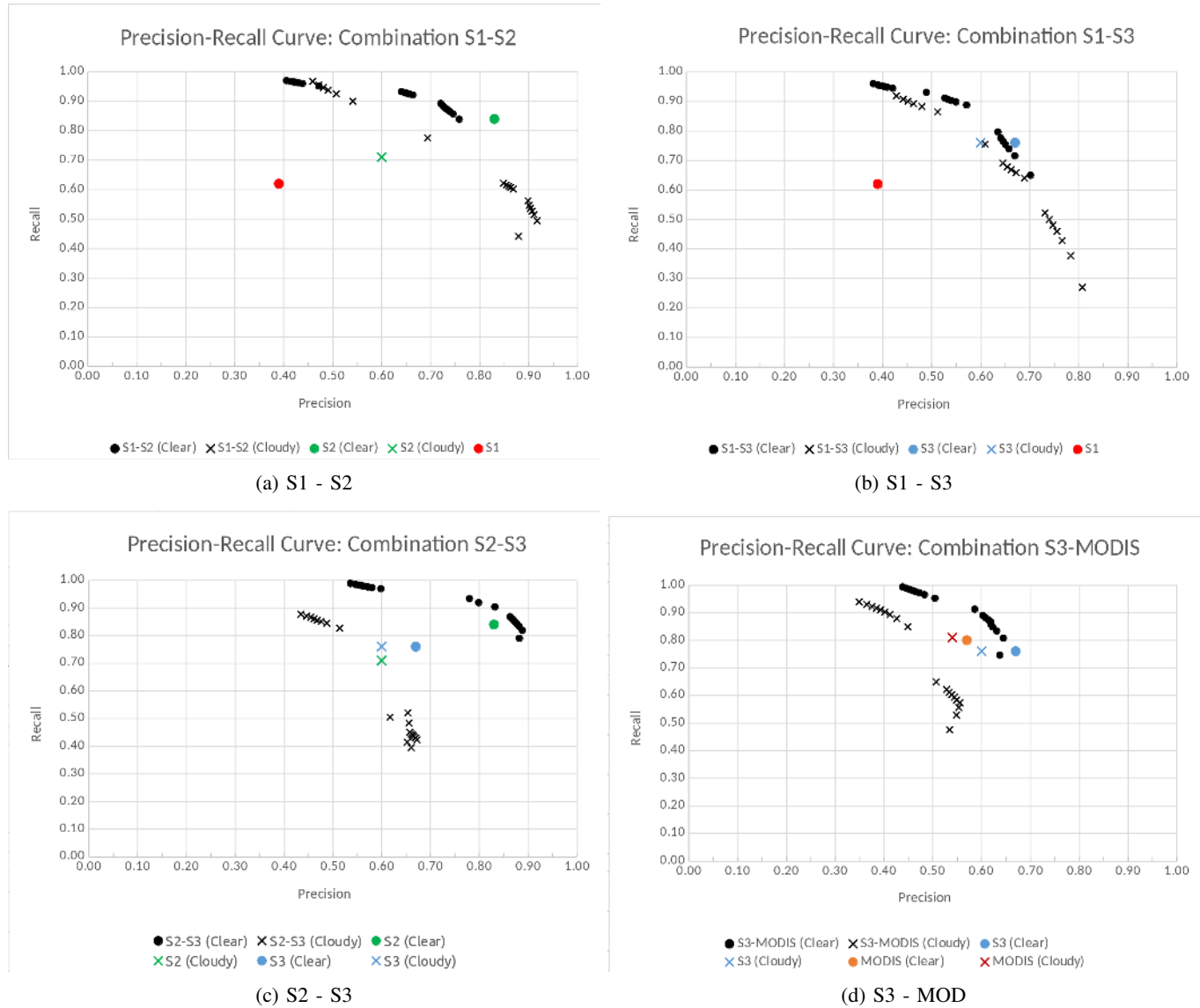
Fig. 8: Precision-Recall curves of bi-instrument segmentation results. Best precision-recall results obtained with single instrument models are plotted in comparison.
