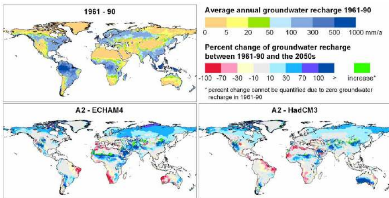
Fig. 3 Impact of climate change on long-term average annual diffuse groundwater recharge. Percent changes of average groundwater recharge between 30-year intervals, 1961–1990 and the 2050s (understood as a 30-year standard normal, centred on 2050s, i.e. 2041–2070), as computed by WGHM applying two different climate change scenarios (climate models ECHAM4 and HadCM3, each fed by IPCC greenhouse gas emissions scenario SRES A2, cf. Nakićenović & Swart (2000)). Modified after Döll & Flörke (2005).
