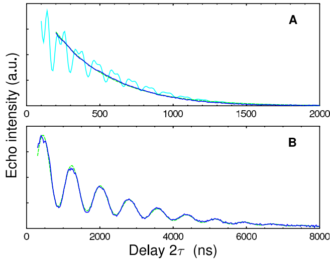
FIG. 2 (color online). (a) Decay of the Hahn-echo intensity in \text{Cr}_7\text{Ni} as a function of delay time for long, selective pulses (64 ns \pi/2 pulse, 128 ns \pi pulse, blue) and for short broadband pulses (16 ns \pi/2 pulse, 32 ns \pi pulse, cyan). (b) Decay of the Hahn-echo intensity for long, selective pulses in perdeuterated \text{Cr}_7\text{Ni} . Dashed green lines indicate fits to the data. The fit in (b) assumes that the ESEEM effect is dominated by a single harmonic at the ^2\text{D} Zeeman frequency [31]. (Note the different horizontal axis scales.)
