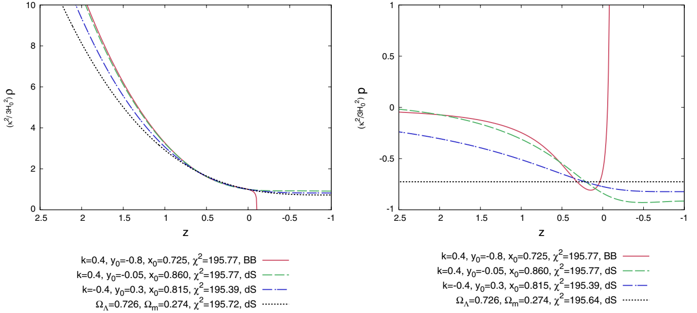
FIG. 2 (color online). The evolution in the recent past of the Universe and in the future of the normalized energy density \frac{\rho}{\rho_{\text{cr},0}} (left panel) and of the normalized pressure \frac{p}{\rho_{\text{cr},0}} (right panel) is shown for four models. One of the models leads to a Big Brake singularity in the future while the other three models shown tend asymptotically to a de Sitter space.
