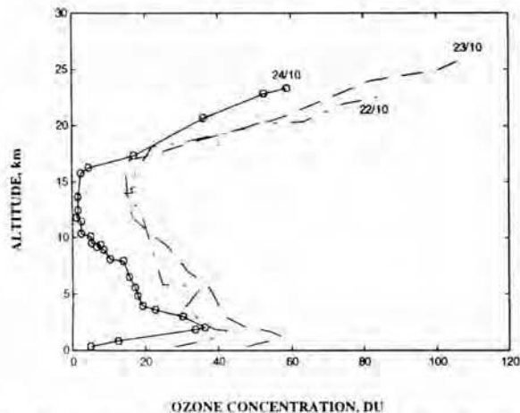
Fig. 3—Comparison of vertical ozone distribution during solar eclipse (circle) of 24 Oct. 1995 with control day profile at Ramgarh (23°38'N)
