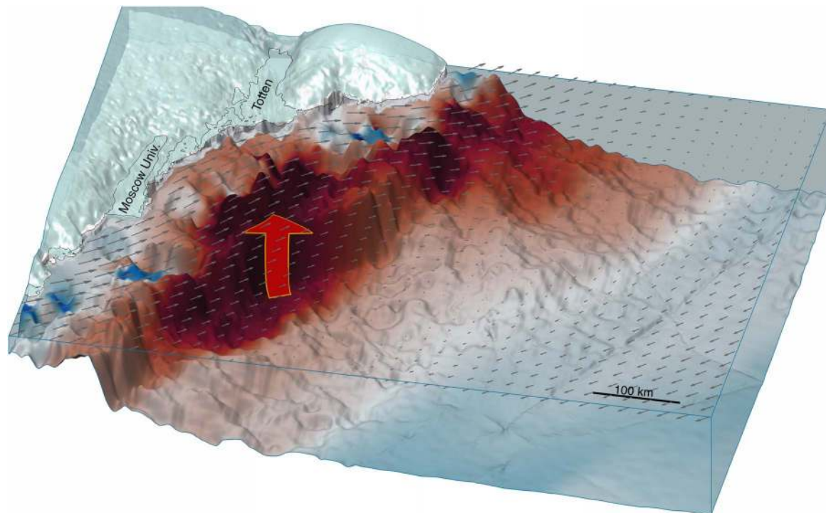
Fig. 4. Schematic of mCDW upwelling along the Antarctica's Sabrina Coast. Around Antarctica, the warmest waters are found in the deep ocean north of the continental shelf break. Where wind stress (gray vectors) causes surface waters to part, warm deep water (red arrow) can upwell, surmount the continental shelf, and melt nearby ice shelves from below. Seafloor color depicts the covariance of TIS velocity and local upwelling as in Fig. 3D, indicating where wind driven upwelling is closely linked to TIS velocity.
