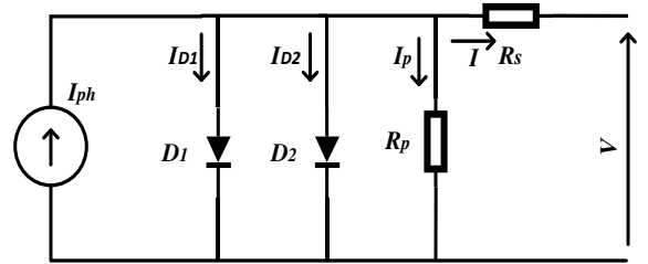
Fig. 1. Double – diode solar PV equivalent circuit.
