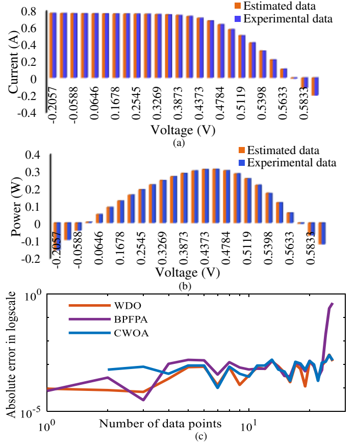
Fig. 4 (a) RTC France solar cell (a) I-V Characteristics, (b) P-V characteristics (c) Absolute error of three optimization techniques.
