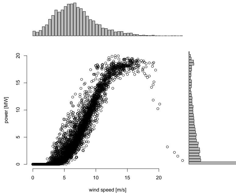
FIG 2. Example empirical power curve for the Klim wind farm over a 6-month period in 2002, based on hourly measurements of wind speed and corresponding power output. Marginal distributions of wind speed and power are also represented above, and respectively right of, the power curve itself.
