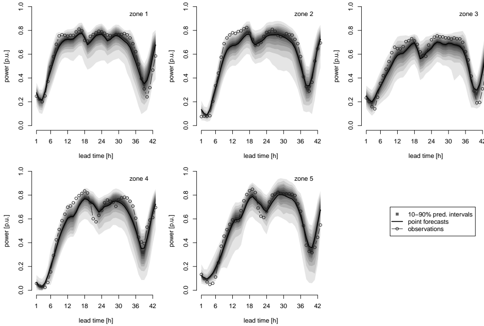
FIG 6. Example episode with probabilistic forecasts for the 5 aggregated zones of Western Denmark (and corresponding measurements obtained a posteriori), as issued on 16 March 2007 at 06 UTC. They take the form of so-called river-of-blood fan charts (termed coined after Wallis, K. F. (2003)), represented by a set of central prediction intervals with increasing nominal coverage rates (from 10% to 90%).
