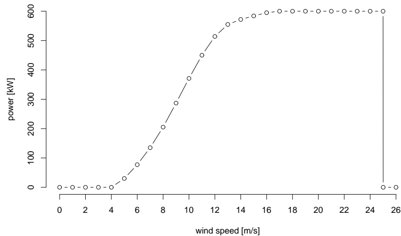
FIG 1. Power curve of the Vestas V44 (600kW) wind turbines installed at the Klim wind farm, for an air density of 1.225 \text{ kg/m}^3 .
