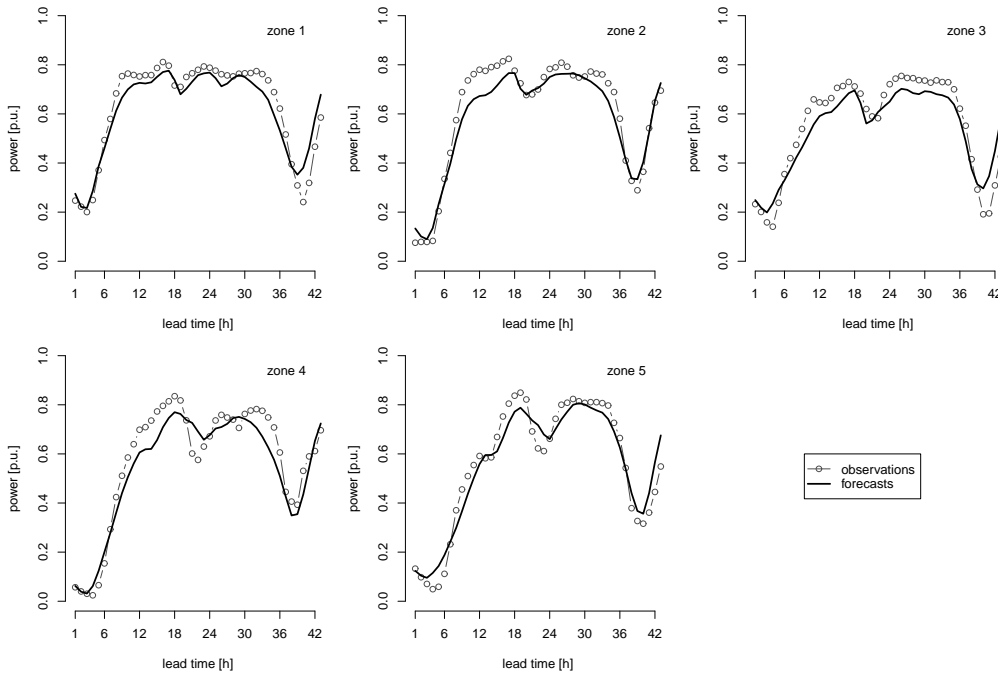
FIG 5. Example episode with point forecasts for the 5 aggregated zones of Western Denmark, as issued on 16 March 2007 at 06 UTC. Corresponding power measurements, obtained a posteriori, are also shown.
