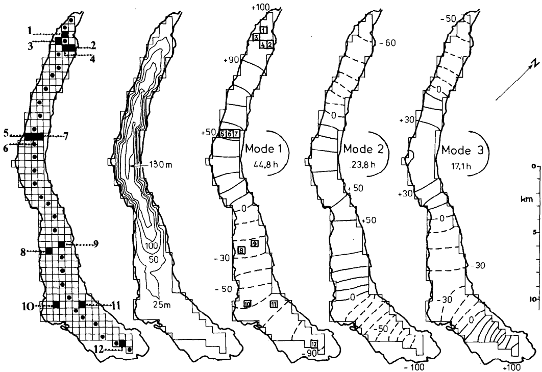
Fig. 4. Predictions by the TVDM of interface elevation distributions, associated with the first three internal modes, relative to a maximum elevation of 100 in each case and with upper- and lower-layer temperatures and interface depth as defined in Fig. 1, top right. The model grid (based on a design by Oman 1982) and the corresponding model depth contours are shown at the left. ■—Mooring positions 1–12; ●—grid-points taken to represent the Talweg for comparisons with the Defant model.
