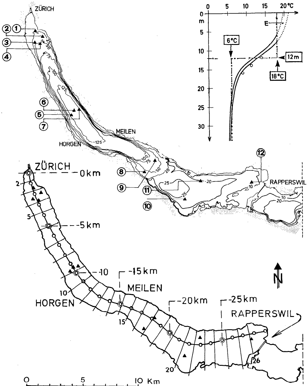
Fig. 1. Bathymetric chart of Lake Zurich; ▲—1978 positions of current meter and thermistor-chain moorings (1–12, Table 1). Depth contours are in meters, relative to a mean surface level of 406 m ASL; the lower chart displays the cross-sections (2–26) used in the Defant calculation and the Talweg (defined in the text) marked at kilometer intervals (O). Temperature/depth profiles at eleven of the moorings, averaged over the interval 6 August–28 September 1978, fall within the double-line envelope illustrated at the top right (from W. Horn's data report, see Fig. 2 legend). Mooring 4 values are shown circled; extrapolation E above 6 m is shown dotted. The two-layered approximation to the whole-basin average profile is displayed by dash-dot lines.
