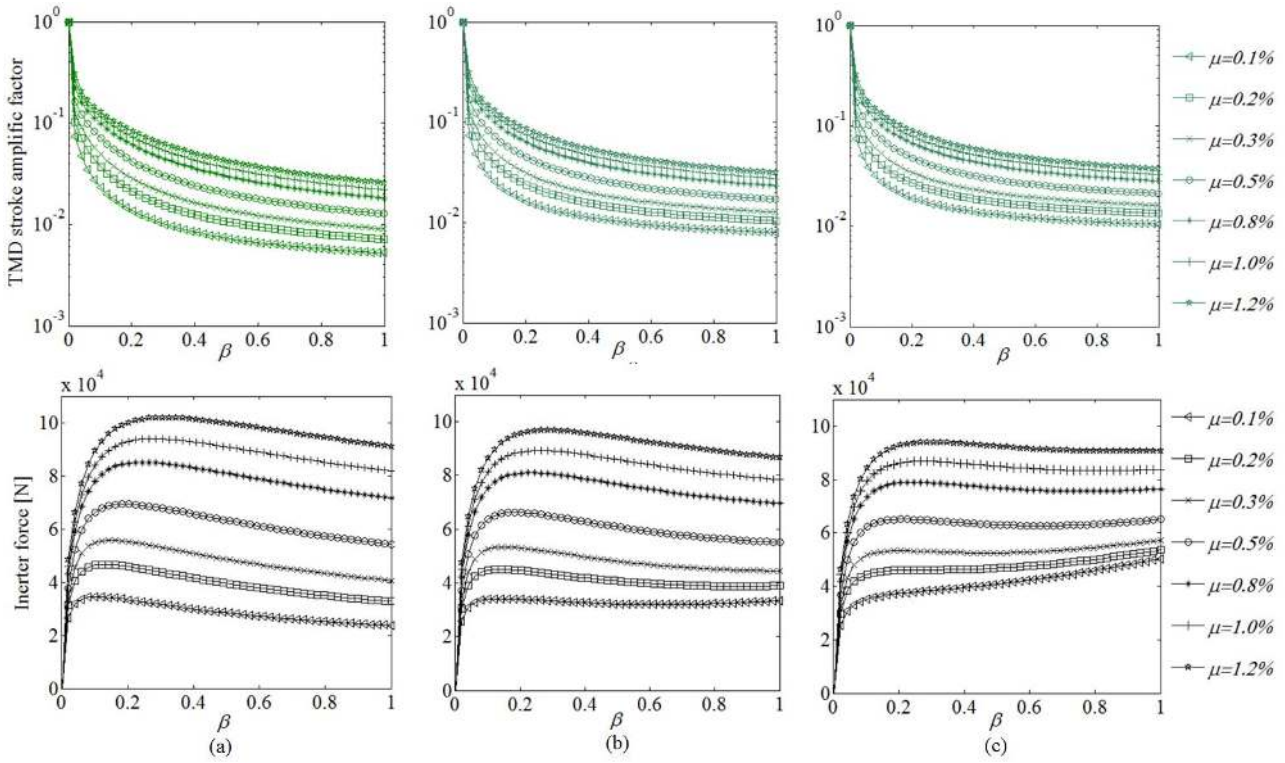
Fig. 5. Peak TMDI attached mass displacement over peak TMD attached mass displacement (upper panels), and peak inverter resisting force (lower panels) for different values of inertia ratio \beta and attached mass ratio \mu for TMDI topologies (a) “-1”, (b) “-2”, and (c) “-3”.
