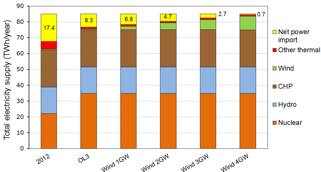
Figure 6. Evolution of power supply mix in Finland from 2012 to the commissioning of Olkiluoto 3 (OL3), and further in wind integrations up to 4000 MW (power demand 85 TWh/a)—The amount of net power imports are labeled on each bar.
