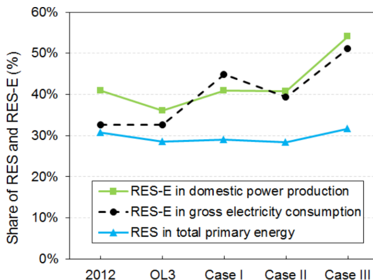
Figure 9. Share of RES and RES-E in different Cases compared to 2012, based on the assumptions in Table 3 (OL3: Olkiluoto 3).
