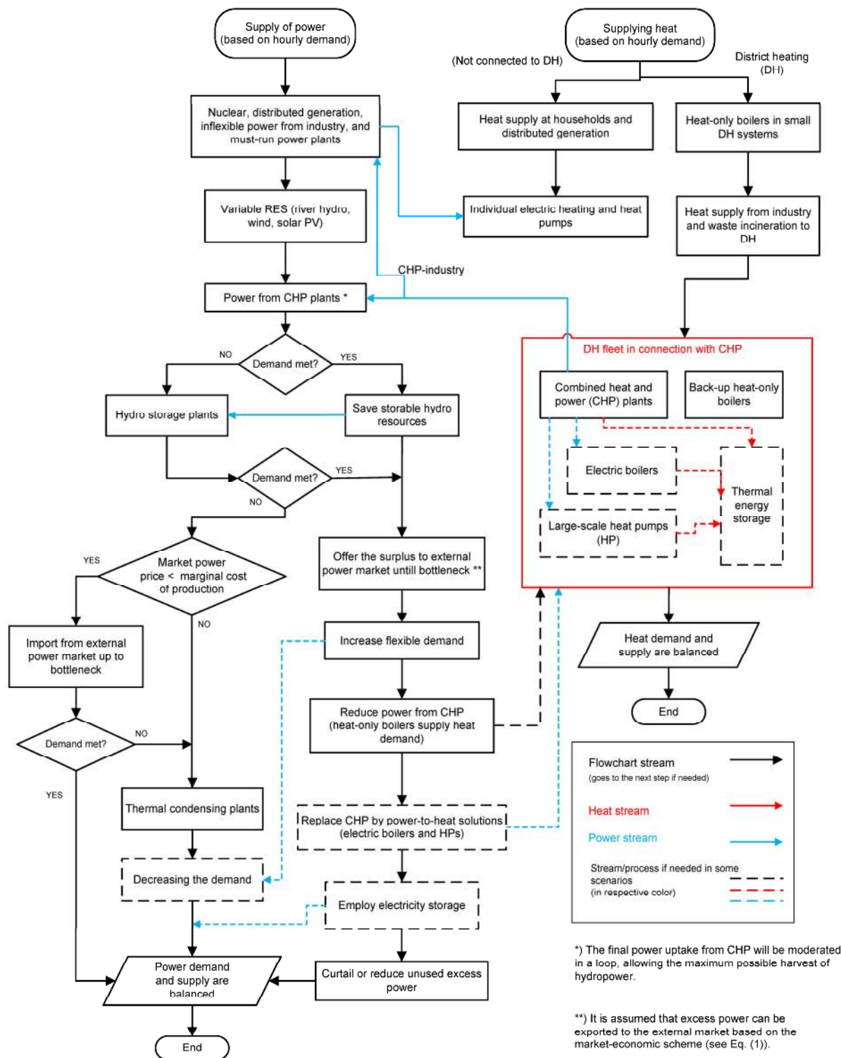
Figure 1. Schematic scheme of the model in supplying power and heat in an integrated method based on hourly distributions of demand and market prices of electricity—This procedure is translated into a set of regulation strategies to be run by EnergyPLAN.
