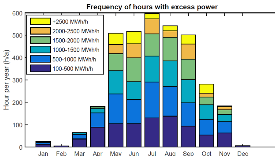
Figure 13. The frequency and magnitude of excess power in different months of the year (conditions for Case I, see Table 3).
