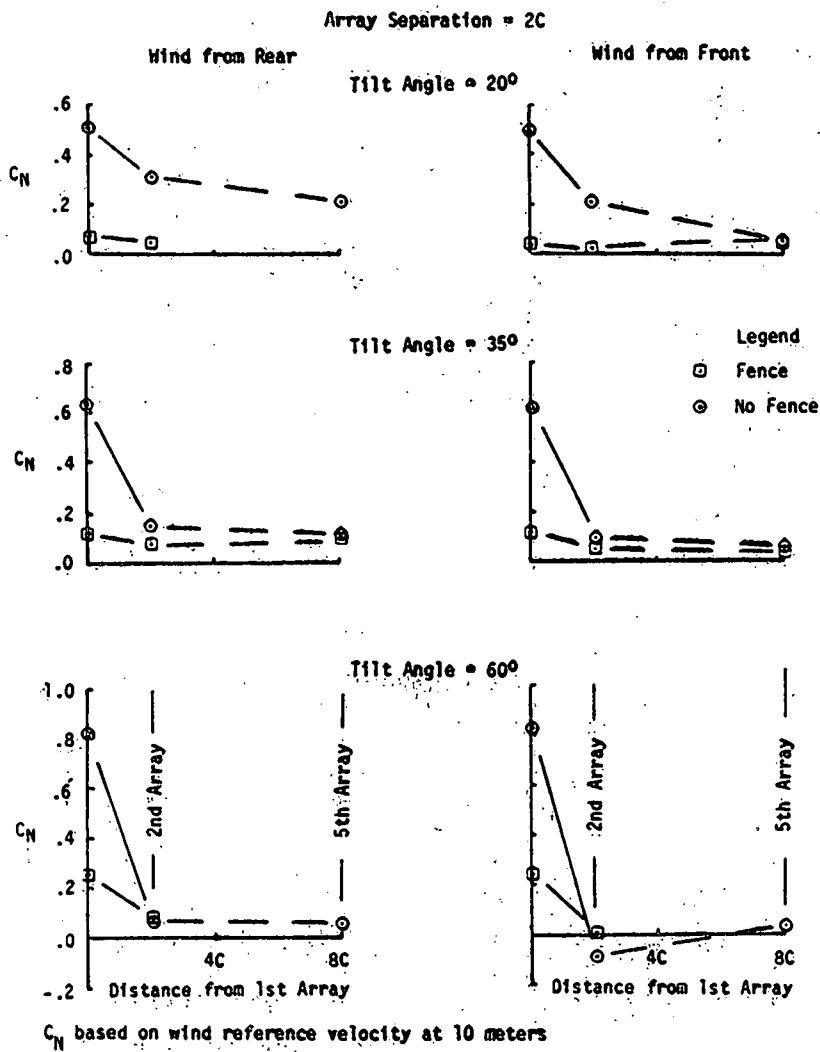
Figure 4-6. Effect of a Fence on Array Normal Force Coefficients for Head-On and Rearward Winds.
