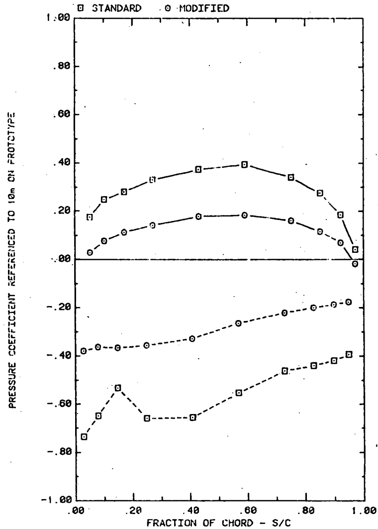
FRONT AND BACK PRESSURES ON ARRAY #1 WITH X=2C , AND WIND=45 EFFECT OF TAP LOCATION; ALPHA=145, H=3°, D=10°, FC=1, AND P=30%
