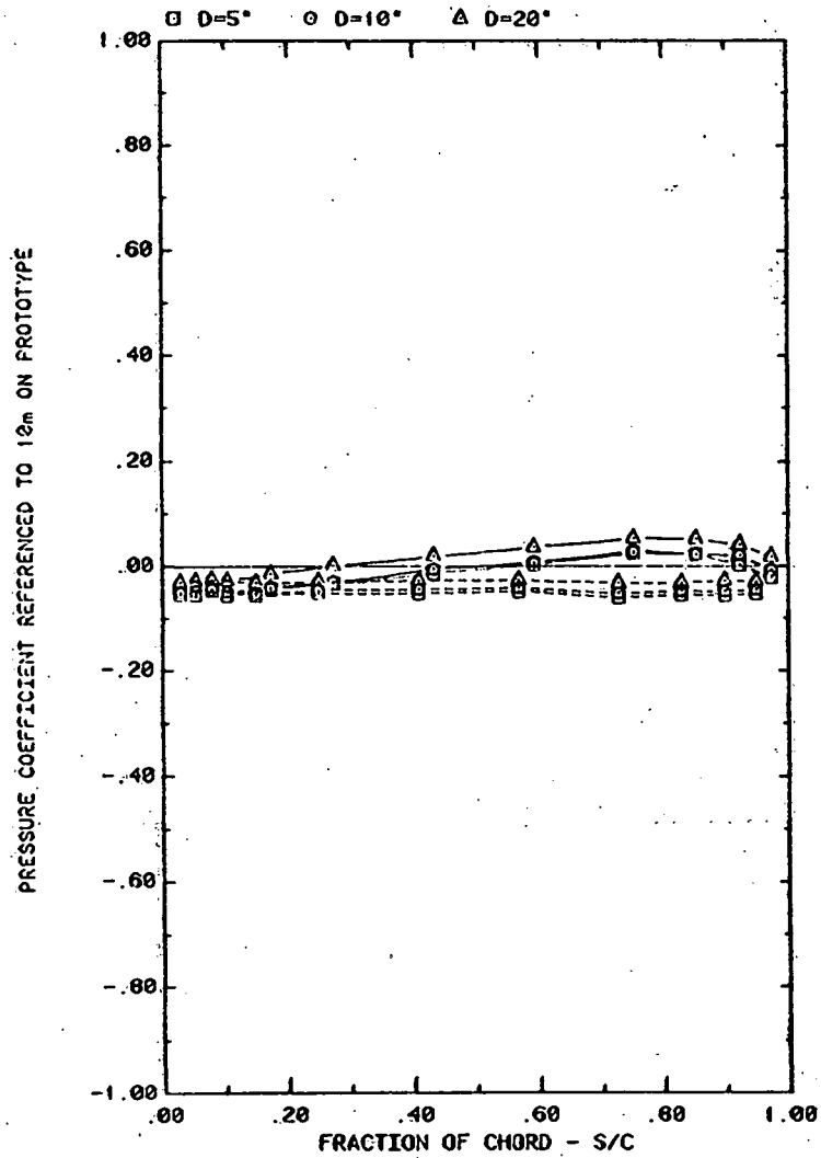
FRONT AND BACK PRESSURES ON ARRAY #5 WITH SEPARATION = .2C EFFECT OF FENCE DISTANCE WITH H=3^\circ , P=30\% , AND \alpha=145
