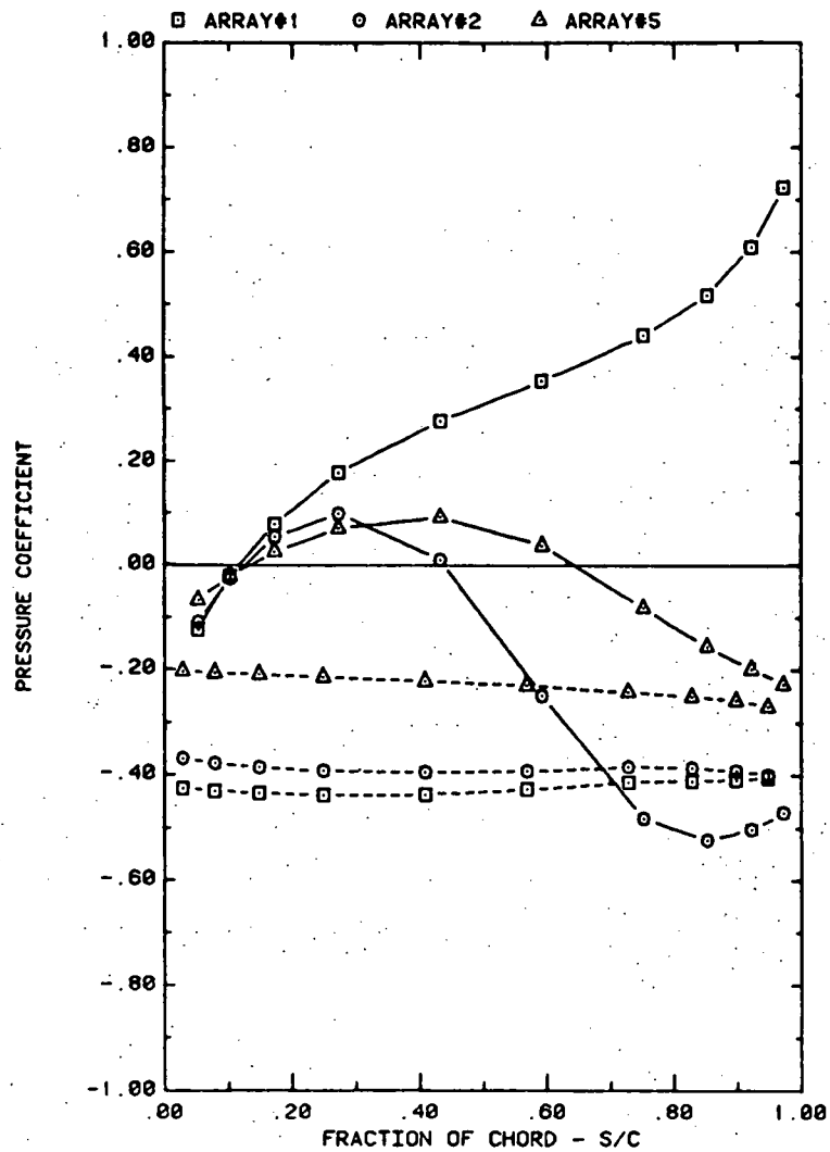
FRONT AND BACK PRESSURES ON VARIOUS ARRAYS FOR SEPARATION = 1.5C EFFECT OF ARRAY CONFIGURATION FOR ATTACK ANGLE, ALPHA = 20
