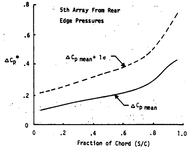
Figure 4-7. Array Chordwise Pressure Coefficient Distribution Located .15 Chord Lengths from Side Edge for Head-On and Rearward Winds (No Fence)
