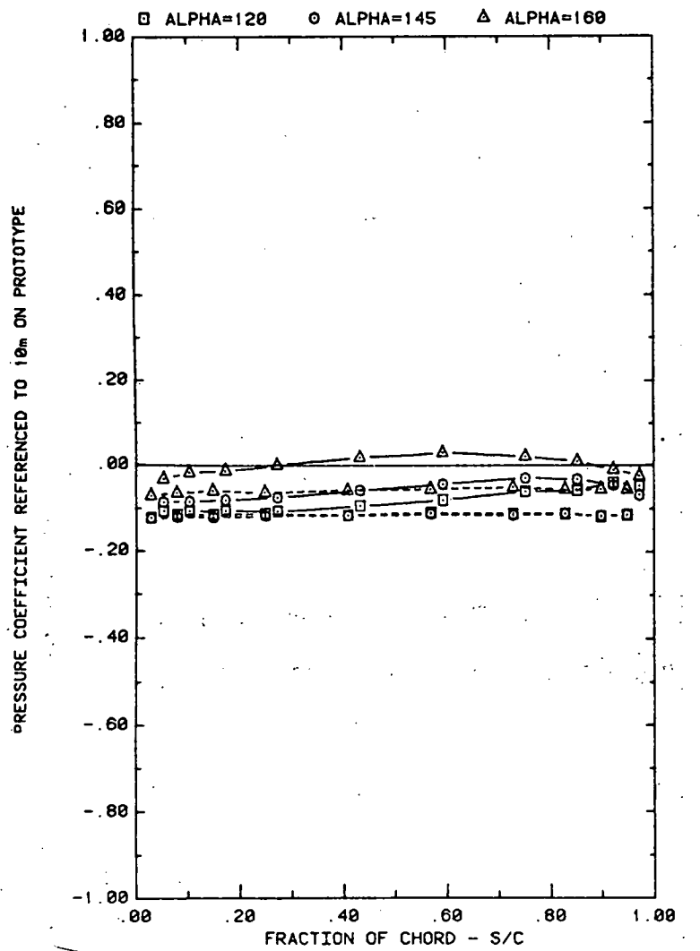
FRONT AND BACK PRESSURES ON ARRAY #5 IN BOUNDARY LAYER EFFECT OF ATTACK ANGLE FOR SPACING = 2C
