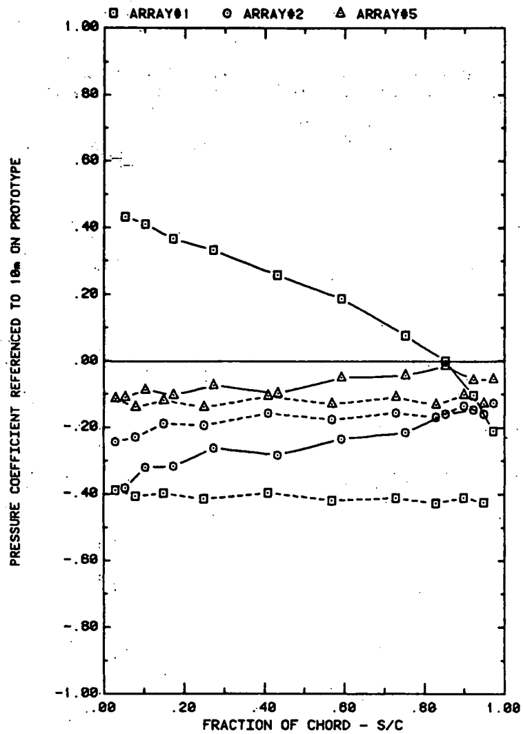
FRONT AND BACK PRESSURES ON ARRAYS IN BOUNDARY LAYER, X = 1.5C EFFECT OF ARRAY CONFIGURATION ON ATTACK ANGLE 145^\circ , H/C = 0.25
