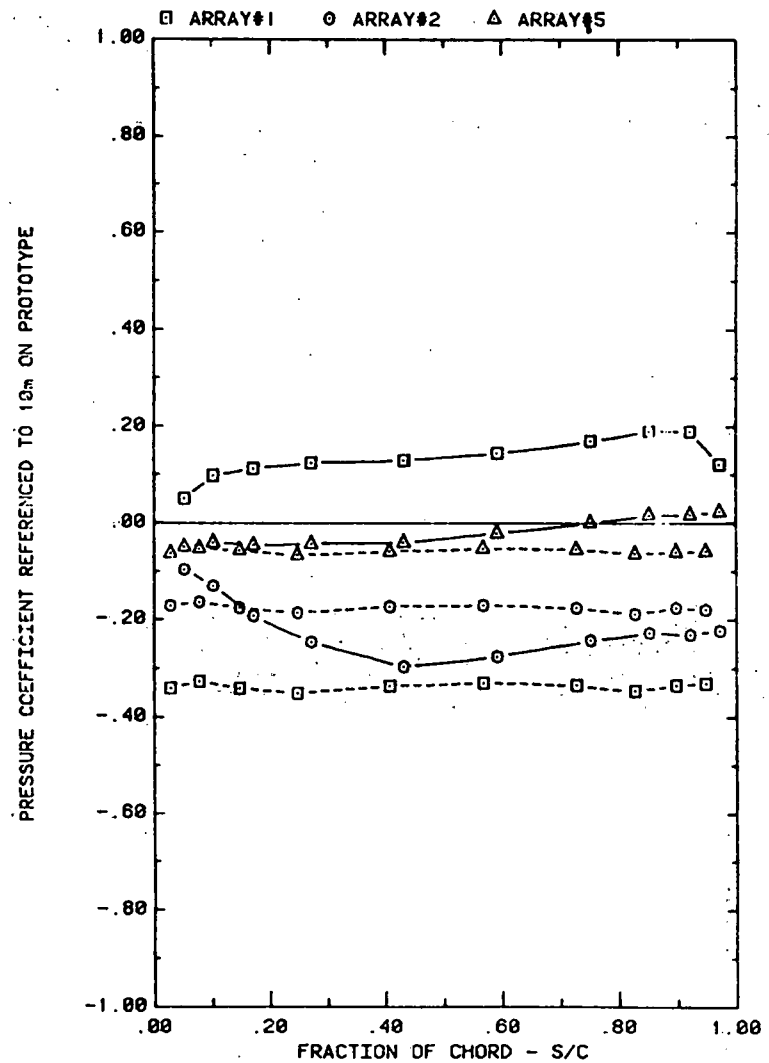
FRONT AND BACK PRESSURES ON VARIOUS ARRAYS WITH SEPARATION = 2C EFFECT OF ARRAYS WITH ATTACK ANGLE=90, H=3°, P=30%, AND D=5°
