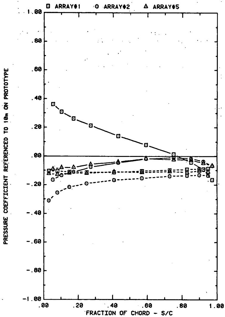
FRONT AND BACK PRESSURES ON ARRAYS IN BOUNDARY LAYER, X = 1.5C EFFECT OF ARRAY CONFIGURATION ON ATTACK ANGLE 160^\circ , H/C = 0.25
