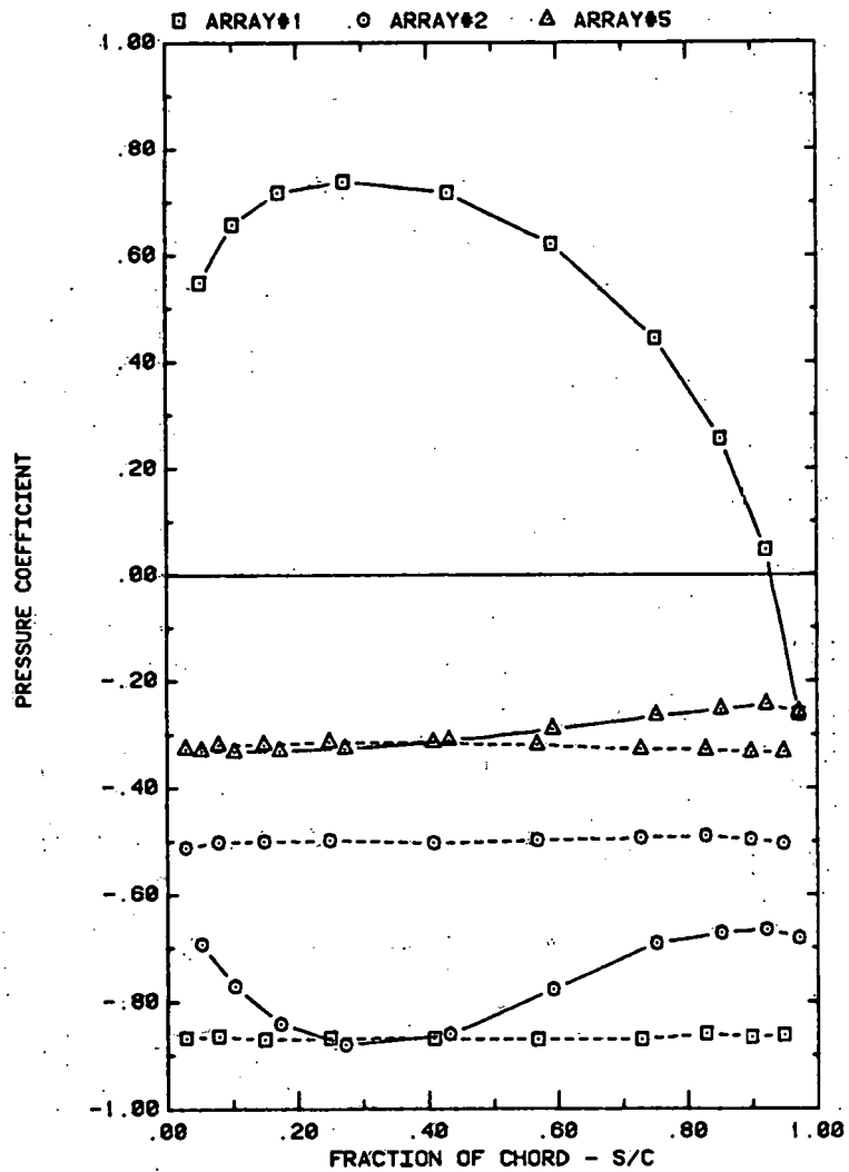
FRONT AND BACK PRESSURES ON VARIOUS ARRAYS FOR SEPARATION = 2C EFFECT OF ARRAY CONFIGURATION FOR ATTACK ANGLE, \alpha = 120
