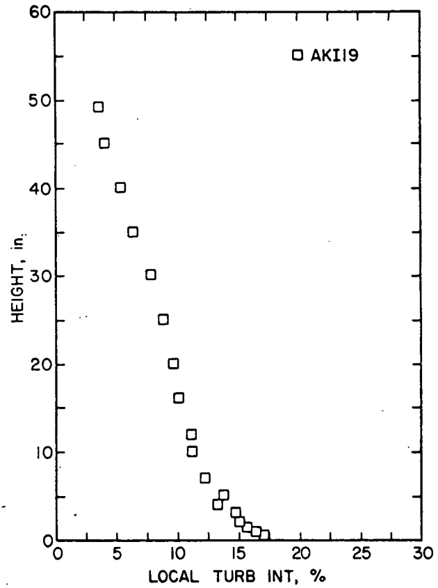
Figure 3. Mean Velocity and Turbulence Distribution in Nonuniform Flow
