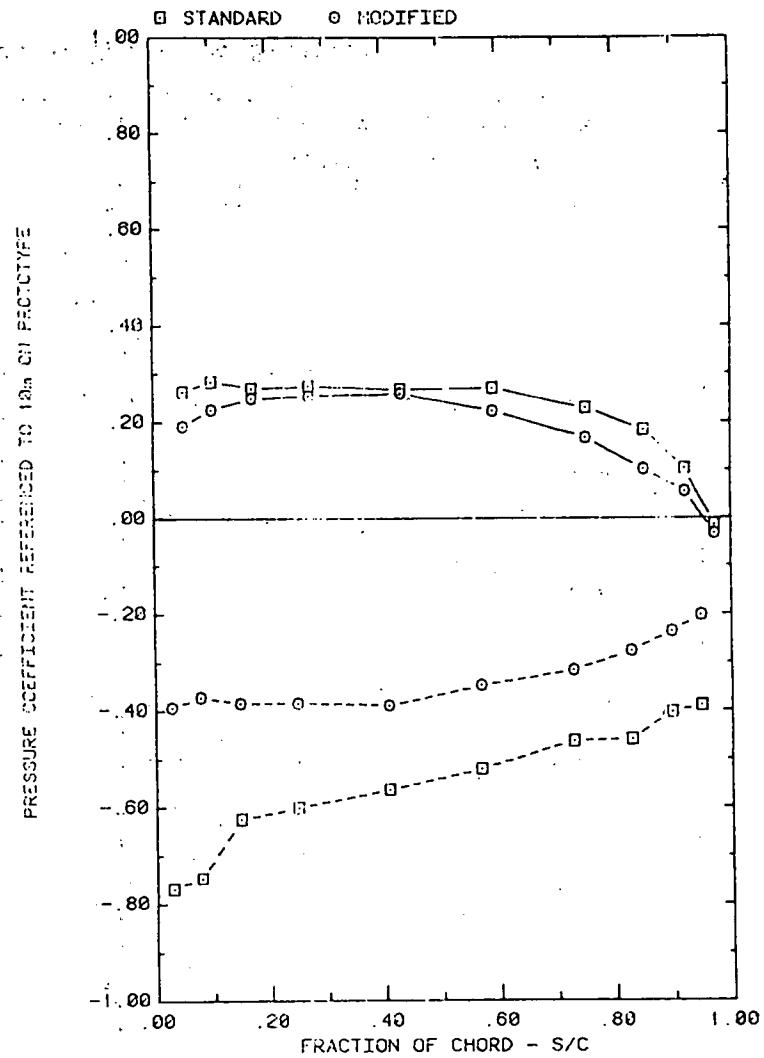
FRONT AND BACK PRESSURES ON ARRAY #2 WITH X=2C , AND WIND=45 EFFECT OF TAP LOCATION; \alpha=145^\circ , H=3^\circ , D=10^\circ , FC=1 , AND P=30\%
