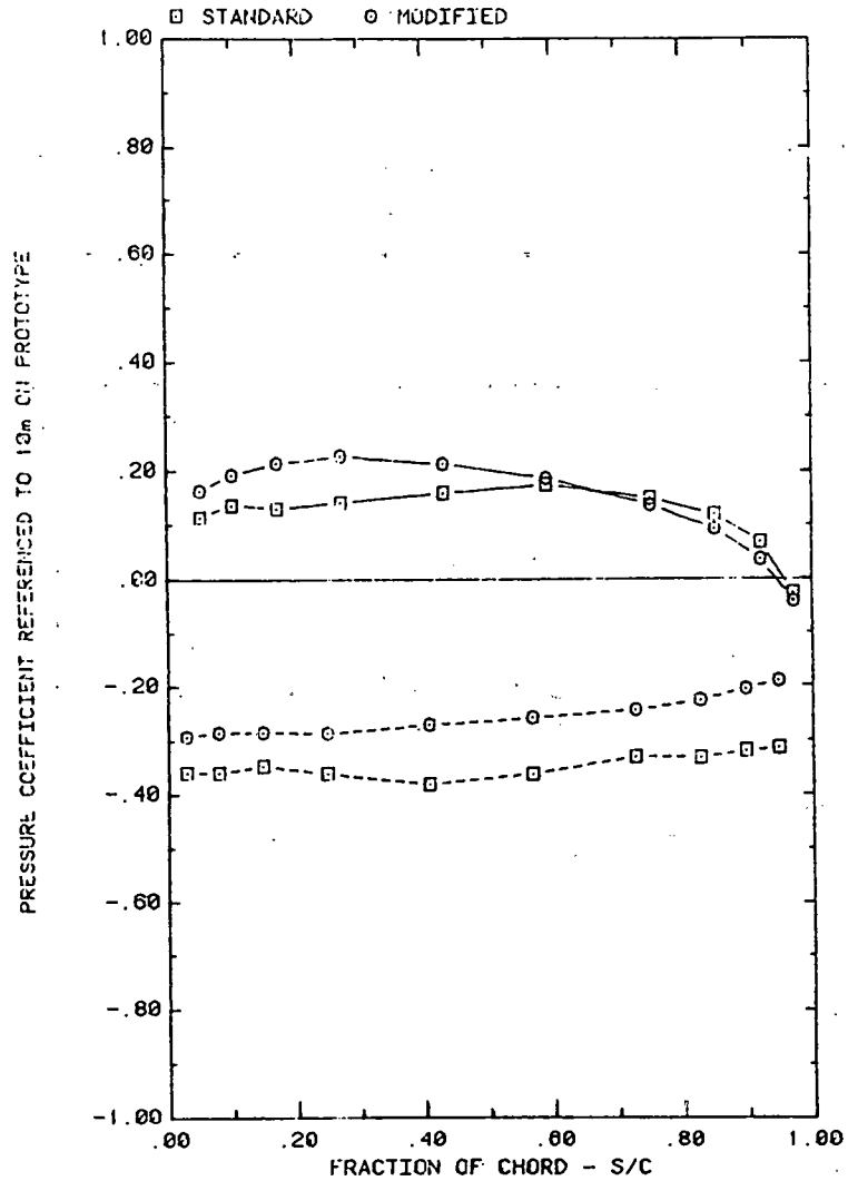
FRONT AND BACK PRESSURES ON ARRAY #3 WITH X=2C , AND WIND=45° EFFECT OF TAP LOCATION; \alpha=145^\circ , H=3^\circ , D=10^\circ , FC=1 , AND P=30\%
