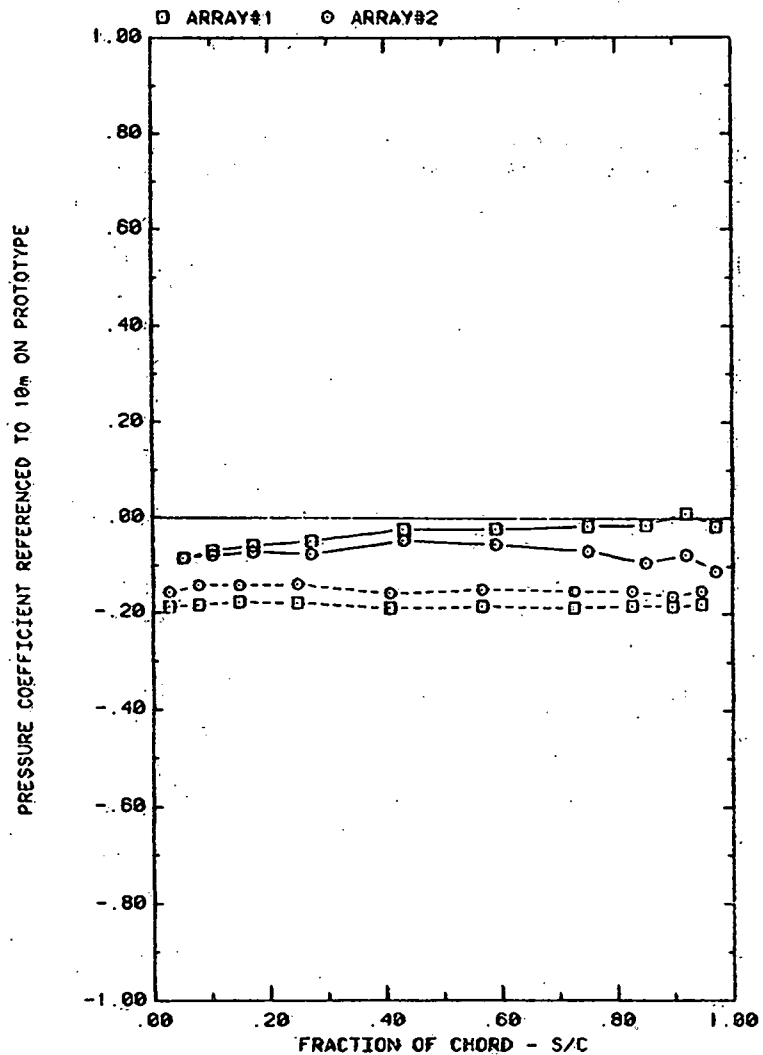
FRONT AND BACK PRESSURES ON ARRAYS #1&2 WITH SEPARATION = 2C EFFECT OF ARRAY WITH ALPHA=35, H=5", D=10", AND P=30%
