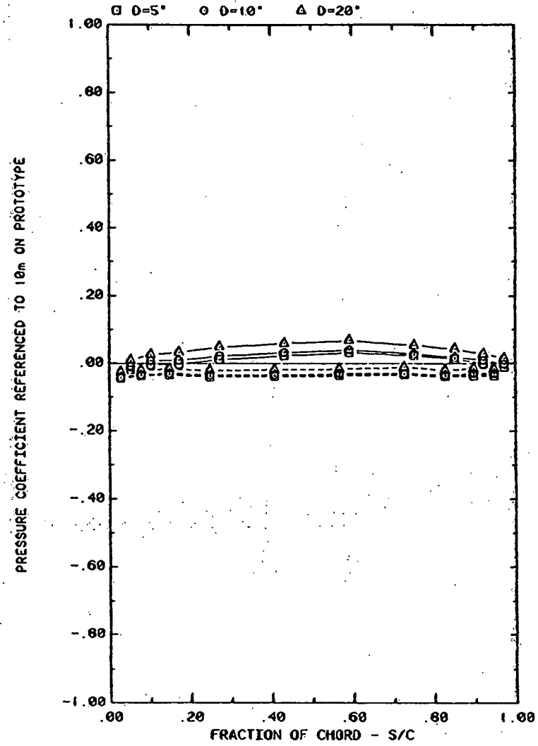
FRONT AND BACK PRESSURES ON ARRAY #5 WITH SEPARATION = .2C EFFECT OF FENCE DISTANCE WITH H=3^\circ , P=30\% , AND \alpha=160
