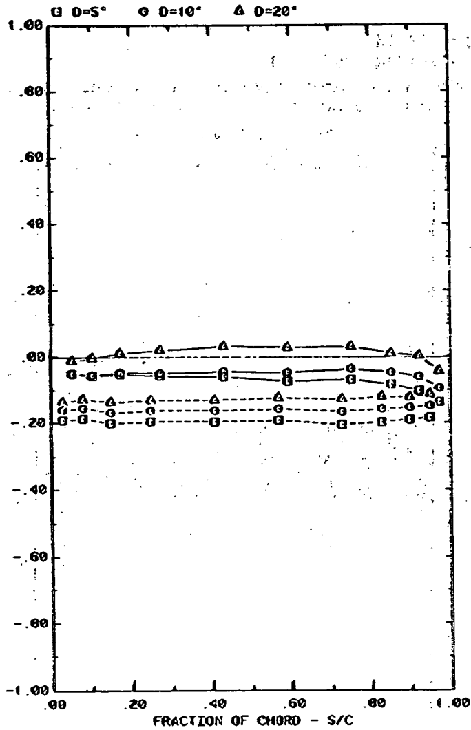
FRONT AND BACK PRESSURES ON ARRAY #1 WITH SEPARATION = 2C EFFECT OF FENCE DISTANCE WITH H=3^\circ , P=30\% , AND \alpha=145
