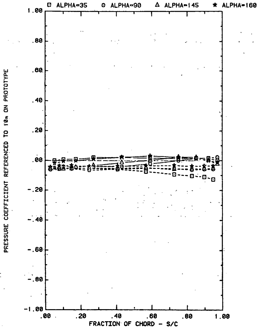
FRONT AND BACK PRESSURES ON ARRAY #5 WITH SEPARATION = 2C EFFECT OF ATTACK ANGLE WITH H=3^\circ , P=30\% , AND D=5^\circ
