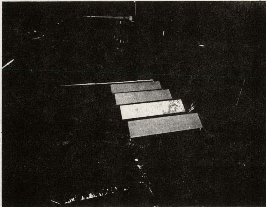
Figure 8. 1:12 Scale Models in Meteorological Wind Tunnel
