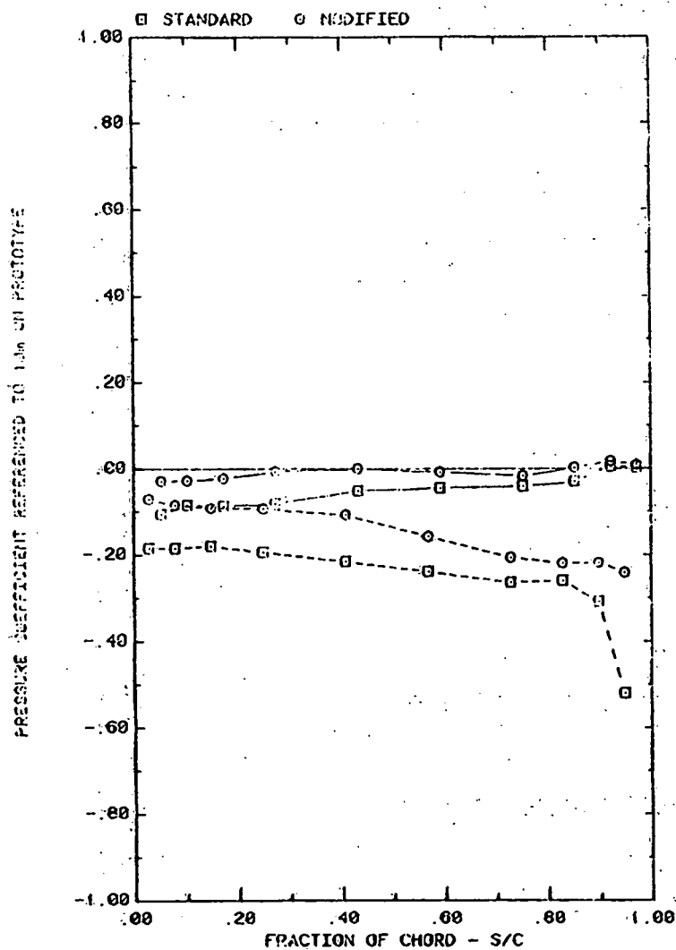
FRONT AND BACK PRESSURES ON ARRAY #2 WITH X=2C , AND WIND=45 EFFECT OF TAP LOCATION; \alpha=35^\circ , H=3^\circ , D=10^\circ , FC=3 , AND P=30\%
