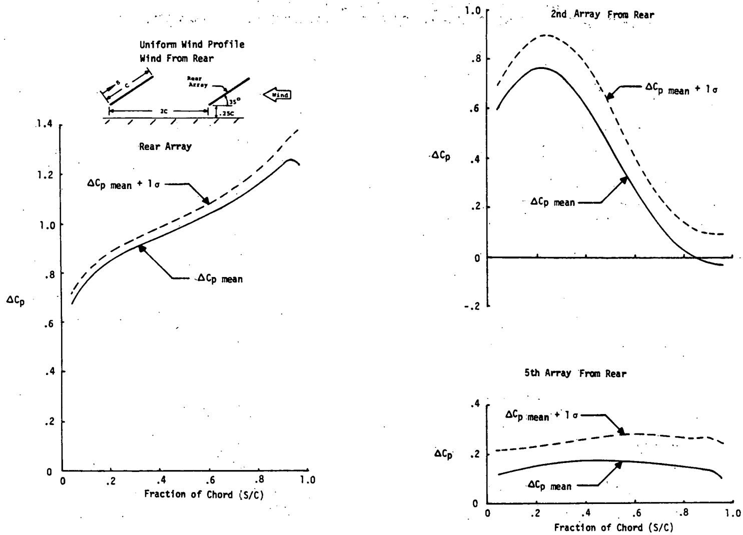
Figure 4-1d. Array Chordwise Pressure Coefficient Distribution in Uniform Wind Velocity Profile (Tilt Angle = 35°, Wind from Rear)
