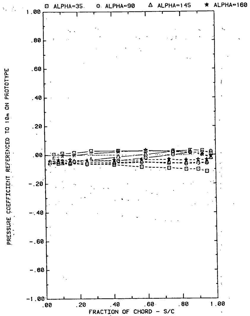
FRONT AND BACK PRESSURES ON ARRAY #5 WITH SEPARATION = 2C EFFECT OF ATTACK ANGLE WITH H=3", P=30%, AND D=10"
