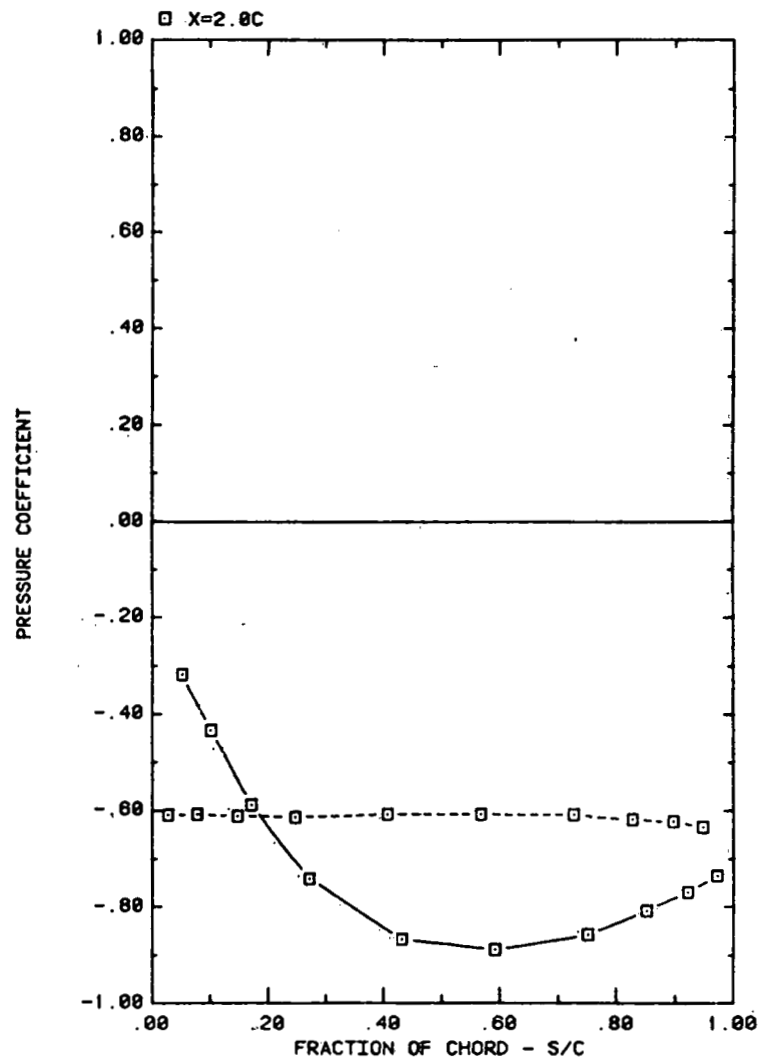
FRONT AND BACK PRESSURES ON ARRAY #2 IN UNIFORM FLOW. EFFECT OF SEPARATION (X) ON ATTACK ANGLE 90, H/C = 0.25
