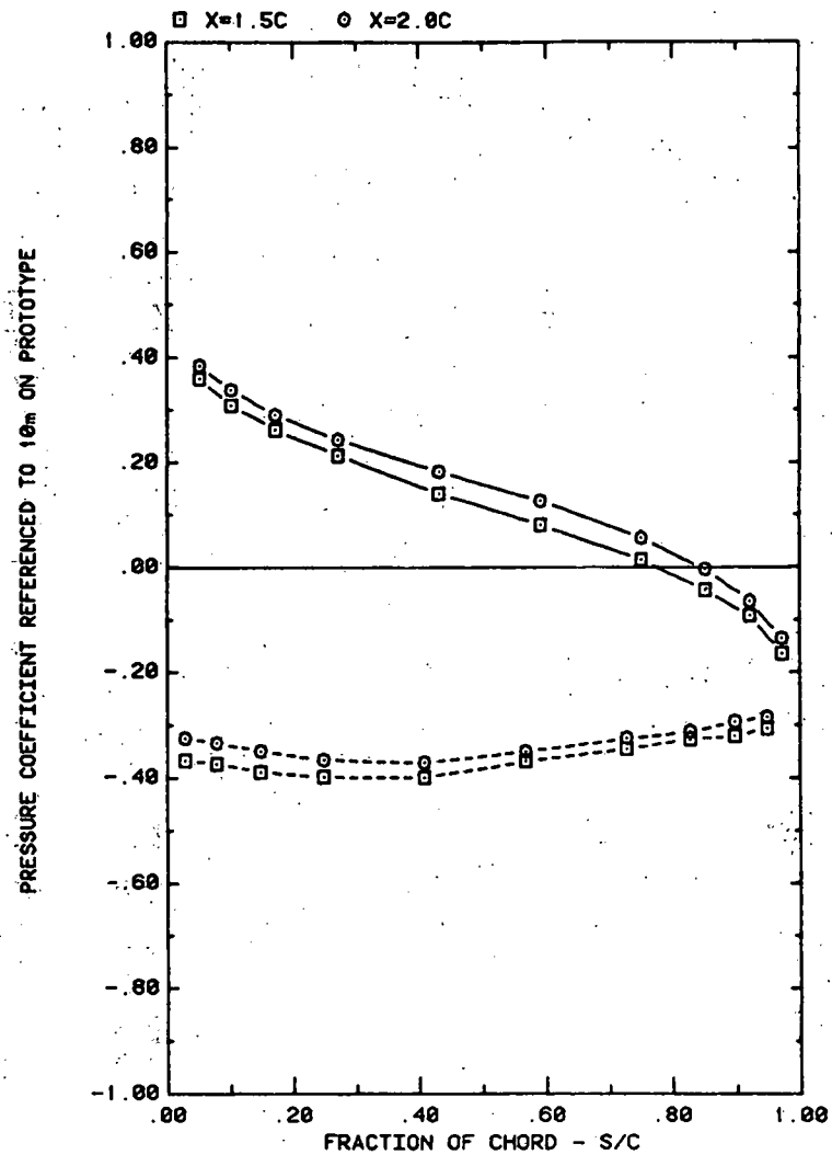
FRONT AND BACK PRESSURES ON ARRAY #1 IN BOUNDARY LAYER EFFECT OF SEPARATION (X) ON ATTACK ANGLE 160, H/C = 0.25
