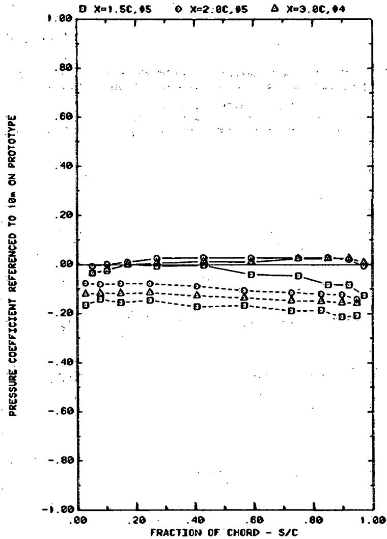
FRONT AND BACK PRESSURES ON ARRAY #4 OR #5 IN BOUNDARY LAYER EFFECT OF SEPARATION (X) ON ATTACK ANGLE 35; H/C = 0.25
