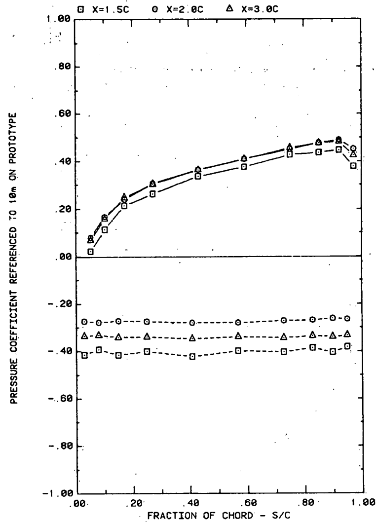
FRONT AND BACK PRESSURES ON ARRAY #1 IN BOUNDARY LAYER EFFECT OF SEPARATION ( X ) ON ATTACK ANGLE 35^\circ , H/C = 0.25
