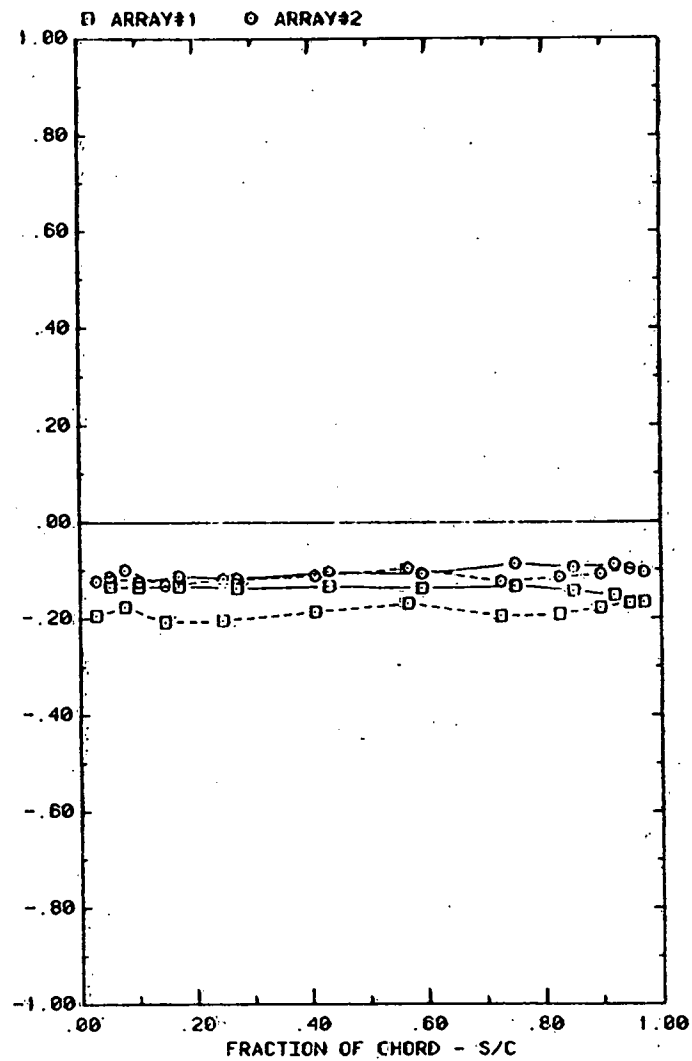
FRONT AND BACK PRESSURES ON ARRAYS #1&#2 WITH SEPARATION = 2C EFFECT OF ARRAY WITH \alpha=145^\circ , H=4^\circ , D=10^\circ , AND P=30\%
