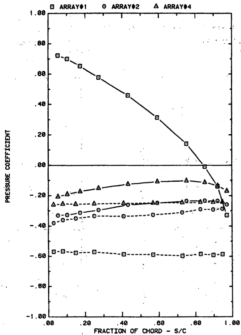
FRONT AND BACK PRESSURES ON VARIOUS ARRAYS FOR SEPARATION = 3C EFFECT OF ARRAY CONFIGURATION FOR ATTACK ANGLE, ALPHA = 145
