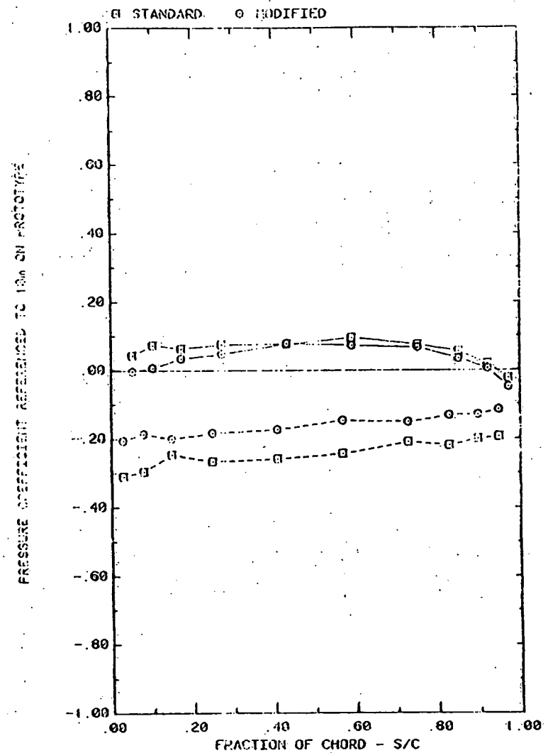
FRONT AND BACK PRESSURES ON ARRAY #2 WITH X=2C , AND WIND=45 EFFECT OF TAP LOCATION; \alpha=145^\circ , H=3^\circ , D=10^\circ , FC=3 , AND P=30\%
