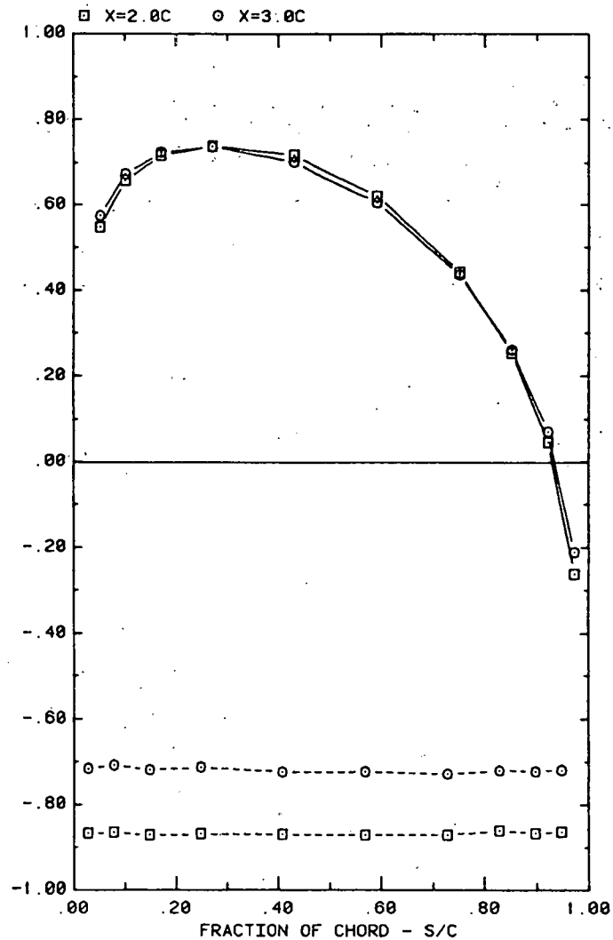
FRONT AND BACK PRESSURES ON ARRAY #1 IN UNIFORM FLOW EFFECT OF SEPARATION (X) ON ATTACK ANGLE 120, H/C = 0.25
