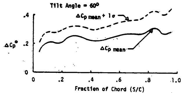
Figure 4-5. Effect of a Fence on Array Chordwise Pressure Coefficient Distribution for Head-On and Rearward Winds.
