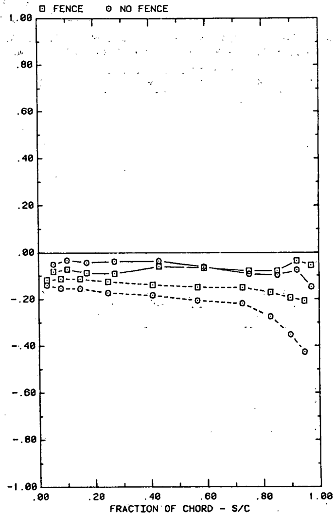
FRONT AND BACK PRESSURES ON ARRAY #2 WITH X=2C , AND WIND=0 EFFECT OF FENCE ON ARRAY EDGE; \alpha=35^\circ , H=3^\circ , D=10^\circ , AND P=30\%
