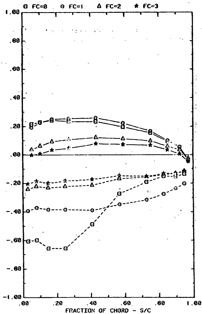
FRONT AND BACK PRESSURES 3.6° IN FROM EDGE OF ARRAY#2; WIND=45 EFFECT OF FC WITH ALPHA=145, H=3°, D=10°, P=30%, AND X=2C
