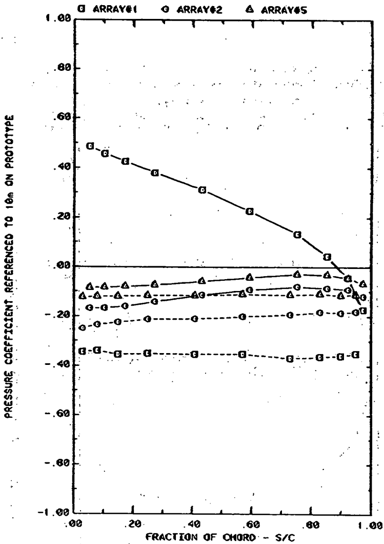
FRONT AND BACK PRESSURES ON ARRAYS IN BOUNDARY LAYER, \alpha = 145^\circ EFFECT OF ARRAY CONFIGURATION ON ATTACK ANGLE 145, h/c = 0.25
