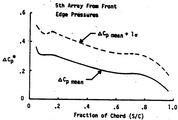
Figure 4-7. Array Chordwise Pressure Coefficient Distribution Located .15 Chord Lengths from Side Edge for Head-On and Rearward Winds (No Fence)
