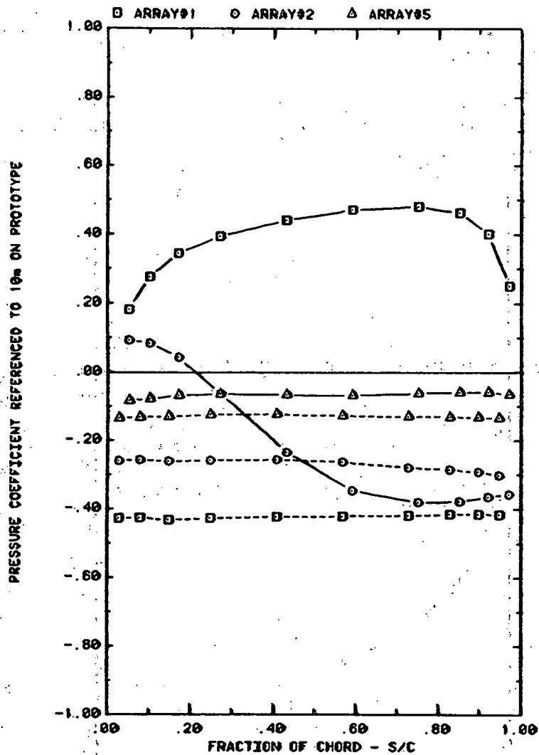
FRONT AND BACK PRESSURES ON ARRAYS IN BOUNDARY LAYER, \alpha = 60^\circ EFFECT OF ARRAY CONFIGURATION ON ATTACK ANGLE 60^\circ , H/C = 0.25
