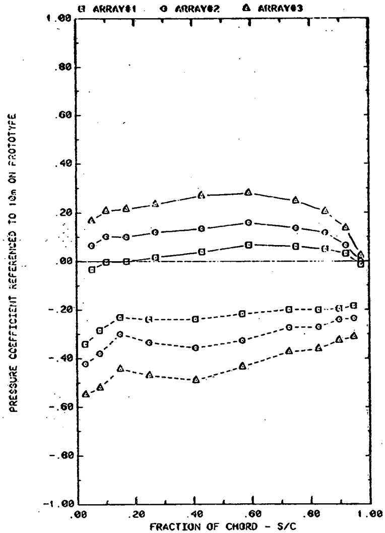
FRONT AND BACK PRESSURES 0.6° IN FROM ARRAY EDGE; X=2C, WIND=45 EFFECT OF ARRAY WITH ALPHA=145, FC=2, H=3°, D=10°, AND P=30%
