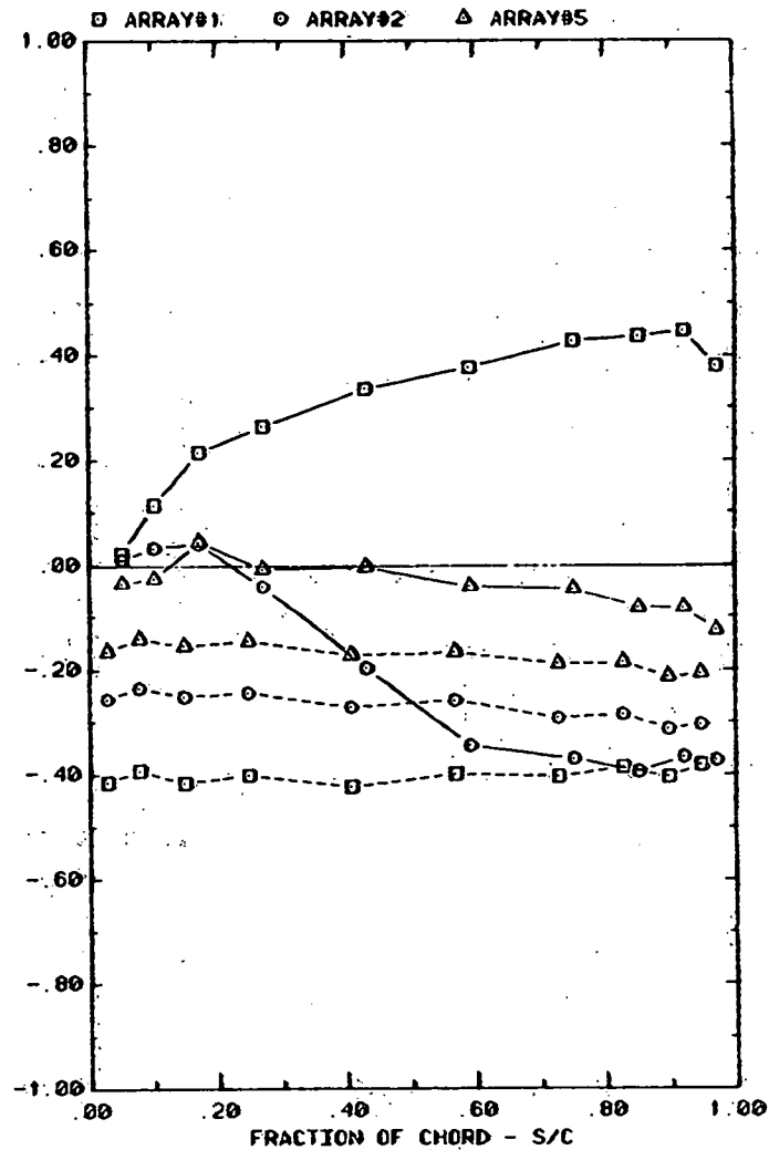
FRONT AND BACK PRESSURES ON ARRAYS IN BOUNDARY LAYER, x = 1.5c EFFECT OF ARRAY CONFIGURATION ON ATTACK ANGLE 35^\circ , h/c = 0.25
