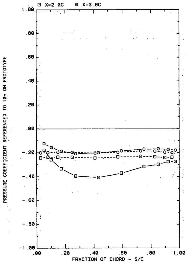
FRONT AND BACK PRESSURES ON ARRAY #2 IN BOUNDARY LAYER EFFECT OF SEPARATION (X) ON ATTACK ANGLE 120, H/C = 0.25
