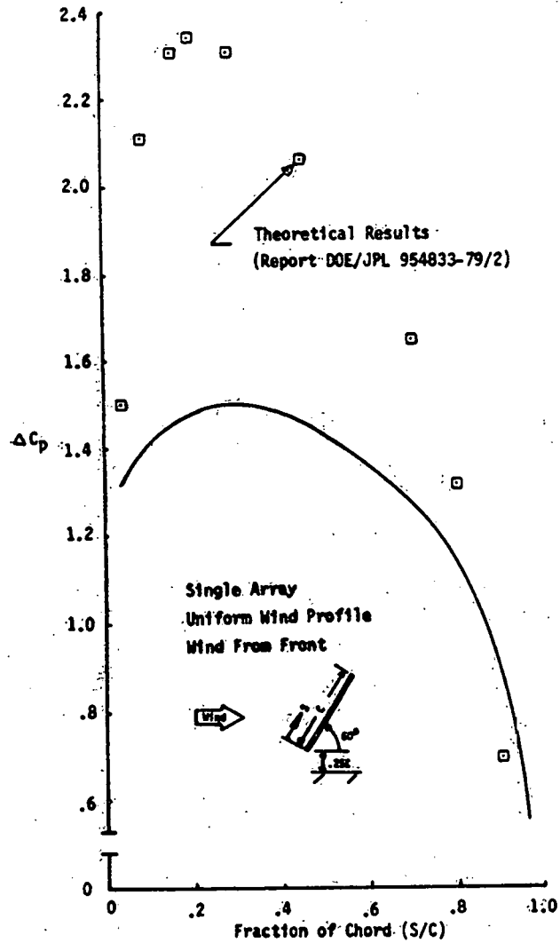
Figure 5-2c. Array Pressure Coefficient Distribution Comparison Between Wind Tunnel Test and Theoretical Methods in Close Ground Proximity (Tilt Angle = 60°)
