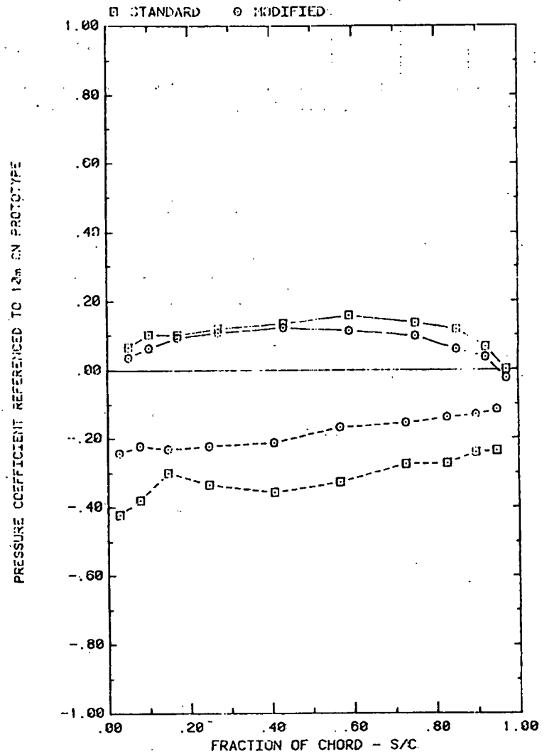
FRONT AND BACK PRESSURES ON ARRAY #2 WITH X=2C , AND WIND=45 EFFECT OF TAP LOCATION; ALPHA=145, H=3°, D=10°, FC=2°, AND P=30%
