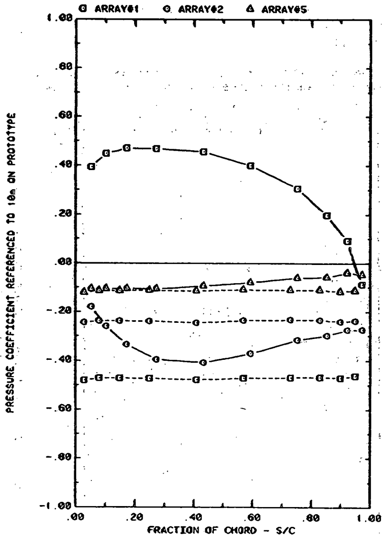
FRONT AND BACK PRESSURES ON ARRAYS IN BOUNDARY LAYER, \alpha = 120^\circ EFFECT OF ARRAY CONFIGURATION ON ATTACK ANGLE 120, h/c = 0.25
