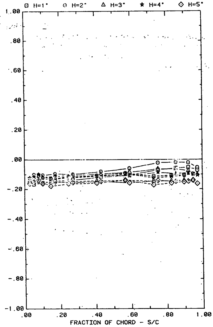
FRONT AND BACK PRESSURES ON ARRAY #2 WITH SEPARATION = 2C EFFECT OF FENCE HEIGHT WITH ALPHA=145, D=10°, AND P=30%
