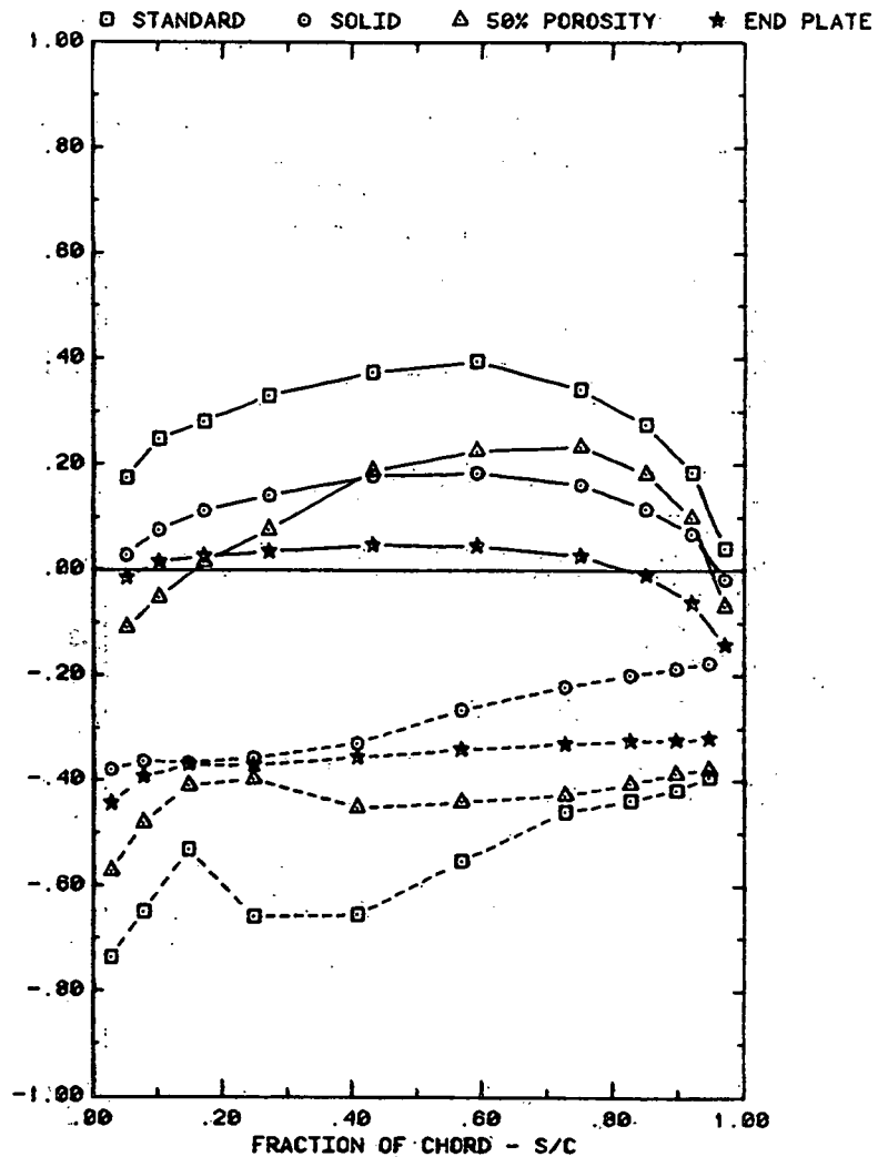
FRONT AND BACK PRESSURES ON ARRAYS; X = 2C , WIND = 45 EFFECT OF EXTENSIONS; ARRAY = 1, ALPHA = 145, FC = 1
