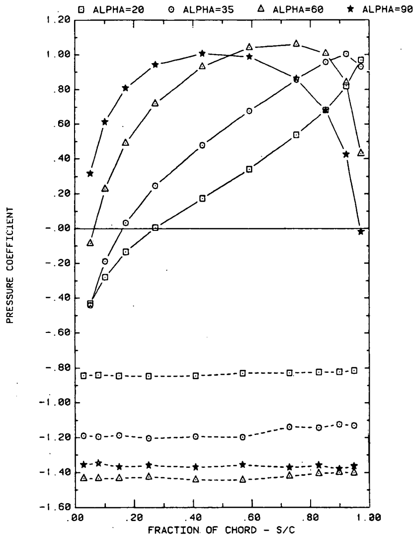
FRONT AND BACK PRESSURES ON A SINGLE ARRAY IN UNIFORM FLOW EFFECT OF ATTACK ANGLE FOR GROUND CLEARANCE, H/C = INFINITY
