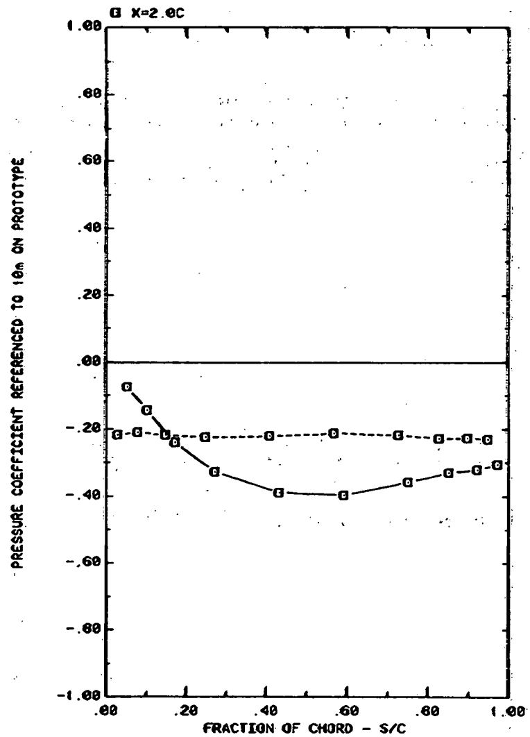
FRONT AND BACK PRESSURES ON ARRAY #2 IN BOUNDARY LAYER EFFECT OF SEPARATION (X) ON ATTACK ANGLE 90, H/C = 0.25
