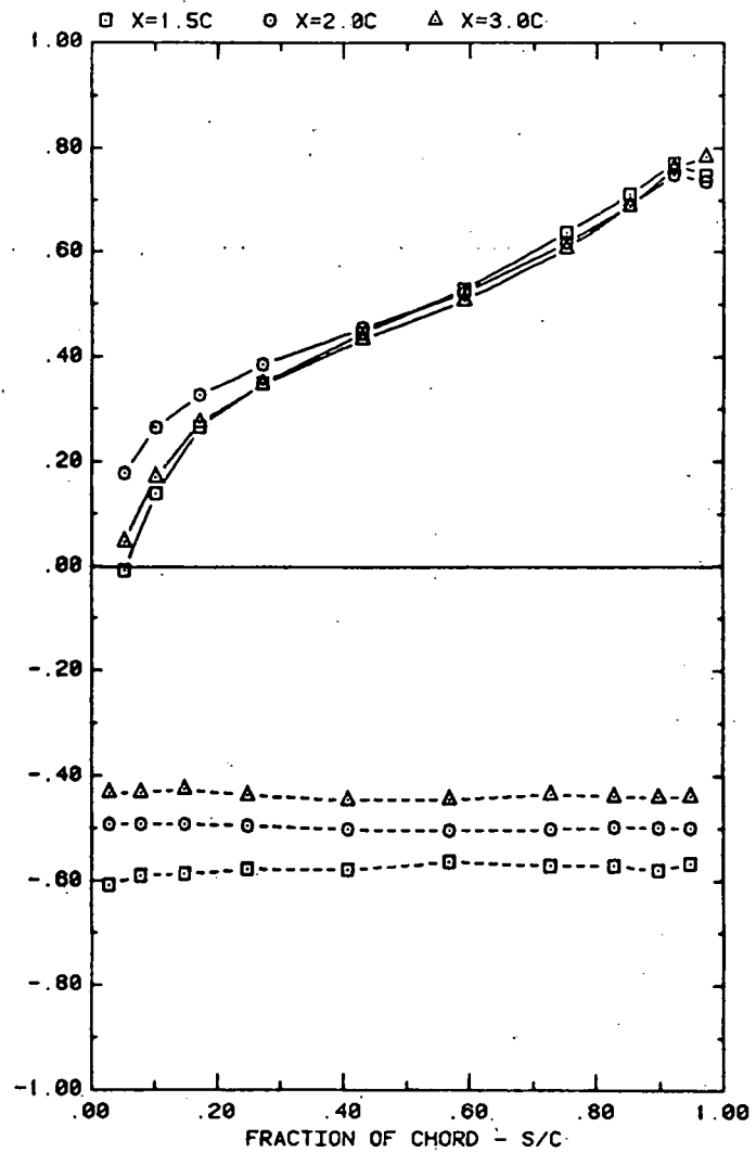
FRONT AND BACK PRESSURES ON ARRAY #1 IN UNIFORM FLOW EFFECT OF SEPARATION (X) ON ATTACK ANGLE 35, H/C = 0.25
