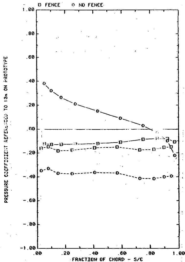
FRONT AND BACK PRESSURES ON ARRAY #1 WITH X=2C , AND WIND= 0^\circ EFFECT OF FENCE ON ARRAY EDGE; \alpha=145^\circ , H=3^\circ , D=10^\circ , AND P=30\%
