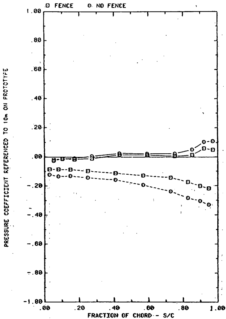
FRONT AND BACK PRESSURES ON ARRAY #5 WITH X=2C , AND WIND= 0^\circ EFFECT OF FENCE ON ARRAY EDGE; \alpha=35^\circ , H=3^\circ , D=10^\circ , AND P=30\%
