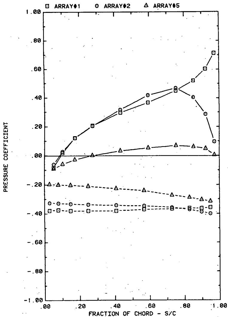
FRONT AND BACK PRESSURES ON VARIOUS ARRAYS FOR SEPARATION = 2C EFFECT OF ARRAY CONFIGURATION FOR ATTACK ANGLE, ALPHA = 20
