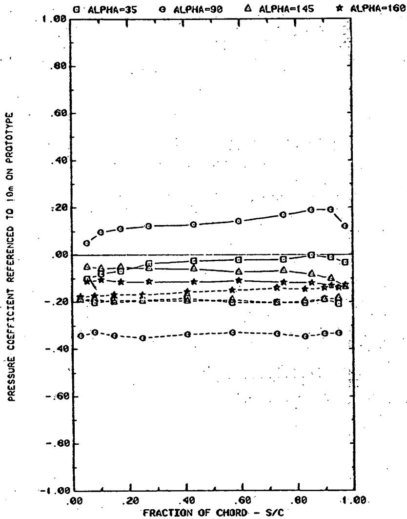
FRONT AND BACK PRESSURES ON ARRAY #1 WITH SEPARATION = 2C EFFECT OF ATTACK ANGLE WITH H=3^\circ , P=30\% , AND D=5^\circ
