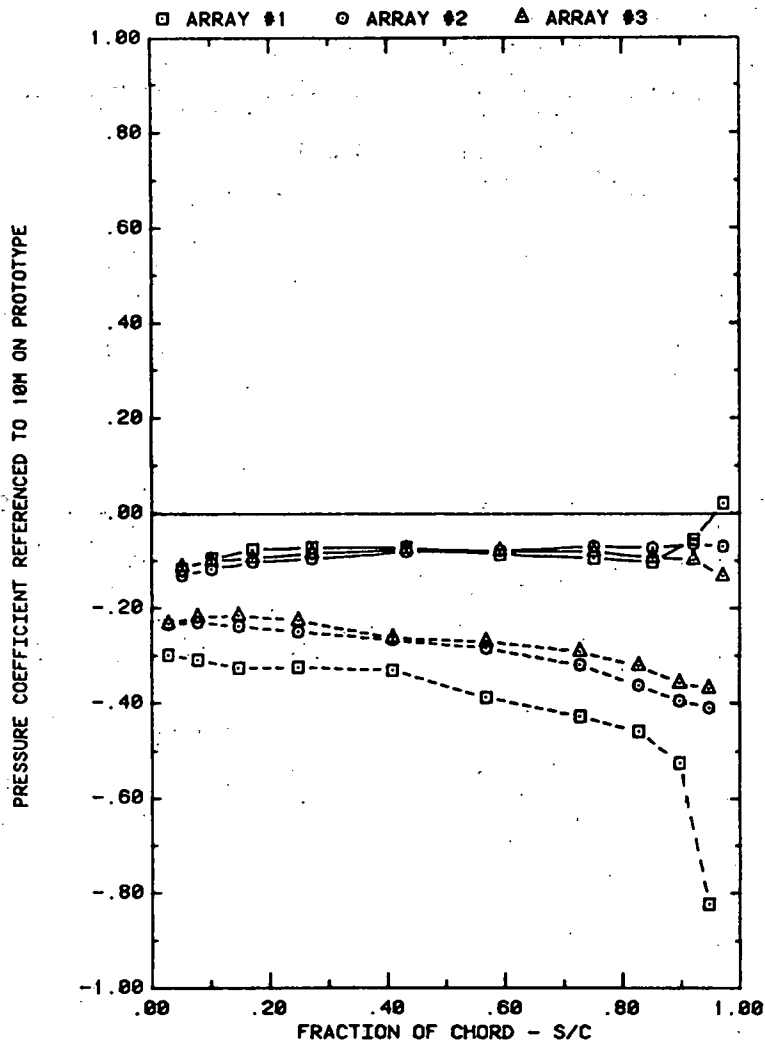
FRONT AND BACK PRESSURES ON ARRAYS #1, 2 & 3 \END PLATE EFFECT OF ARRAY WITH ALPHA = 35, WIND = 45, X = 2C, FC = 1
