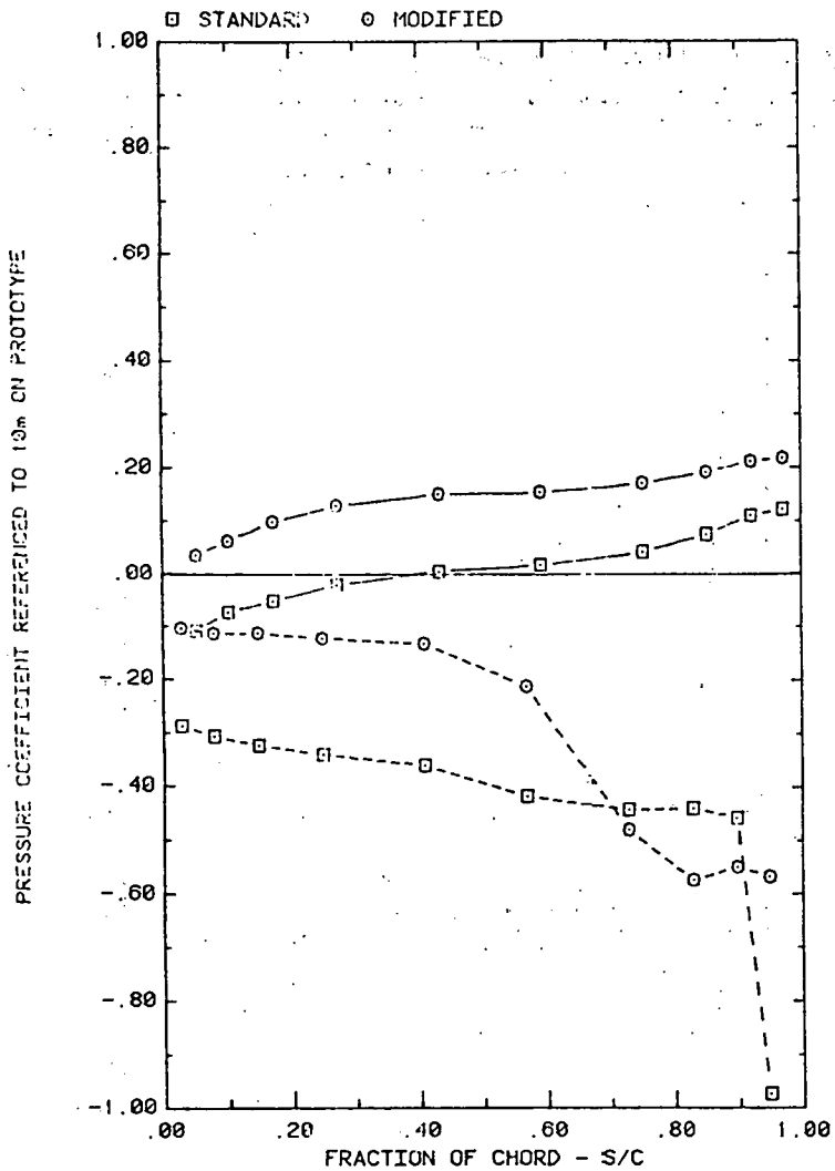
FRONT AND BACK PRESSURES ON ARRAY #2 WITH X=2C , AND WIND=45 EFFECT OF TAP LOCATION; \alpha=35^\circ , H=3^\circ , D=10^\circ , FC=1 , AND P=30\%
