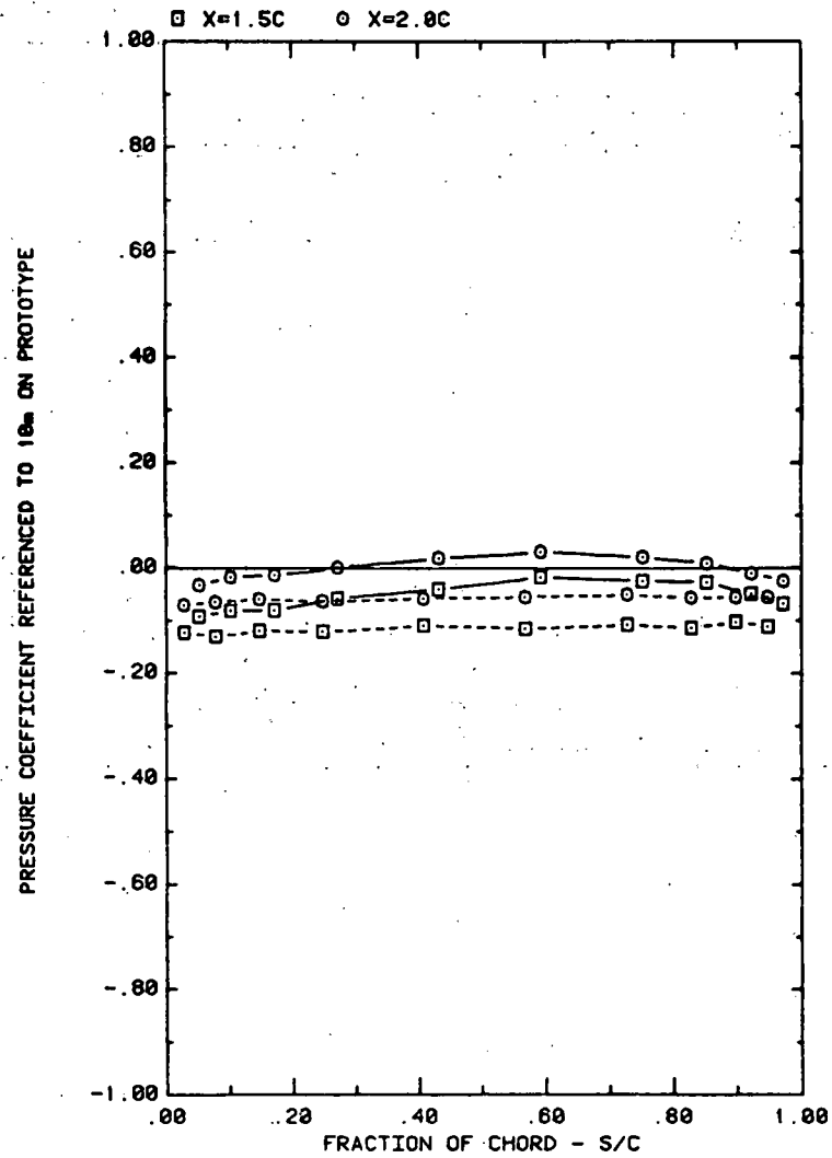
FRONT AND BACK PRESSURES ON ARRAY #5 IN BOUNDARY LAYER EFFECT OF SEPARATION (X) ON ATTACK ANGLE 160, H/C = 0.25
