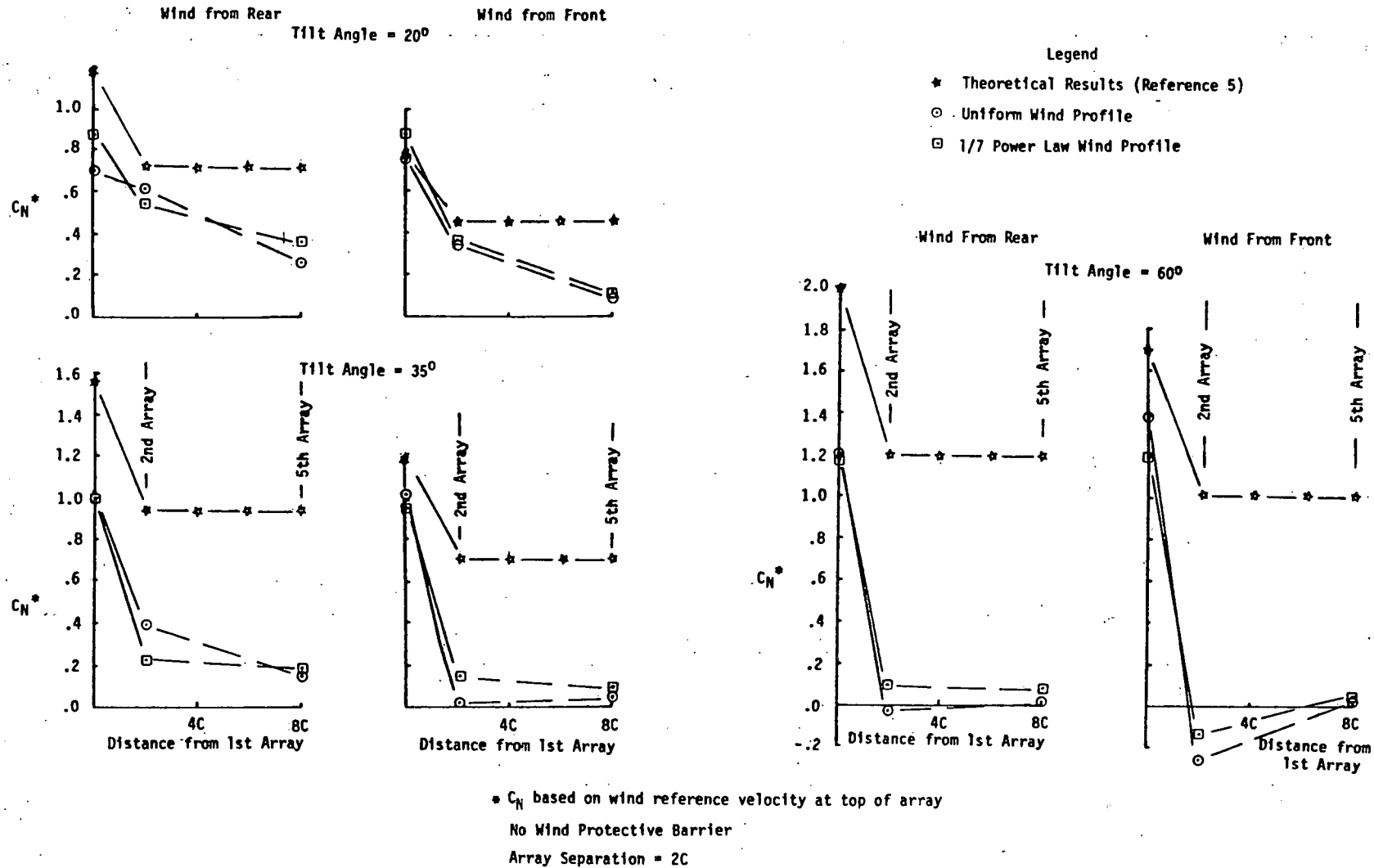
Figure 5-4. Array Normal Force Coefficient Comparison Between Wind Tunnel Test and Theoretical Methods
