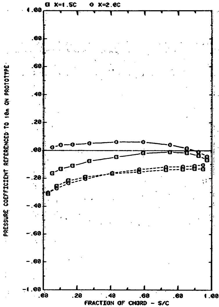
FRONT AND BACK PRESSURES ON ARRAY #2 IN BOUNDARY LAYER EFFECT OF SEPARATION (X) ON ATTACK ANGLE 160, H/C = 0.25
