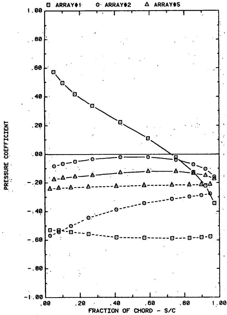
FRONT AND BACK PRESSURES ON VARIOUS ARRAYS FOR SEPARATION = 2C EFFECT OF ARRAY CONFIGURATION FOR ATTACK ANGLE, ALPHA = 160
