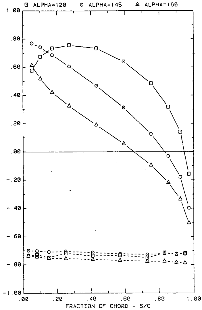
FRONT AND BACK PRESSURES ON A SINGLE ARRAY IN UNIFORM FLOW EFFECT OF ATTACK ANGLE FOR GROUND CLEARANCE, H/C = 0.25
