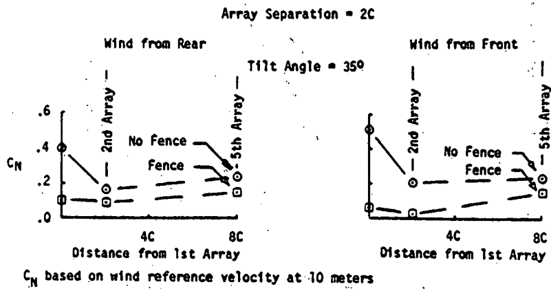
Figure 4-10. Effect of Fence on Array Edge Normal Force Coefficients for Head-On and Rearward Winds
