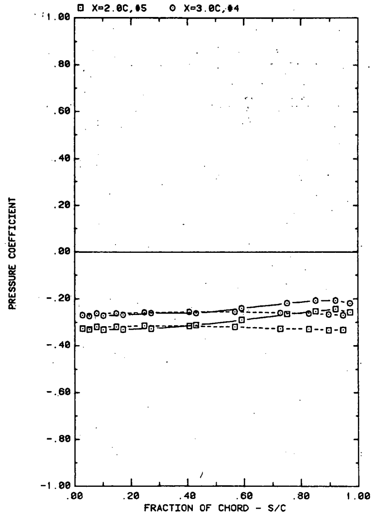
FRONT AND BACK PRESSURES ON ARRAY #4 OF #5 IN UNIFORM FLOW EFFECT OF SEPARATION (X) ON ATTACK ANGLE 20, H/C = 0.25
