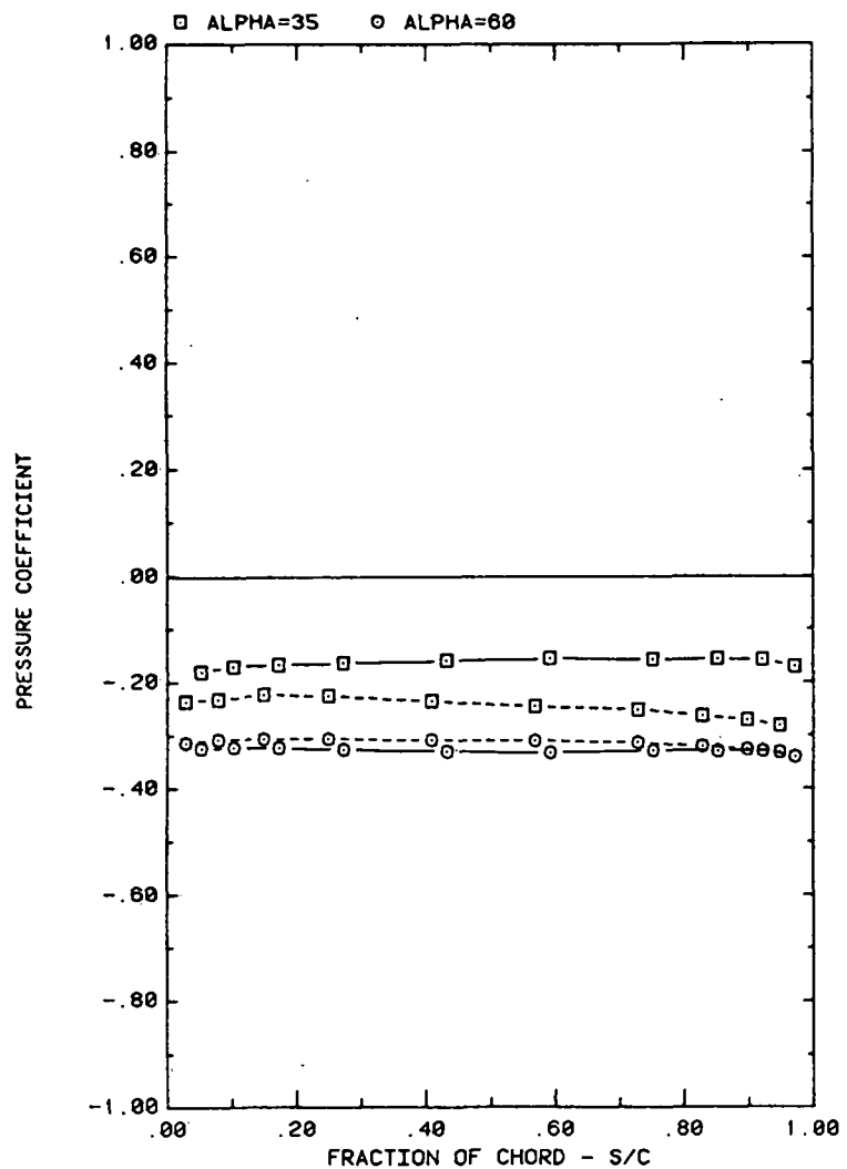
FRONT AND BACK PRESSURES ON ARRAY #4 IN UNIFORM FLOW EFFECT OF ATTACK ANGLE FOR SPACING = 3C
