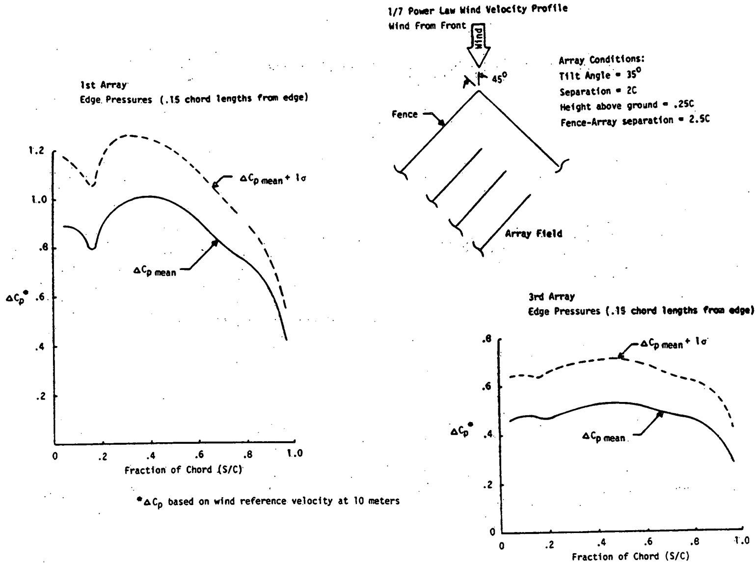
Figure 4-11c. Effect of Oblique Winds on Array Edge Pressure Distribution (Conventional Fence, Wind from Front)
