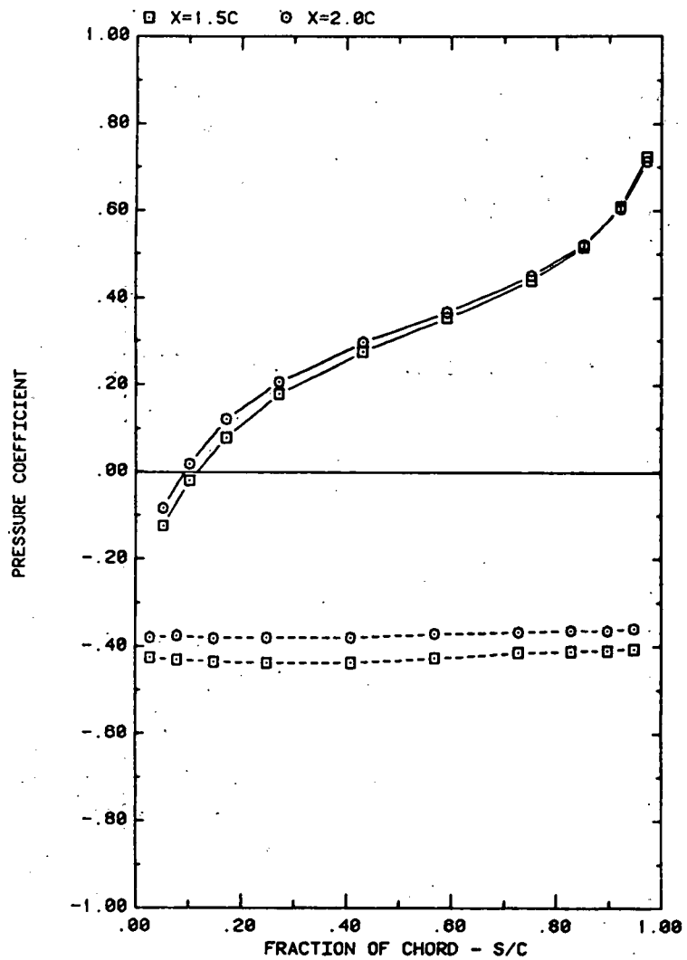
FRONT AND BACK PRESSURES ON ARRAY #1 IN UNIFORM FLOW EFFECT OF SEPARATION (X) ON ATTACK ANGLE 20, H/C = 0.25
