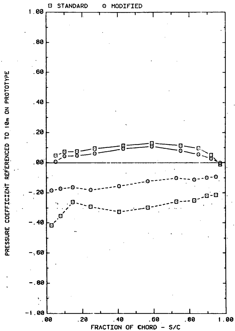
FRONT AND BACK PRESSURES ON ARRAY #3 WITH X=2C, AND WIND=45 EFFECT OF TAP LOCATION; ALPHA=145, H=3°, D=10°, FC=3, AND P=30%
