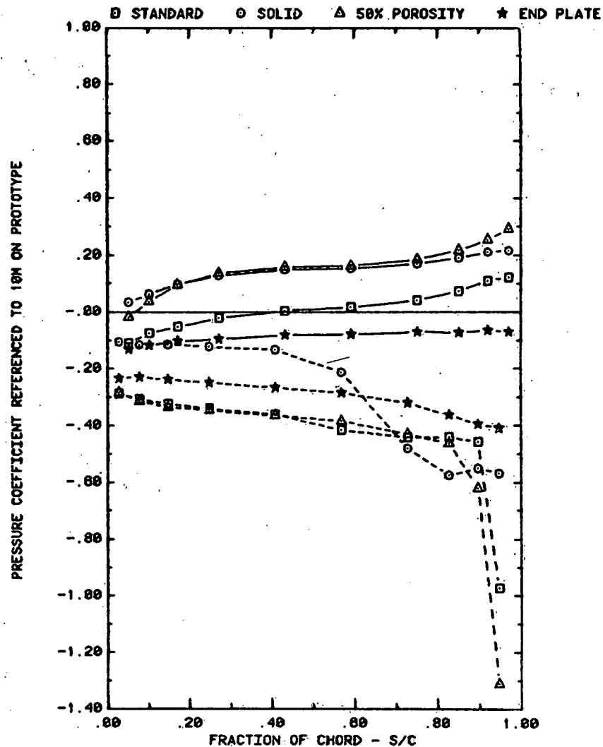
Plot 5-3-2. Corner Study, WD = 45^\circ , Modified Model with Various Extension Effect of Model Configuration
