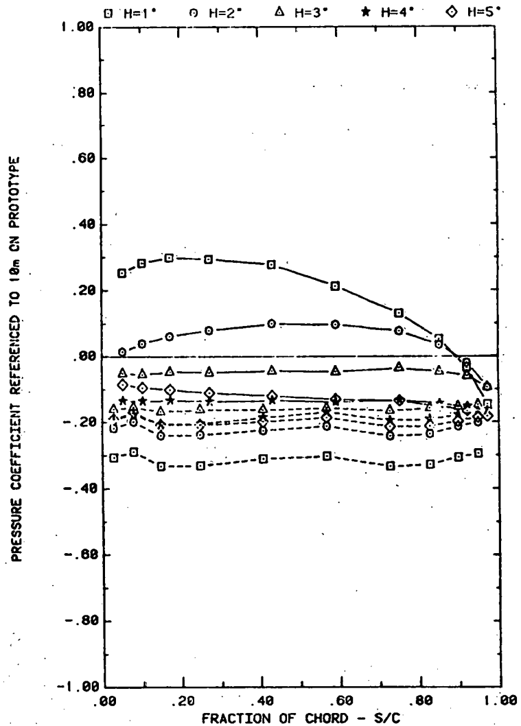
FRONT AND BACK PRESSURES ON ARRAY #1 WITH SEPARATION = 2C EFFECT OF FENCE HEIGHT WITH ALPHA=145, D=10°, AND P=30%
