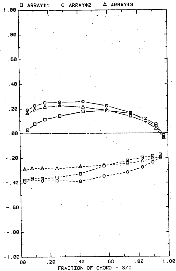
FRONT AND BACK PRESSURES 3.6° IN FROM ARRAY EDGE; X=2C, WIND=45 EFFECT OF ARRAY WITH ALPHA=145, FC=1, H=3°, D=10°, AND P=30%
