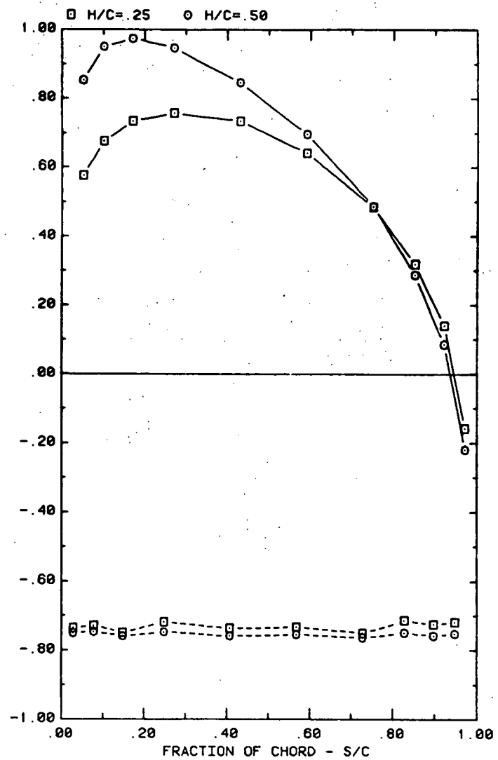
FRONT AND BACK PRESSURES ON A SINGLE ARRAY IN UNIFORM FLOW EFFECT OF GROUND CLEARANCE FOR ATTACK ANGLE, \alpha = 120^\circ
