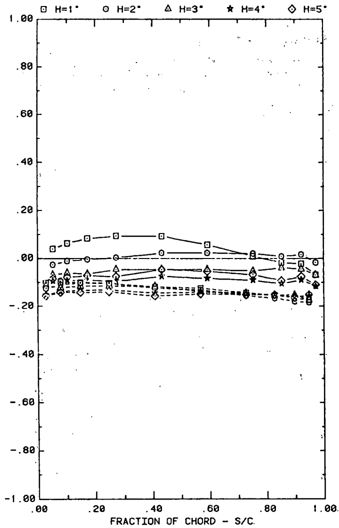
FRONT AND BACK PRESSURES ON ARRAY #2 WITH SEPARATION = 2C EFFECT OF FENCE HEIGHT WITH ALPHA=35, D=10°, AND P=30%
