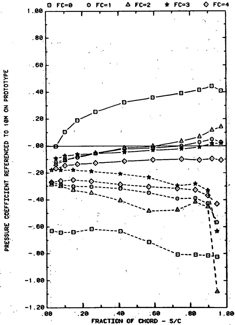
FRONT AND BACK PRESSURES 0.6° IN FROM EDGE OF ARRAY#3; WIND=45 EFFECT OF FC WITH ALPHA=35, H=3°, D=10°, P=30%, AND X=2C
