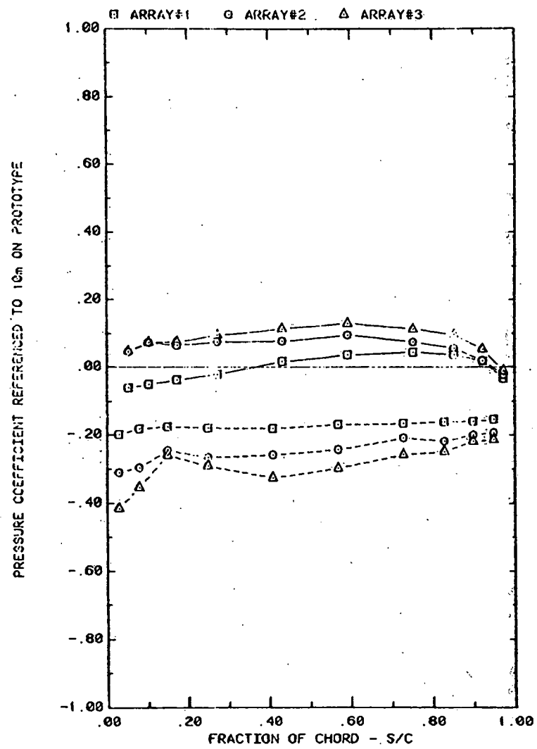
FRONT AND BACK PRESSURES 0.6" IN FROM ARRAY EDGE; X=2C, WIND=45 EFFECT OF ARRAY WITH ALPHA=145, FC=3, H=3°, D=10°, AND P=30%
