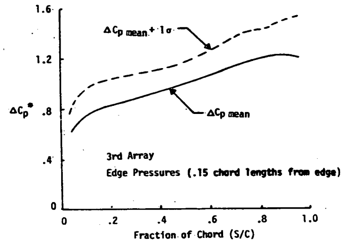
Figure 4-11b. Effect of Oblique Winds on Array Edge Pressure Distribution (No Fence, Wind from Rear)
