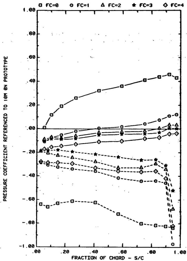
FRONT AND BACK PRESSURES 0.6° IN FROM EDGE OF ARRAY#2; WIND=45 EFFECT OF FC WITH ALPHA=35, H=3°, D=10°, P=30% AND X=2C
