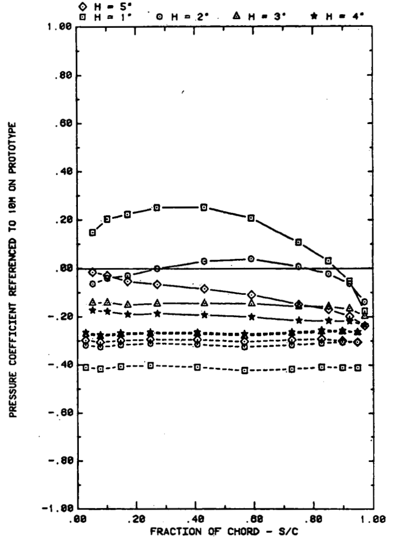
FRONT AND BACK PRESSURES ON SINGLE ARRAY, WIND = 0 EFFECT OF FENCE HEIGHT, ALPHA = 145, D = 10, P = 30%
