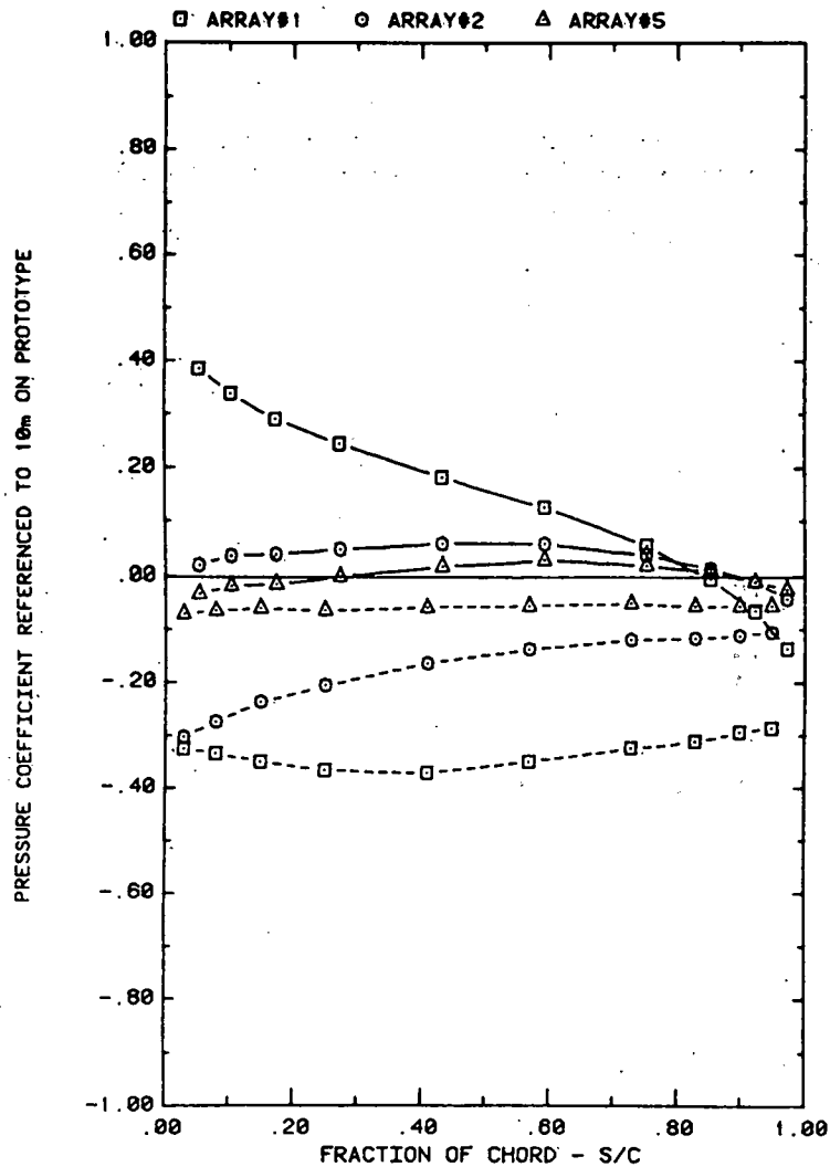
FRONT AND BACK PRESSURES ON ARRAYS IN BOUNDARY LAYER, X = 2.0c EFFECT OF ARRAY CONFIGURATION ON ATTACK ANGLE 160^\circ , H/C = 0.25
