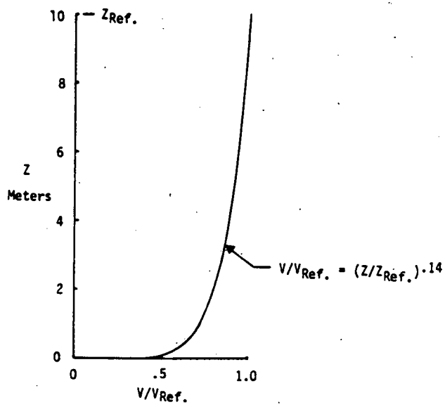
Figure 4-2. 1/7 Power Law Wind Velocity Profile
