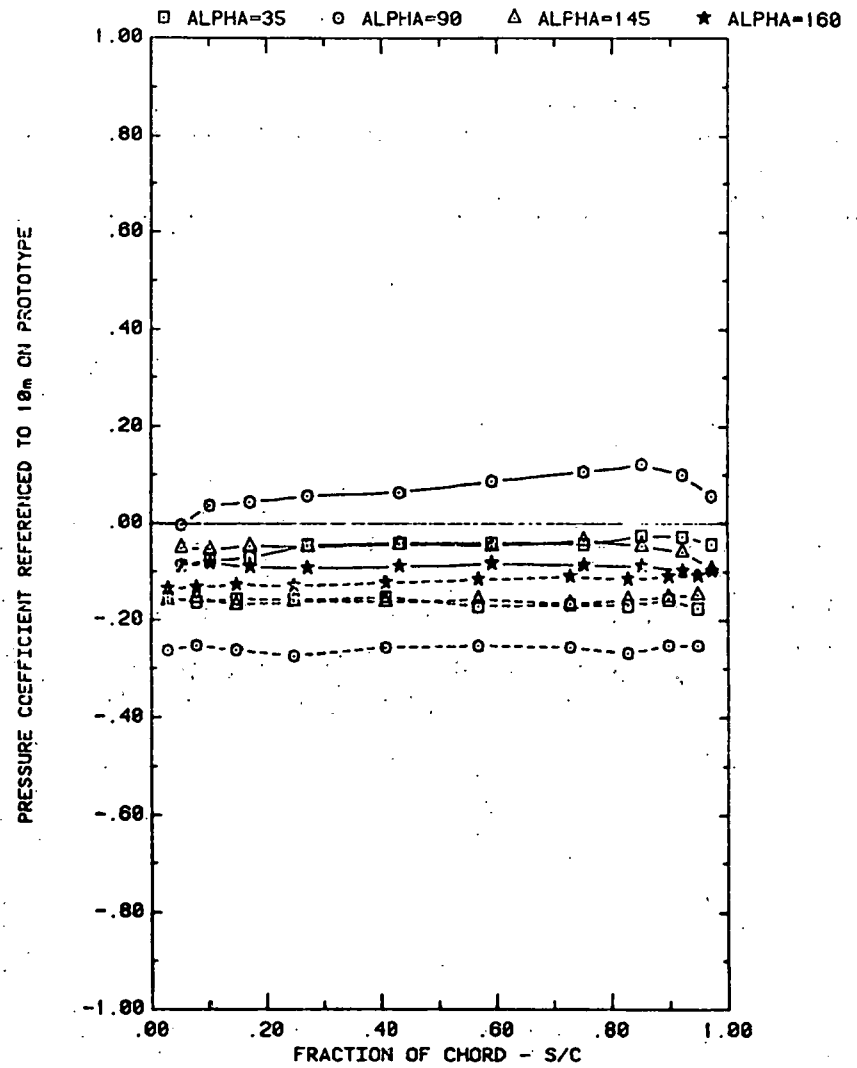
FRONT AND BACK PRESSURES ON ARRAY #1 WITH SEPARATION = 2C EFFECT OF ATTACK ANGLE WITH H=3^\circ , P=30\% , AND D=10^\circ
