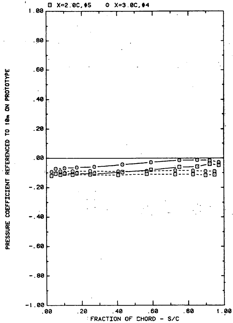
FRONT AND BACK PRESSURES ON ARRAY #4 OR #5 IN BOUNDARY LAYER EFFECT OF SEPARATION (X) ON ATTACK ANGLE 120, H/C = 0.25
