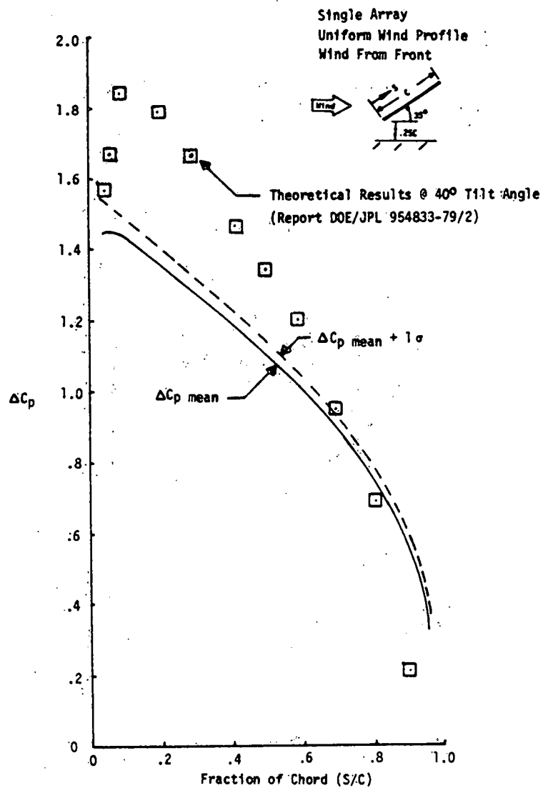
Figure 5-2b. Array Pressure Coefficient Distribution Comparison Between Wind Tunnel Test and Theoretical Methods In Close Ground Proximity (Tilt Angle = 35°)
