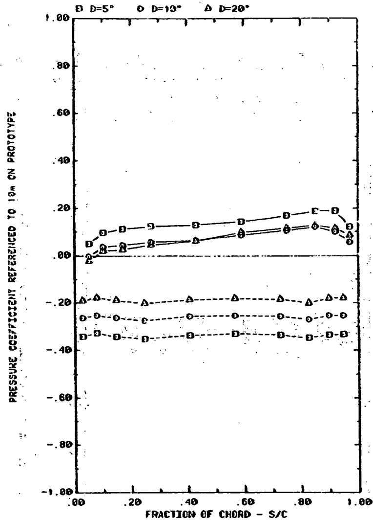
FRONT AND BACK PRESSURES ON ARRAY #1 WITH SEPARATION = 2C EFFECT OF FENCE DISTANCE WITH H=3^\circ , P=30\% , AND \alpha=90^\circ
