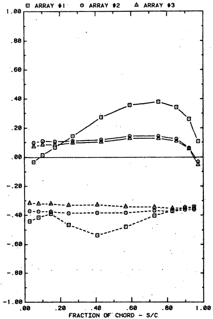
FRONT AND BACK PRESSURES ON ARRAYS #1,2&3, WIND = 45 EFFECT OF ARRAY WITH ALPHA = 145, X = 2C, FC = 4
