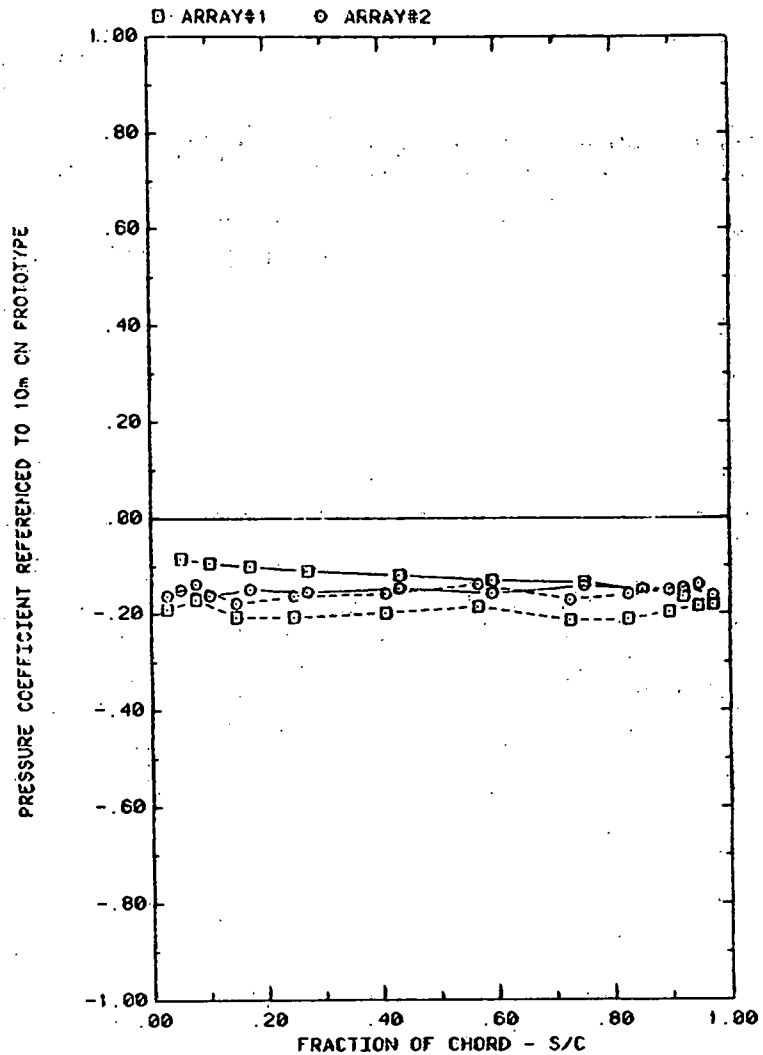
FRONT AND BACK PRESSURES ON ARRAYS #1&2 WITH SEPARATION = 2C EFFECT OF ARRAY WITH ALPHA=45, H=5", D=10", AND P=30%
