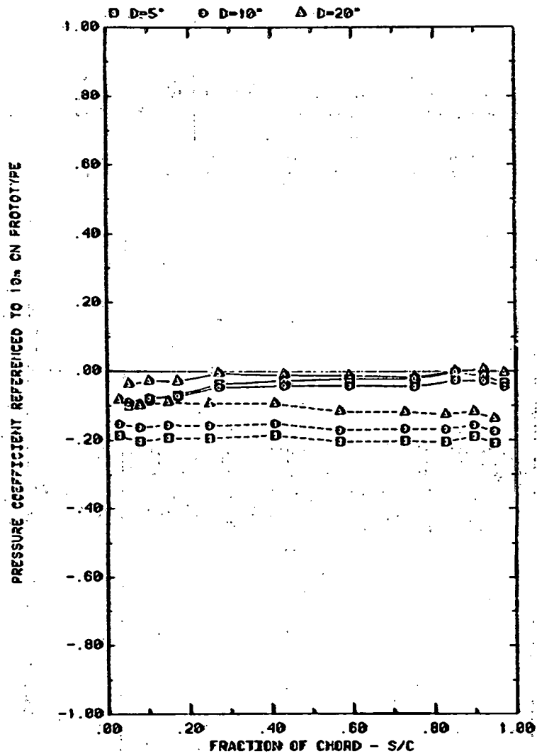
FRONT AND BACK PRESSURES ON ARRAY #1 WITH SEPARATION = 2C EFFECT OF FENCE DISTANCE WITH H=3^\circ , P=30\% , AND \alpha=35^\circ
