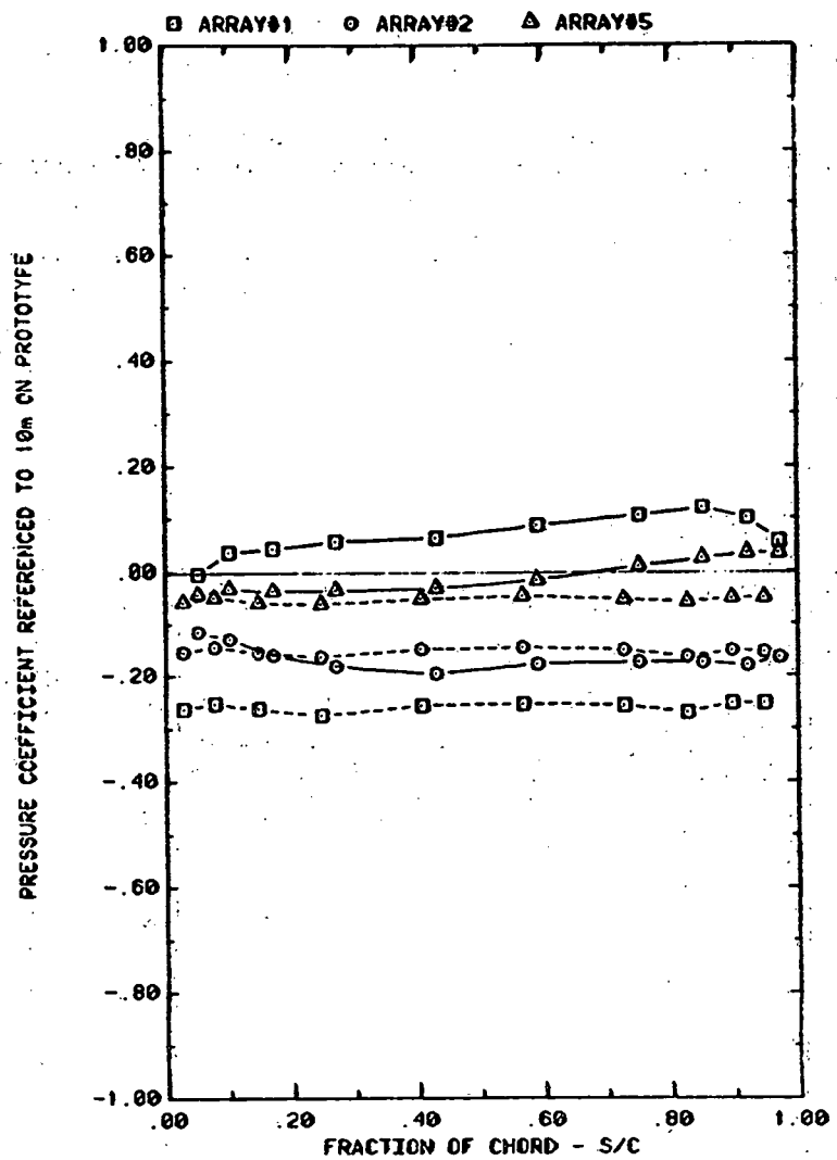
FRONT AND BACK PRESSURES ON VARIOUS ARRAYS WITH SEPARATION = 2C EFFECT OF ARRAYS WITH ATTACK ANGLE=90, H=3°, P=30%, AND D=10°
