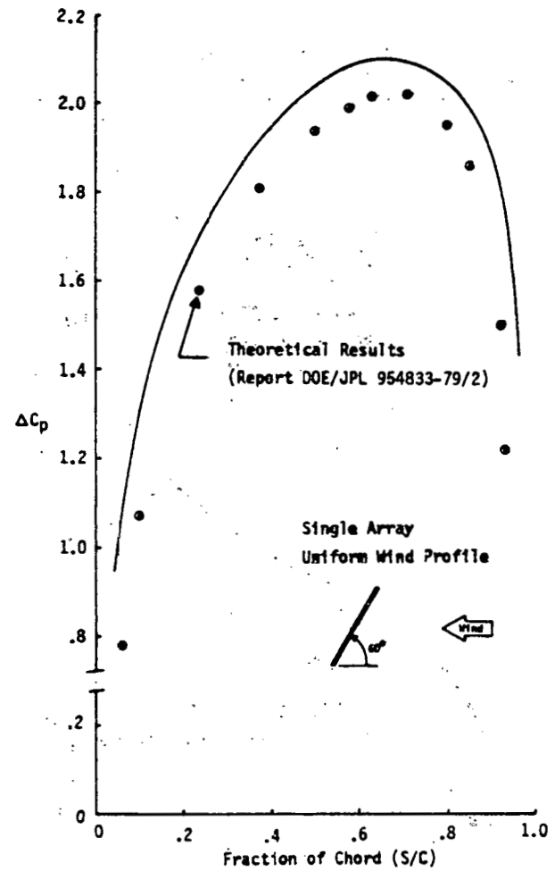
Figure 5-1. Array Pressure Coefficient Distribution Comparison Between Wind Tunnel Test and Theoretical Methods in Free Air
