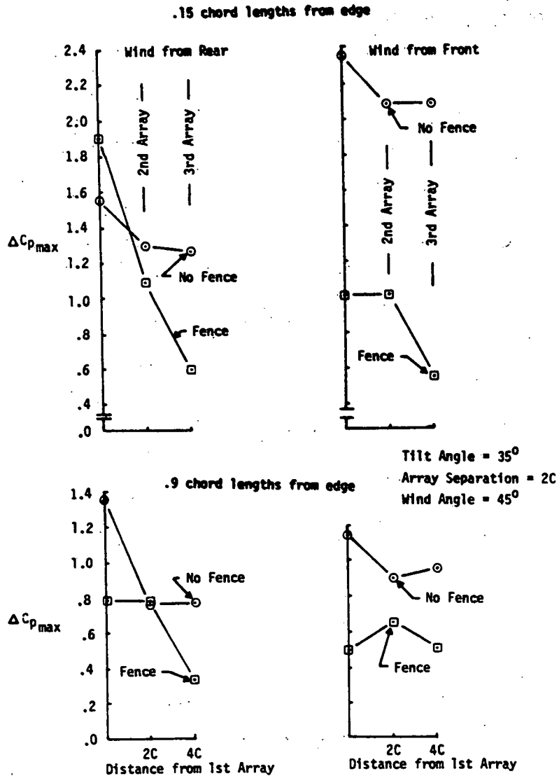
Figure 4-13. Maximum Pressure Coefficient at Array Side Edge Due to Oblique Winds
