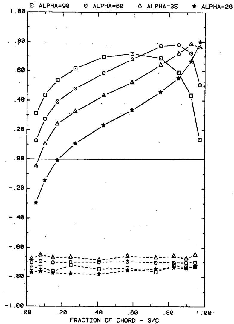
FRONT AND BACK PRESSURES ON A SINGLE ARRAY IN UNIFORM FLOW EFFECT OF ATTACK ANGLE FOR GROUND CLEARANCE, h/c = 0.25
