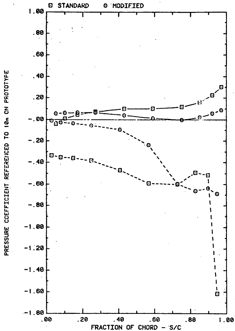
FRONT AND BACK PRESSURES ON ARRAY #1 WITH X=2C , AND WIND=45 EFFECT OF TAP LOCATION; ALPHA=35, H=3°, D=10°, FC=1, AND P=30%
