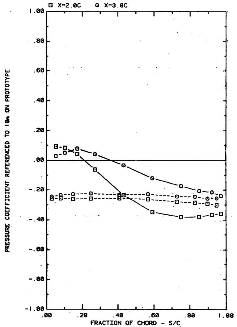
FRONT AND BACK PRESSURES ON ARRAY #2 IN BOUNDARY LAYER EFFECT OF SEPARATION (X) ON ATTACK ANGLE 60, H/C = 0.25
