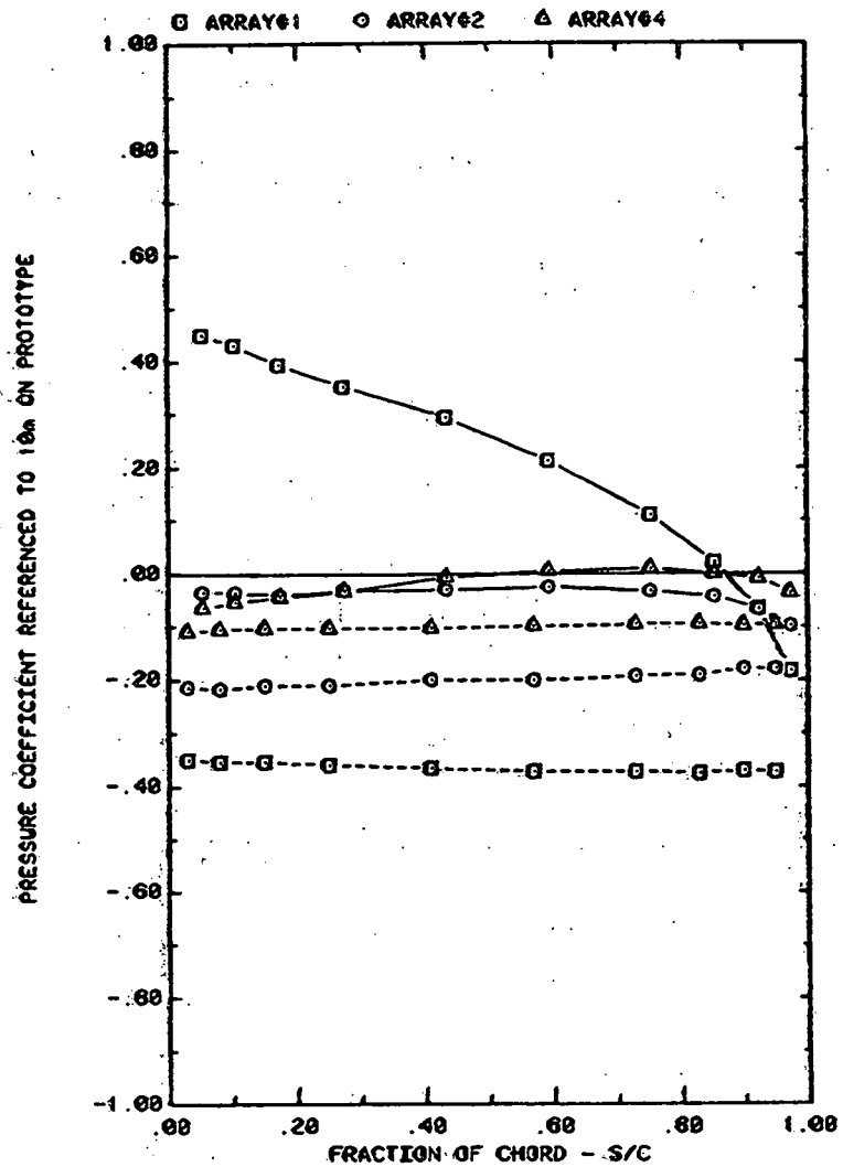
FRONT AND BACK PRESSURES ON ARRAYS IN BOUNDARY LAYER, \alpha = 3.00 EFFECT OF ARRAY CONFIGURATION ON ATTACK ANGLE 145^\circ , H/C = 0.25
