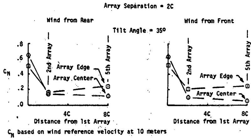
Figure 4-9. Comparison Between Array Edge and Center of Span Normal Force Coefficients for Head-On and Rearward Winds (No Fence)
