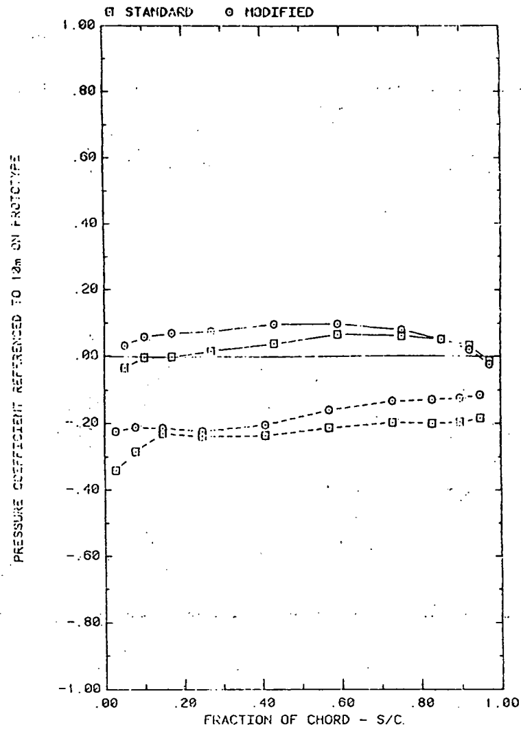
FRONT AND BACK PRESSURES ON ARRAY #1 WITH X=2C , AND WIND=45 EFFECT OF TAP LOCATION; \alpha=145 , H=3'' , D=10'' , FC=2 , AND P=30\%
