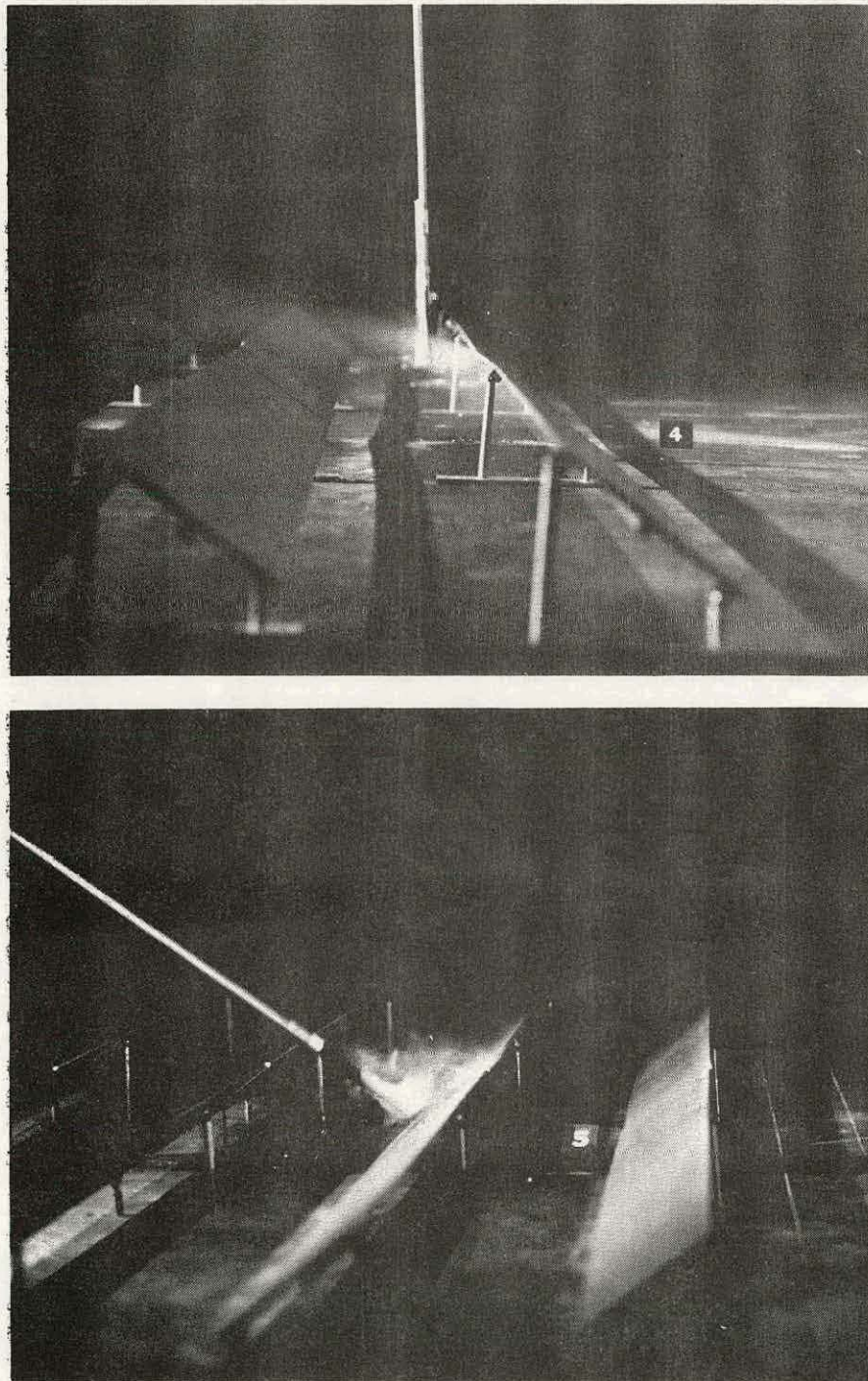
Figure 31c. Flow Visualization for an Array Field, WD = 0^\circ
