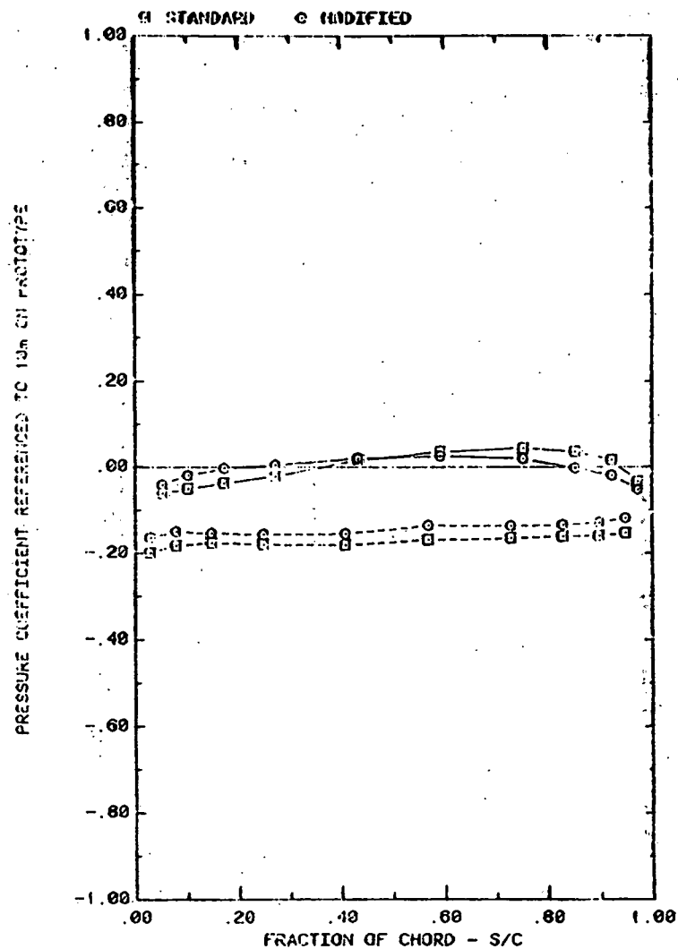
FRONT AND BACK PRESSURES ON ARRAY #1 WITH X=2C , AND WIND=45 EFFECT OF TAP LOCATION; \alpha=145 , H=3^\circ , D=10^\circ , FC=3 , AND P=30\%
