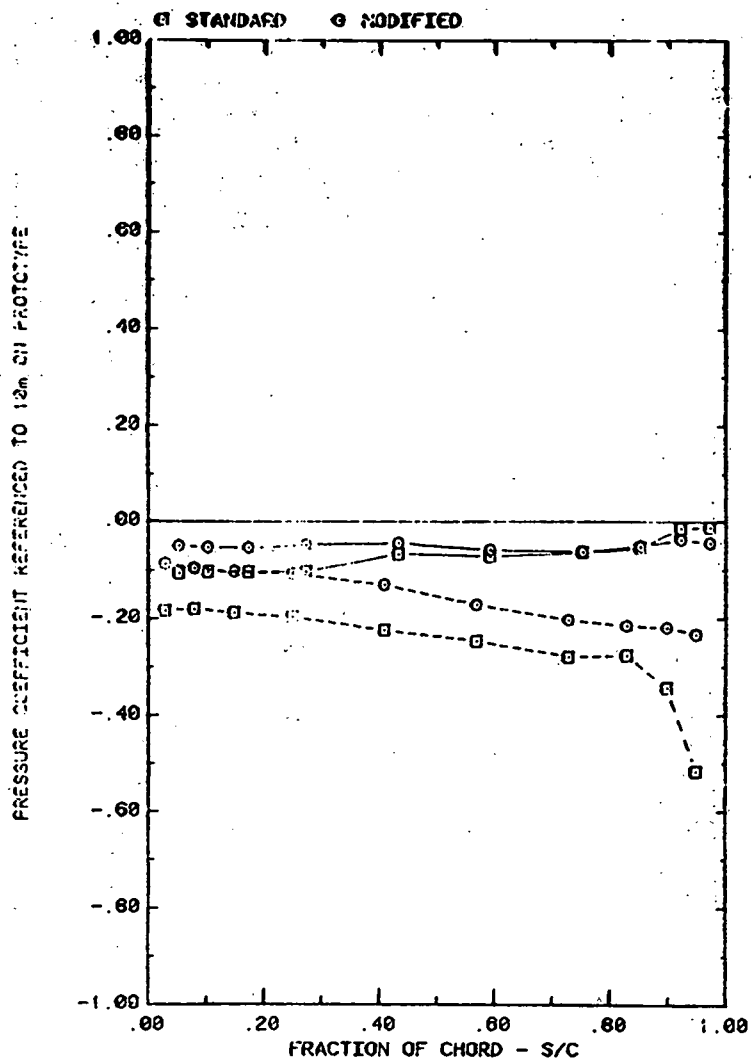
FRONT AND BACK PRESSURES ON ARRAY #1 WITH X=2C , AND WIND=45 EFFECT OF TAP LOCATION; \alpha=35 , H=3^\circ , D=10^\circ , FC=3 , AND P=30\%
