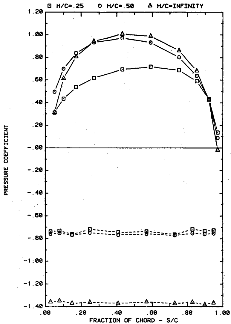
FRONT AND BACK PRESSURES ON A SINGLE ARRAY IN UNIFORM FLOW EFFECT OF GROUND CLEARANCE FOR ATTACK ANGLE, \alpha = 90^\circ
