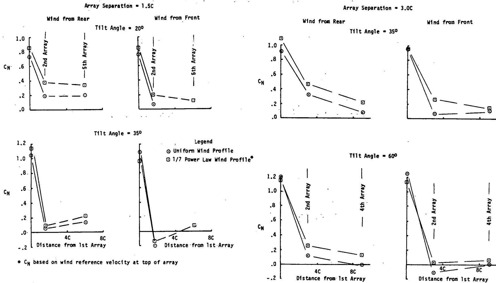
Figure 4-15. Array Normal Force Coefficient Comparison Between Uniform and Boundary Layer Wind Profiles.
