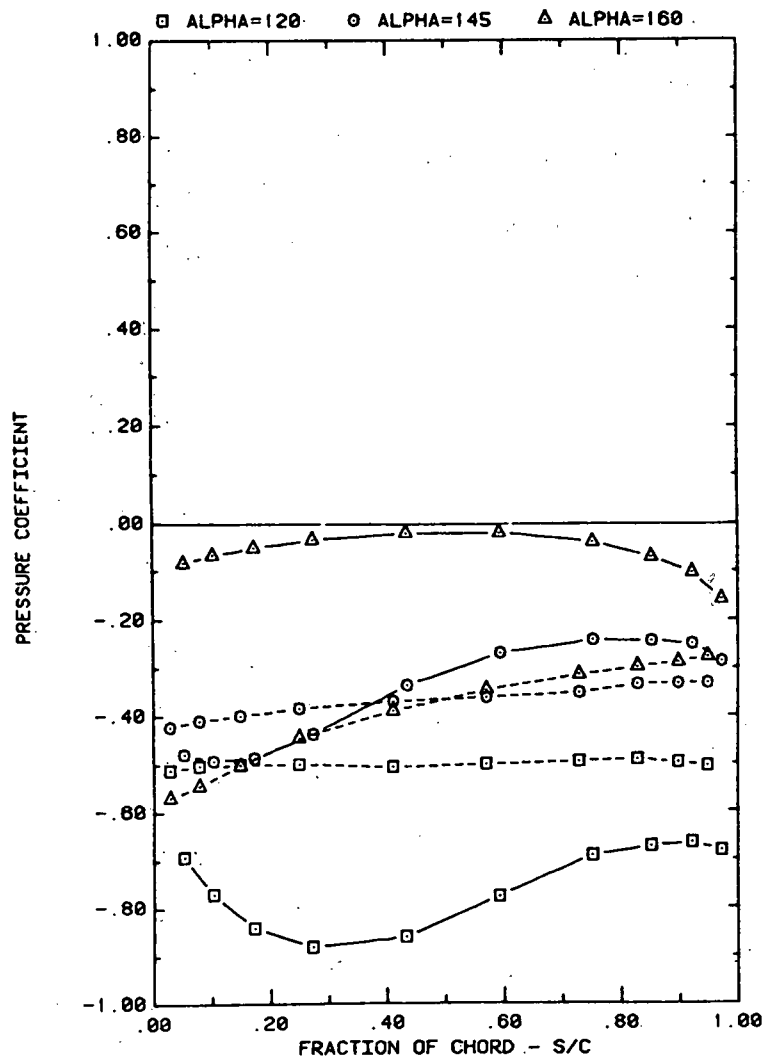
FRONT AND BACK PRESSURES ON ARRAY #2 IN UNIFORM FLOW. EFFECT OF ATTACK ANGLE FOR SPACING = 2C
