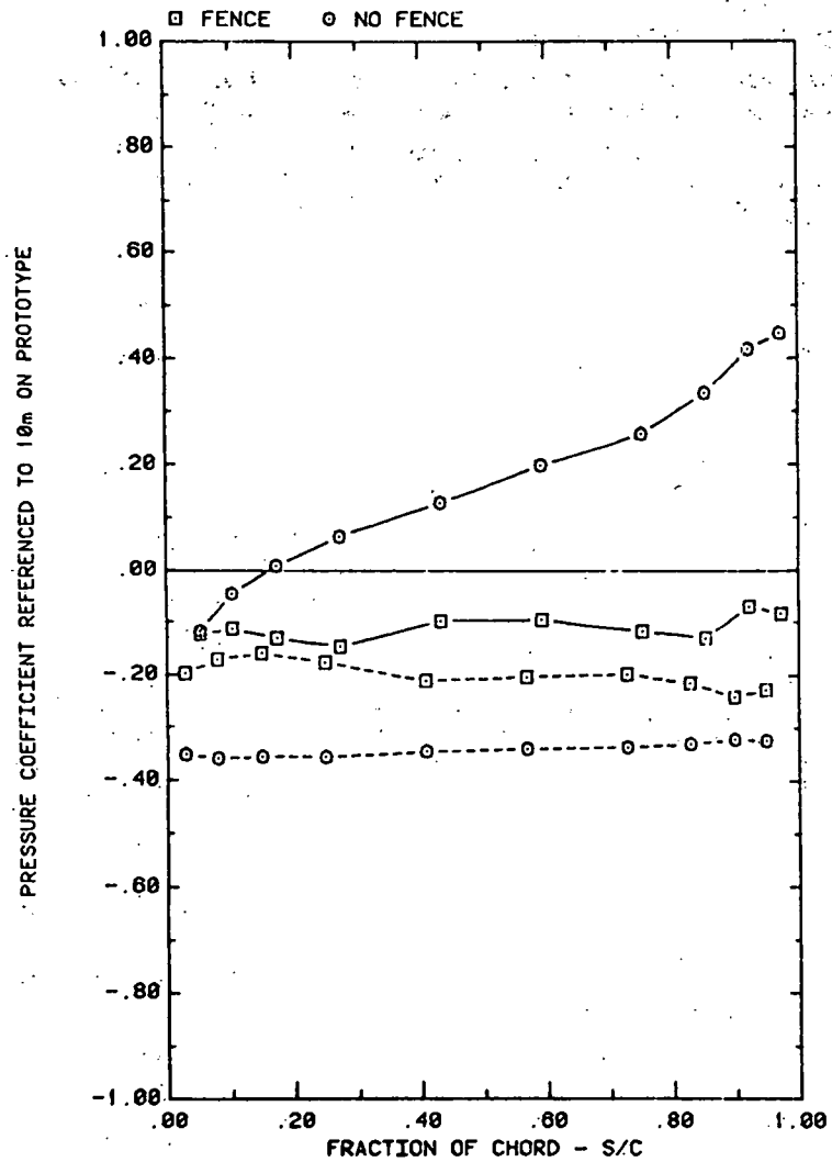
FRONT AND BACK PRESSURES ON ARRAY #1 WITH X=2C , AND WIND=0 EFFECT OF FENCE ON ARRAY EDGE; \alpha=35^\circ , H=3^\circ , D=10^\circ , AND P=30\%
