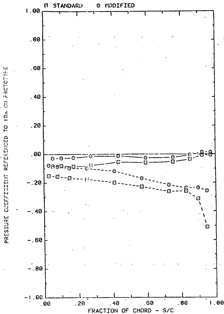
FRONT AND BACK PRESSURES ON ARRAY #1 WITH X=2C , AND WIND=45 EFFECT OF TAP LOCATION; \alpha=35 , H=3'' , D=10'' , FC=2 , AND P=30\%
