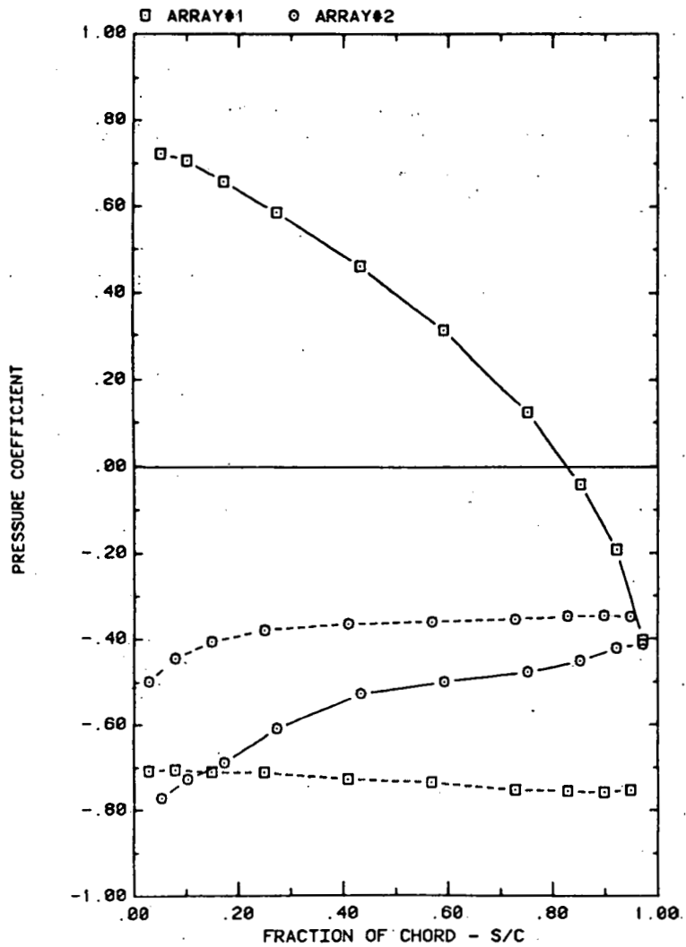
FRONT AND BACK PRESSURES ON VARIOUS ARRAYS FOR SEPARATION = 1.5C EFFECT OF ARRAY CONFIGURATION FOR ATTACK ANGLE, \alpha = 145
