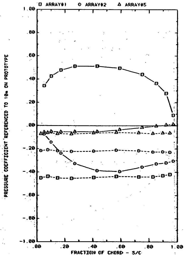
FRONT AND BACK PRESSURES ON ARRAYS IN BOUNDARY LAYER, \alpha = 90^\circ EFFECT OF ARRAY CONFIGURATION ON ATTACK ANGLE 90^\circ , H/C = 0.25
