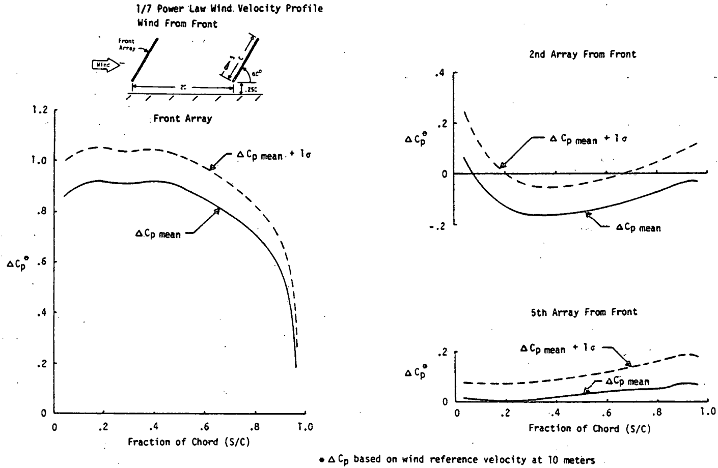
Figure 4-3e. Array Chordwise Pressure Coefficient Distribution in Boundary Layer Wind (Tilt Angle = 60^\circ , Wind from Front)
