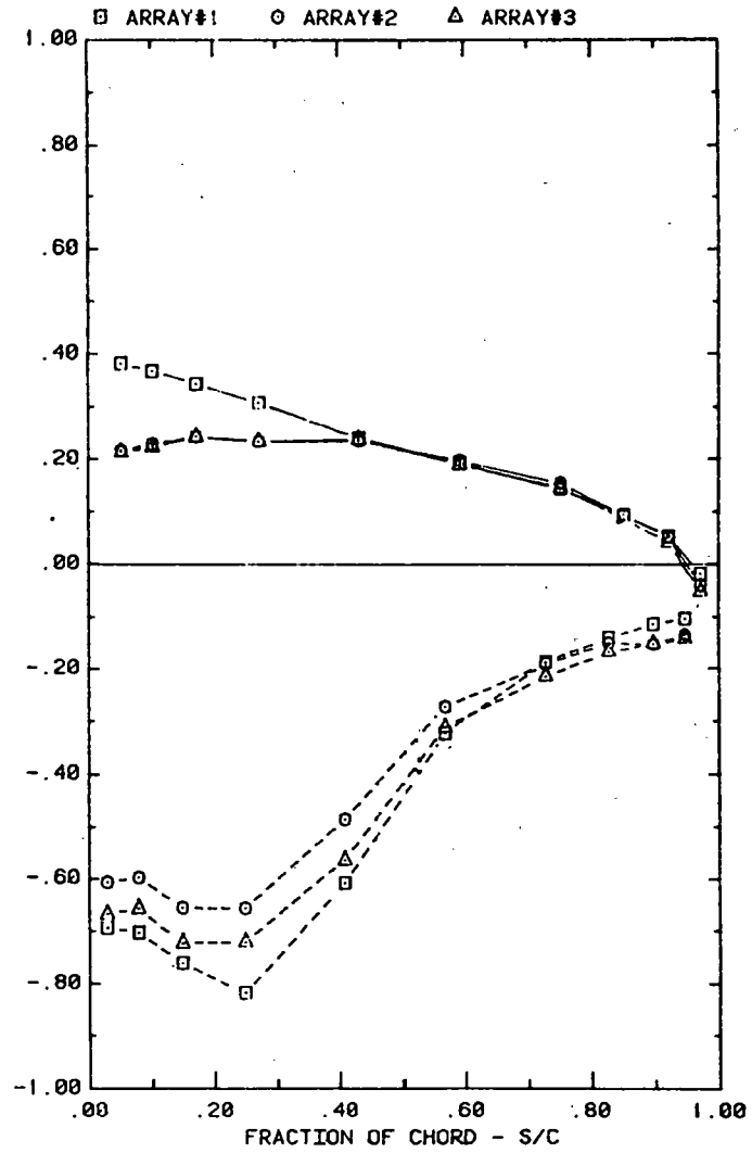
FRONT AND BACK PRESSURES 3.6° IN FROM ARRAY EDGE; X=2C ; WIND=45 EFFECT OF ARRAY WITH \alpha=145 , FC=0 , H=3^\circ , D=10^\circ , AND P=30\%
