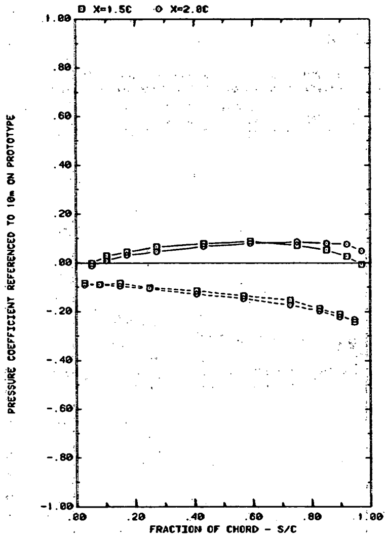
FRONT AND BACK PRESSURES ON ARRAY #5 IN BOUNDARY LAYER EFFECT OF SEPARATION (X) ON ATTACK ANGLE 20; H/C = 0.25
