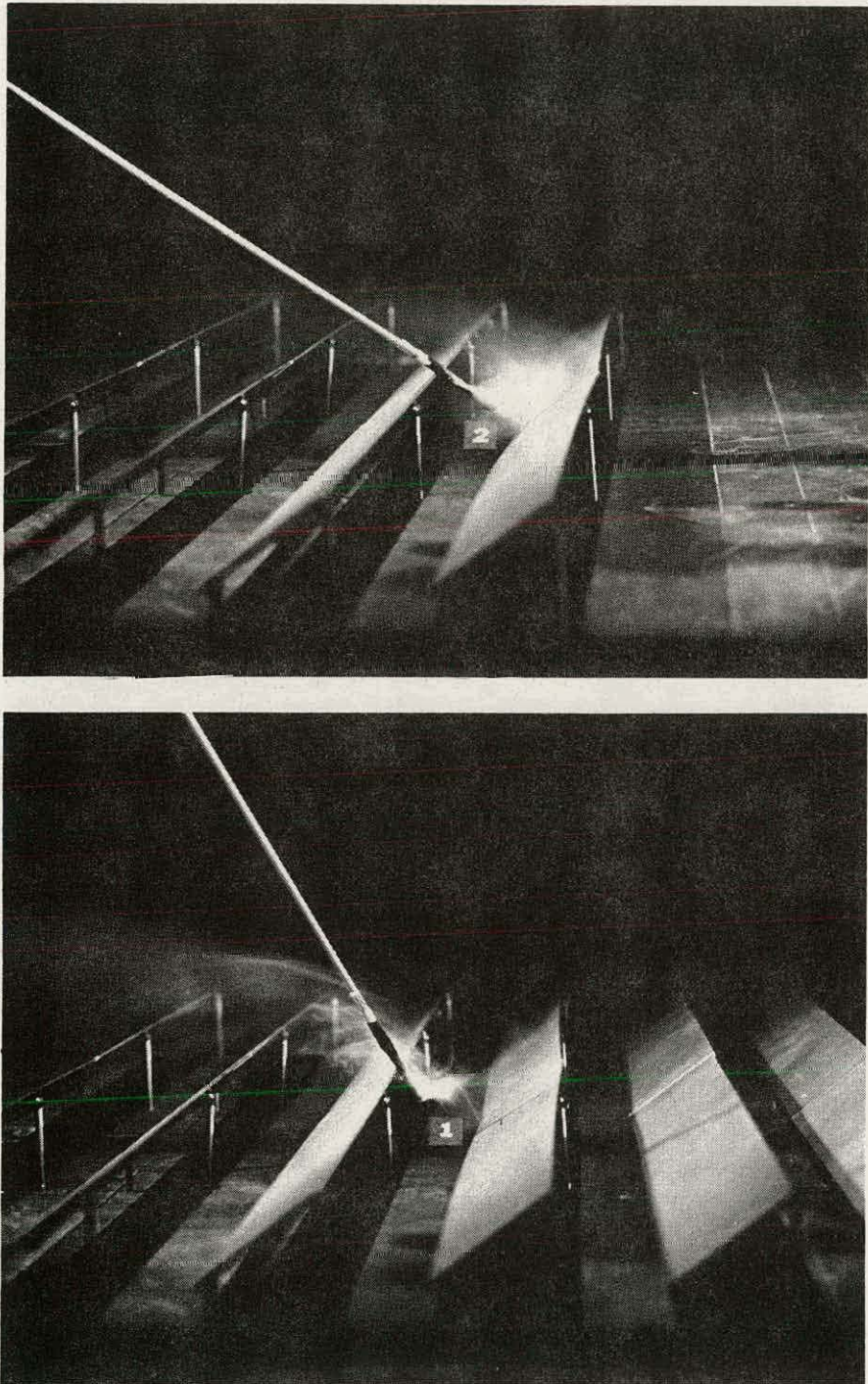
Figure 31b. Flow Visualization for an Array Field, WD = 0^\circ
