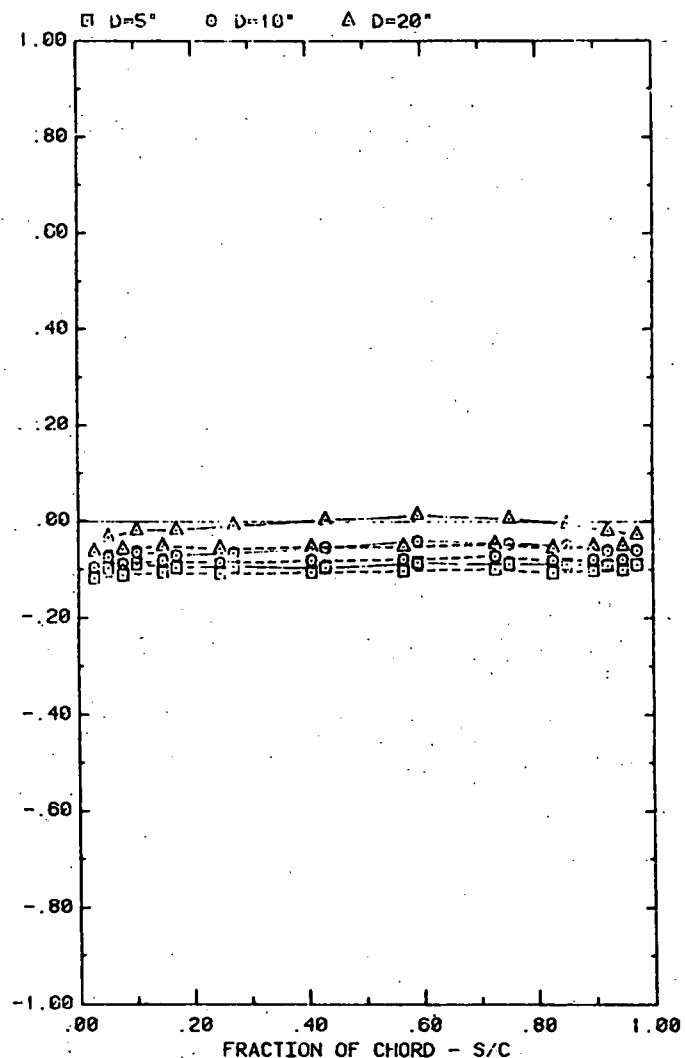
FRONT AND BACK PRESSURES ON ARRAY #2 WITH SEPARATION = 2C EFFECT OF FENCE DISTANCE WITH H=3", P=30%, AND ALPHA=160
