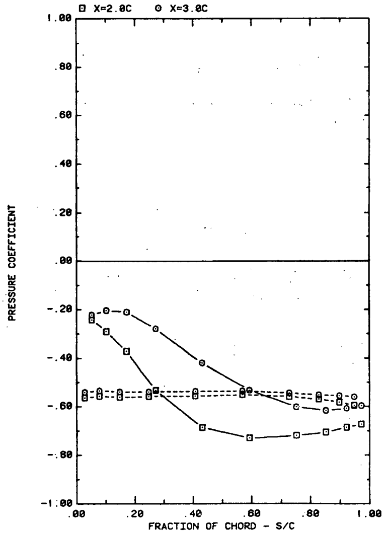
FRONT AND BACK PRESSURES ON ARRAY #2 IN UNIFORM FLOW EFFECT OF SEPARATION (X) ON ATTACK ANGLE 60, H/C = 0.25
