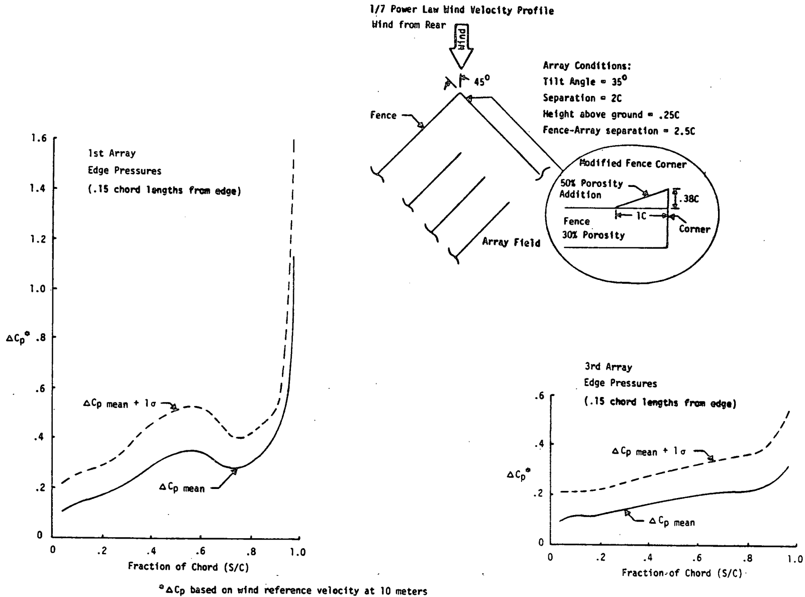
Figure 4-11h. Effect of Oblique Winds on Array Edge Pressure Distribution (Modified Fence Corner, Wind from Rear)
