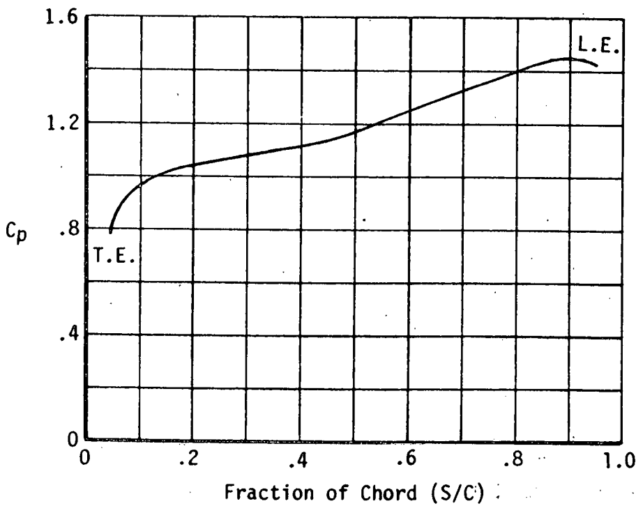
Figure 7-3a. Steady State Wind Pressure Coefficient and Normal Force Coefficient Guidelines for Edge Arrays in an Array Field (No Fence)
