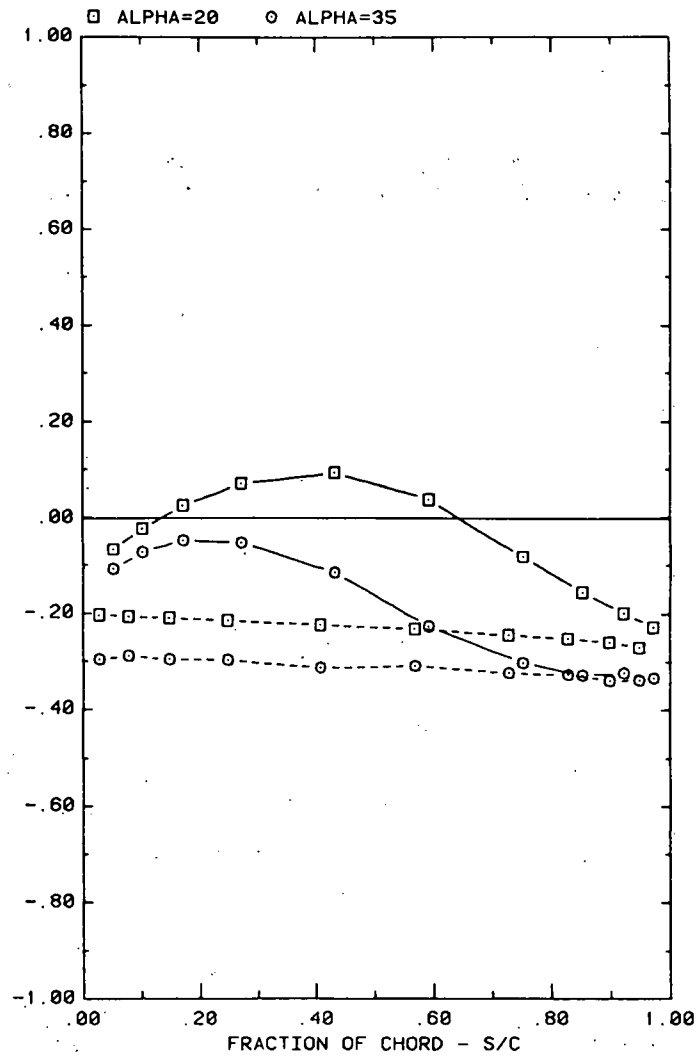
FRONT AND BACK PRESSURES ON ARRAY #5 IN UNIFORM FLOW EFFECT OF ATTACK ANGLE FOR SPACING = 1.5C
