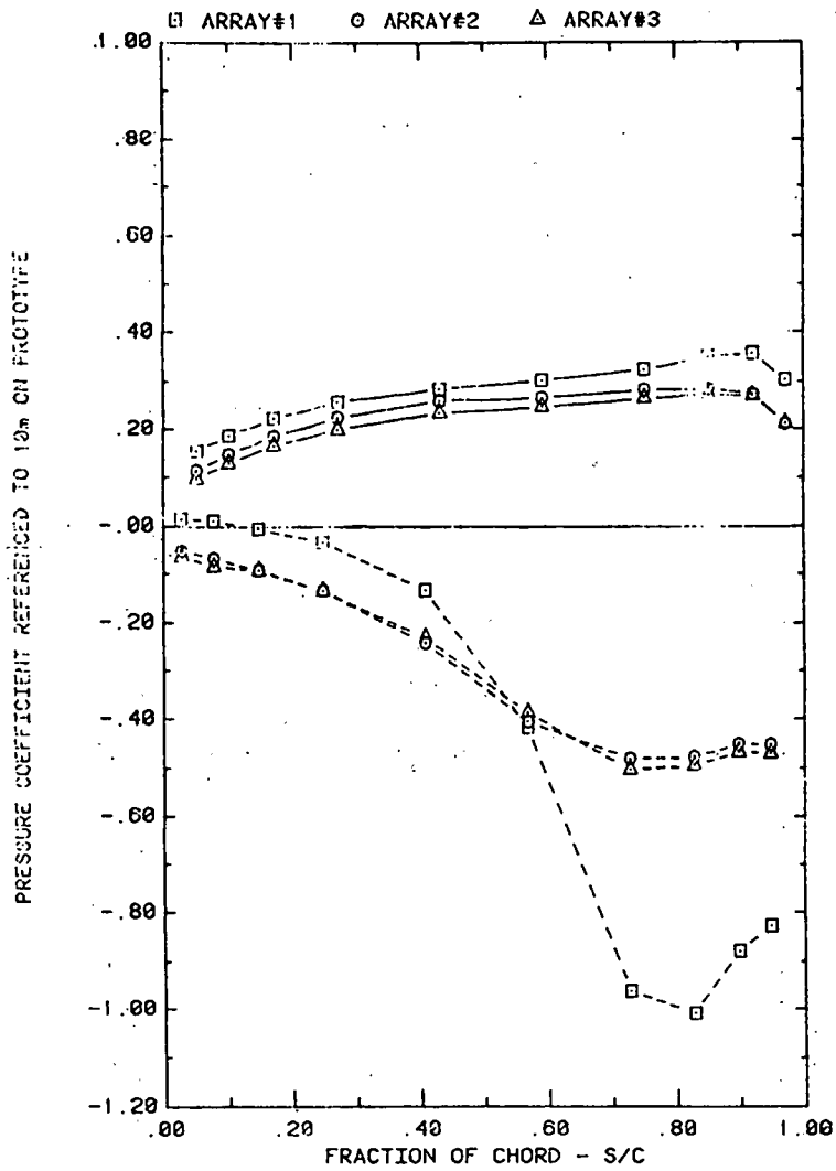
FRONT AND BACK PRESSURES 3.6° IN FROM ARRAY EDGE; X=2C ; WIND=45 EFFECT OF ARRAY WITH \alpha=35 , FC=0 , H=3^\circ , D=10^\circ , AND P=30\%
