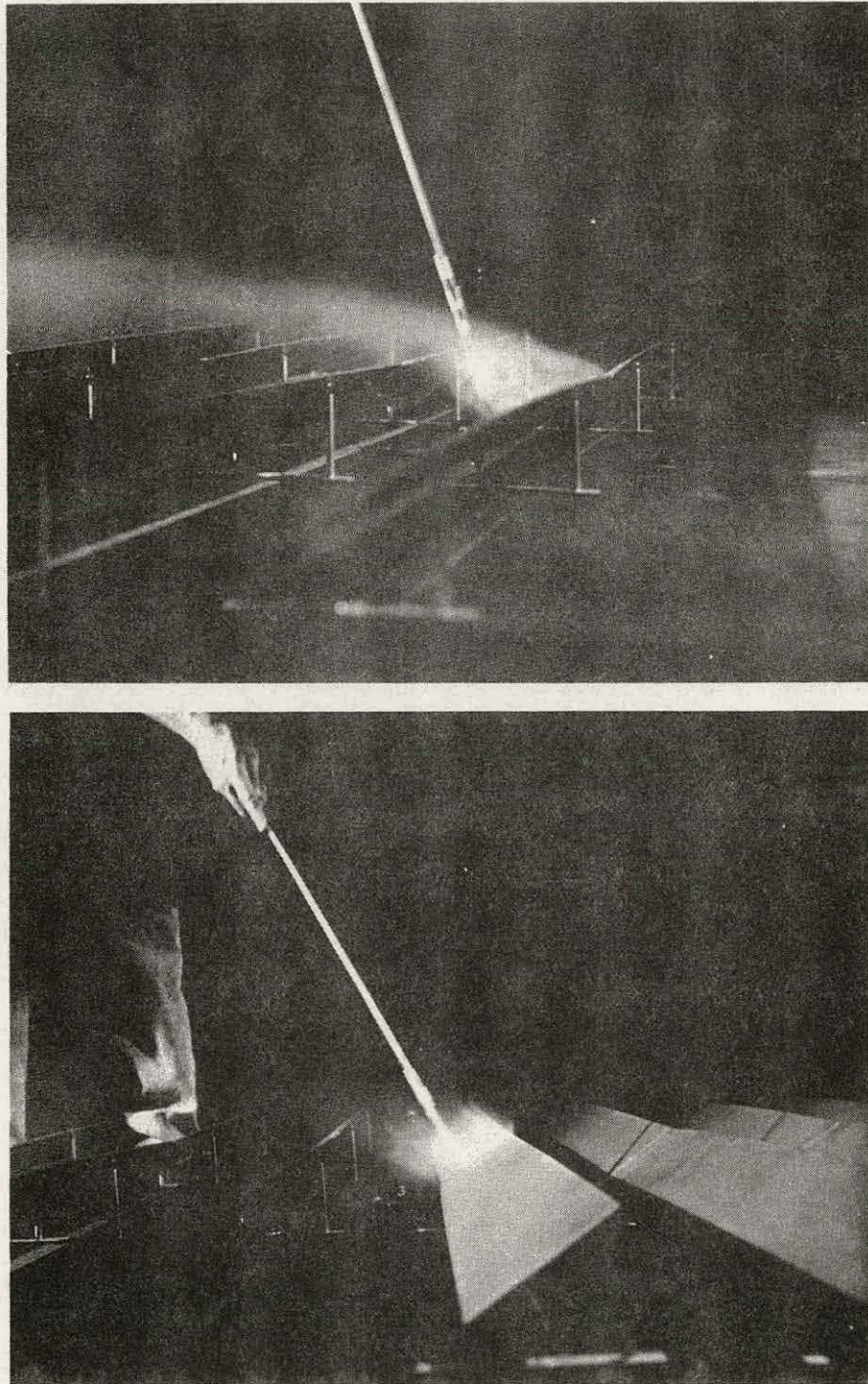
Figure 31a. Flow Visualization for an Array Field, WD = 0^\circ
