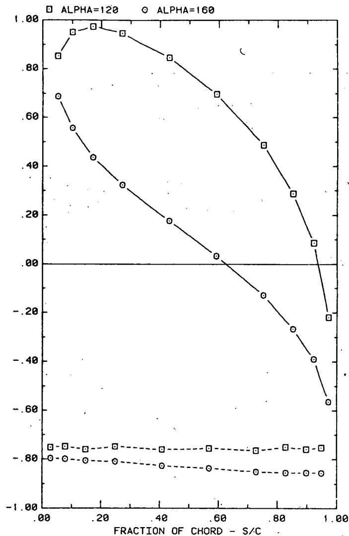
FRONT AND BACK PRESSURES ON A SINGLE ARRAY IN UNIFORM FLOW EFFECT ON ATTACK ANGLE FOR GROUND CLEARANCE, H/C = 0.50
