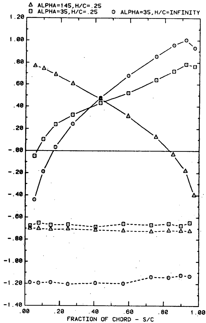
FRONT AND BACK PRESSURES ON A SINGLE ARRAY IN UNIFORM FLOW EFFECT OF GROUND CLEARANCE FOR ATTACK ANGLES
