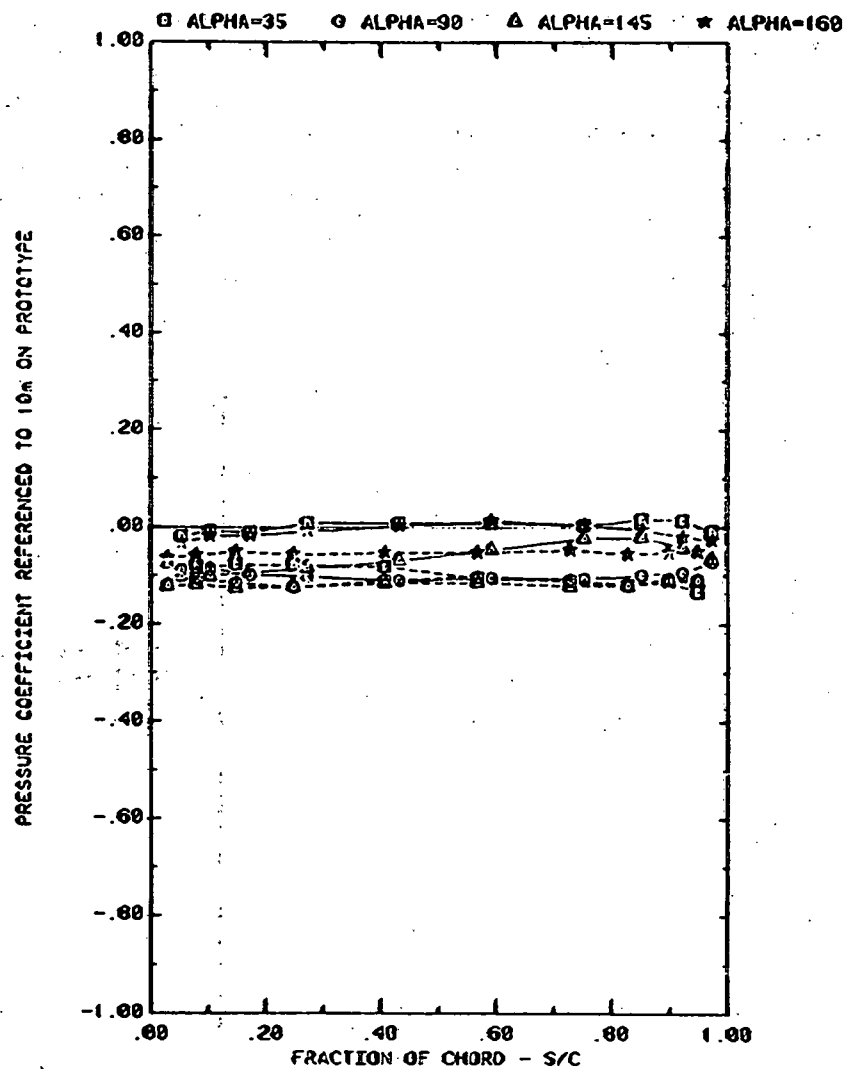
FRONT AND BACK PRESSURES ON ARRAY #2 WITH SEPARATION = 2C EFFECT OF ATTACK ANGLE WITH H=3", P=30%, AND D=20"
