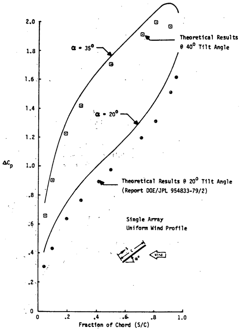
Figure 5-1. Array Pressure Coefficient Distribution Comparison Between Wind Tunnel Test and Theoretical Methods in Free Air
