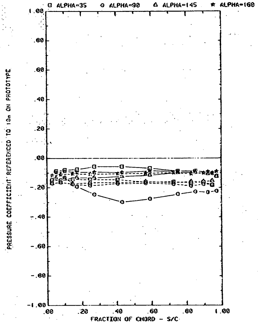
FRONT AND BACK PRESSURES ON ARRAY #2 WITH SEPARATION = 2C EFFECT OF ATTACK ANGLE WITH H=3^\circ , P=30\% , AND D=5^\circ
