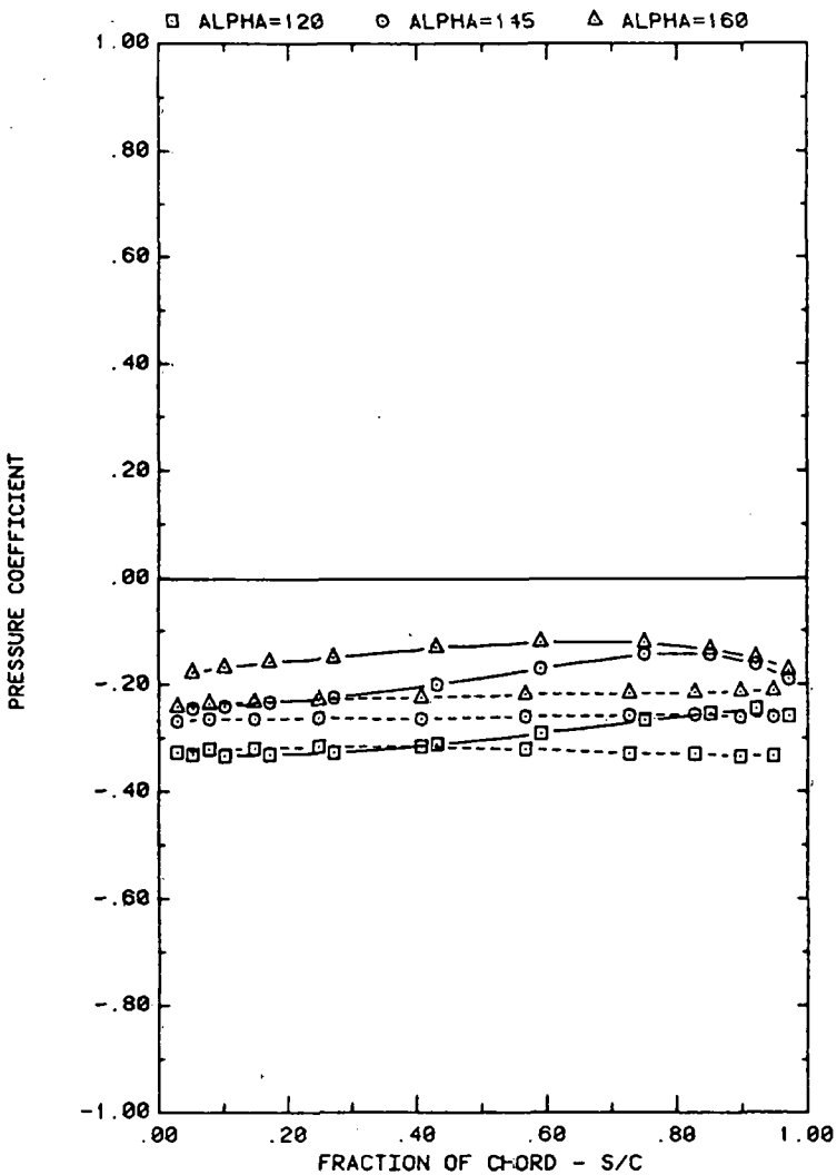
FRONT AND BACK PRESSURES ON ARRAY #5 IN UNIFORM FLOW EFFECT OF ATTACK ANGLE FOR SPACING = 2C
