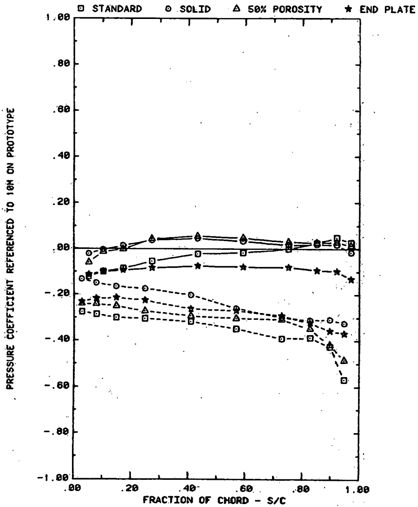
FRONT AND BACK PRESSURES ON ARRAYS; X = 2C , WIND = 45 EFFECT OF EXTENSIONS; ARRAY = 3, ALPHA = 35, FC = 1
