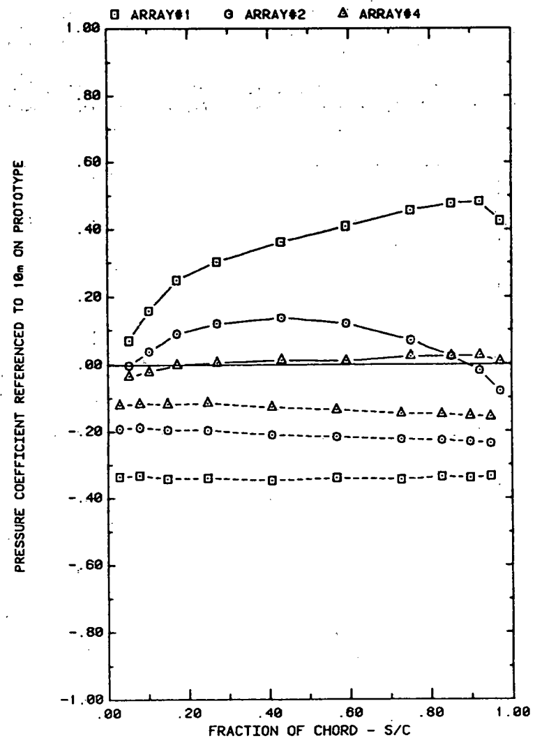
FRONT AND BACK PRESSURES ON ARRAYS IN BOUNDARY LAYER, X = 3.0c EFFECT OF ARRAY CONFIGURATION ON ATTACK ANGLE 35^\circ , H/C = 0.25
