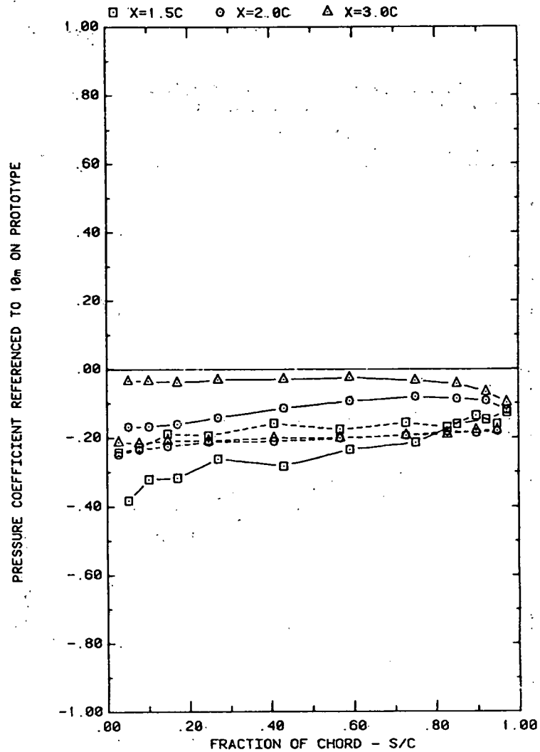
FRONT AND BACK PRESSURES ON ARRAY #2 IN BOUNDARY LAYER EFFECT OF SEPARATION (X) ON ATTACK ANGLE 145, H/C = 0.25
