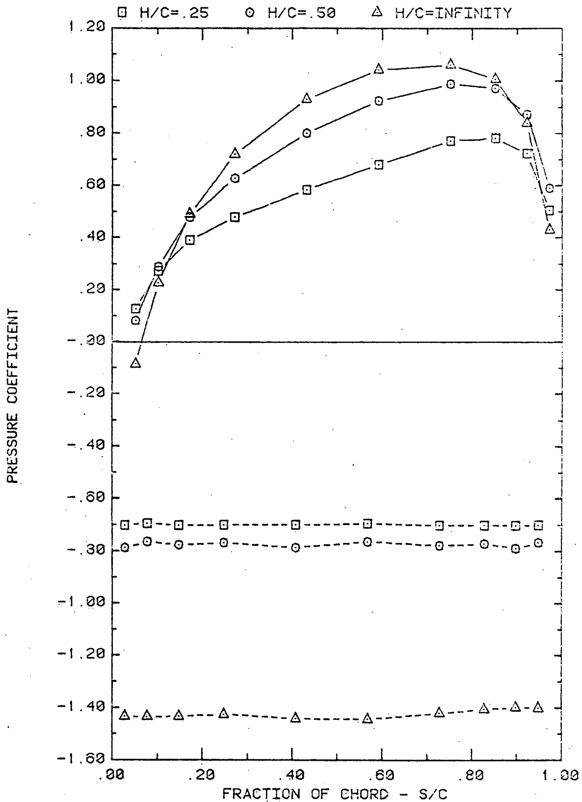
FRONT AND BACK PRESSURES ON A SINGLE ARRAY IN UNIFORM FLOW. EFFECT OF GROUND CLEARANCE FOR ATTACK ANGLE, \alpha = 60^\circ
