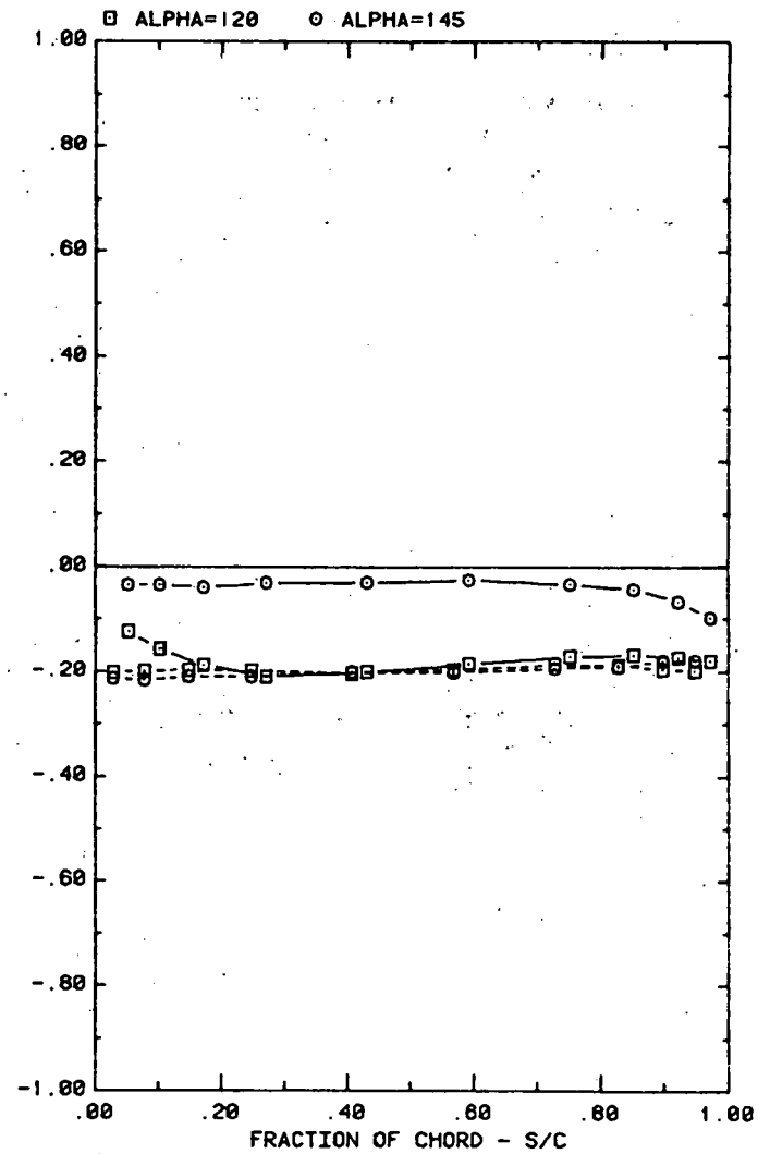
FRONT AND BACK PRESSURES ON ARRAY #2 IN BOUNDARY LAYER EFFECT OF ATTACK ANGLE FOR SPACING = 3C
