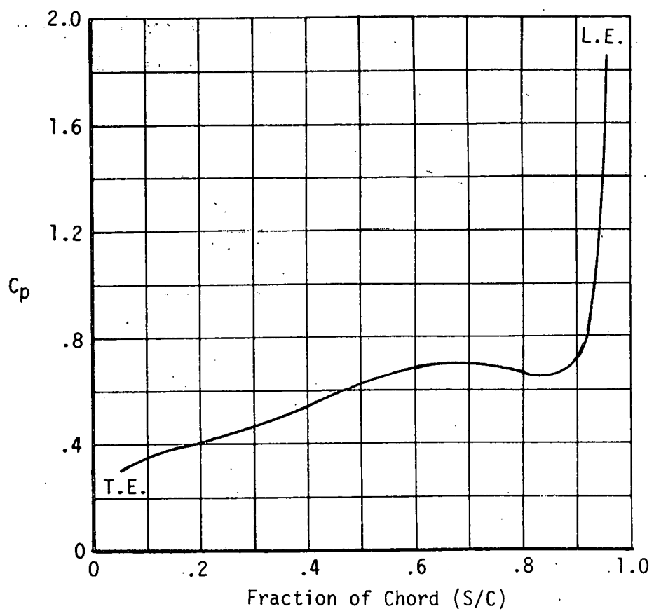
Figure 7-3b. Steady State Wind Pressure Coefficient and Normal Force Coefficient Guidelines for Edge Arrays in an Array Field (Fence)
