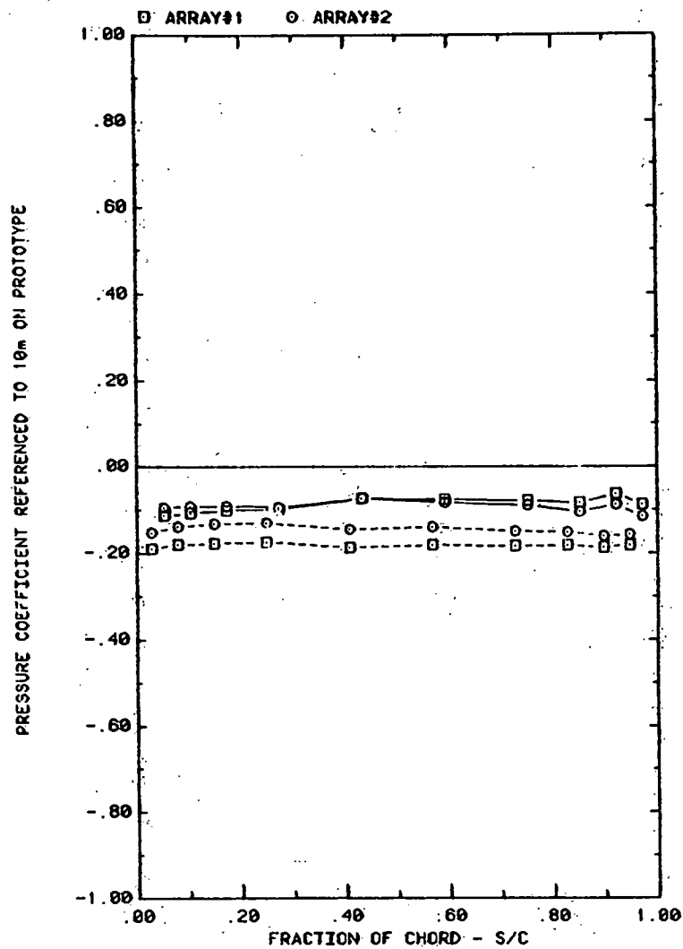
FRONT AND BACK PRESSURES ON ARRAYS #1&#2 WITH SEPARATION = 2C EFFECT OF ARRAY WITH \alpha=35^\circ , H=4^\circ , D=10^\circ , AND P=30\%
