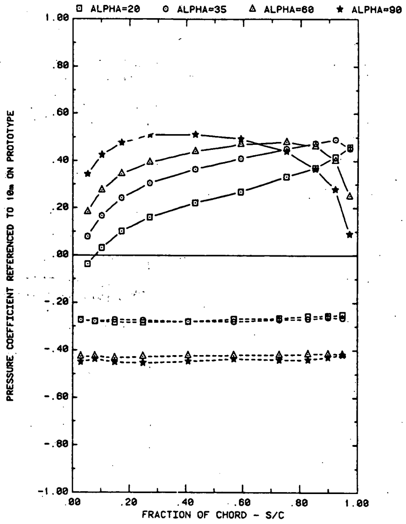
FRONT AND BACK PRESSURES ON ARRAY #1 IN BOUNDARY LAYER EFFECT OF ATTACK ANGLE FOR SPACING = 2C
