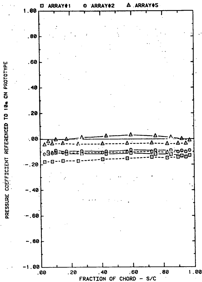
FRONT AND BACK PRESSURES ON VARIOUS ARRAYS WITH SEPARATION = 2C EFFECT OF ARRAYS WITH ATTACK ANGLE=160, H=3°, P=30%, AND D=5°
