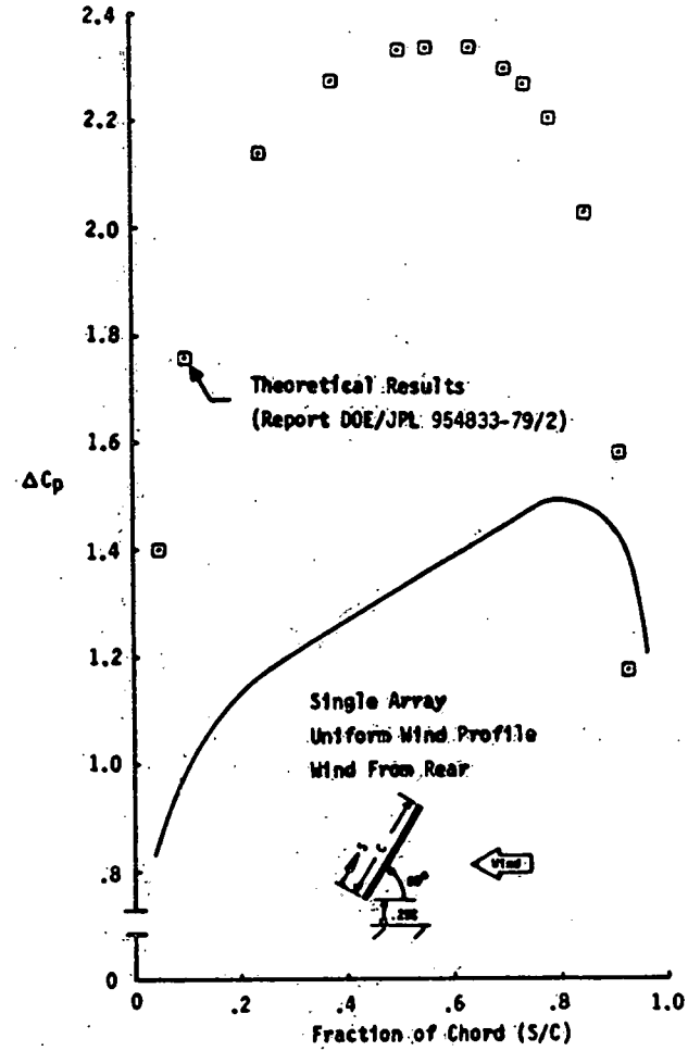
Figure 5-2c. Array Pressure Coefficient Distribution Comparison Between Wind Tunnel Test and Theoretical Methods in Close Ground Proximity (Tilt Angle = 60°)
