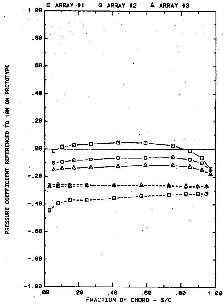
FRONT AND BACK PRESSURES ON ARRAYS #1, 2 & 3 \END PLATE EFFECT OF ARRAY WITH ALPHA = 145, WIND = 45, X = 2C, FC = 1
