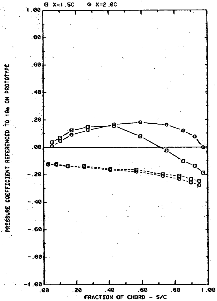
FRONT AND BACK PRESSURES ON ARRAY #2 IN BOUNDARY LAYER EFFECT OF SEPARATION (X) ON ATTACK ANGLE 20, H/C = 0.25
