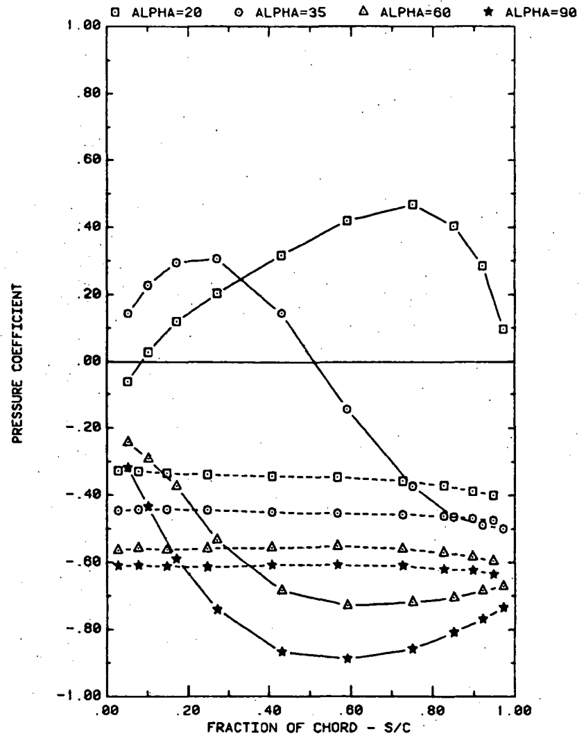
FRONT AND BACK PRESSURES ON ARRAY #2 IN UNIFORM FLOW EFFECT OF ATTACK ANGLE FOR SPACING = 2C
