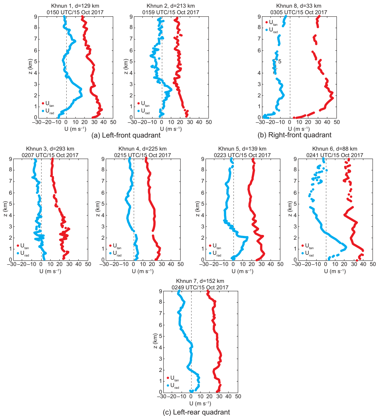
Fig. 5. Wind profiles of a weakening TC at a rate of 5 \text{ kt } 6 \text{ h}^{-1} , namely Khanun on October 15, 2017. Nomenclature as in Figure 2.
