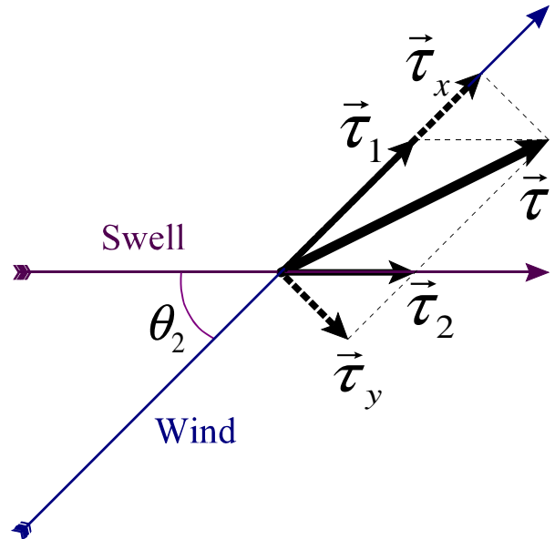
Figure 1. Decomposition of the stress vector, \vec{\tau} , into \vec{\tau}_x and \vec{\tau}_y in a wind-associated coordinate system, and into \vec{\tau}_1 and \vec{\tau}_2 in a wind-swell coordinate system.
