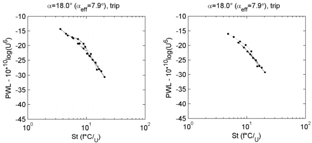
Figure 12. Normalized inflow-turbulence noise spectra for tripped S822 (left) and S834 (right) airfoils (array on suction side). ___ 22.4 m/s; __ 32.0 m/s; ... 47.9 m/s; _ 63.9 m/s.
