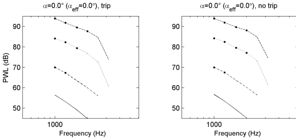
Figure 10. Leading edge noise spectra for S822 airfoil (array on suction side). \text{---} 22.4 m/s; \text{- -} 32.0 m/s; \text{...} 47.9 m/s; \text{- . -} 63.9 m/s. Note that the levels are much higher than the trailing edge noise spectra shown in Figure 7.
