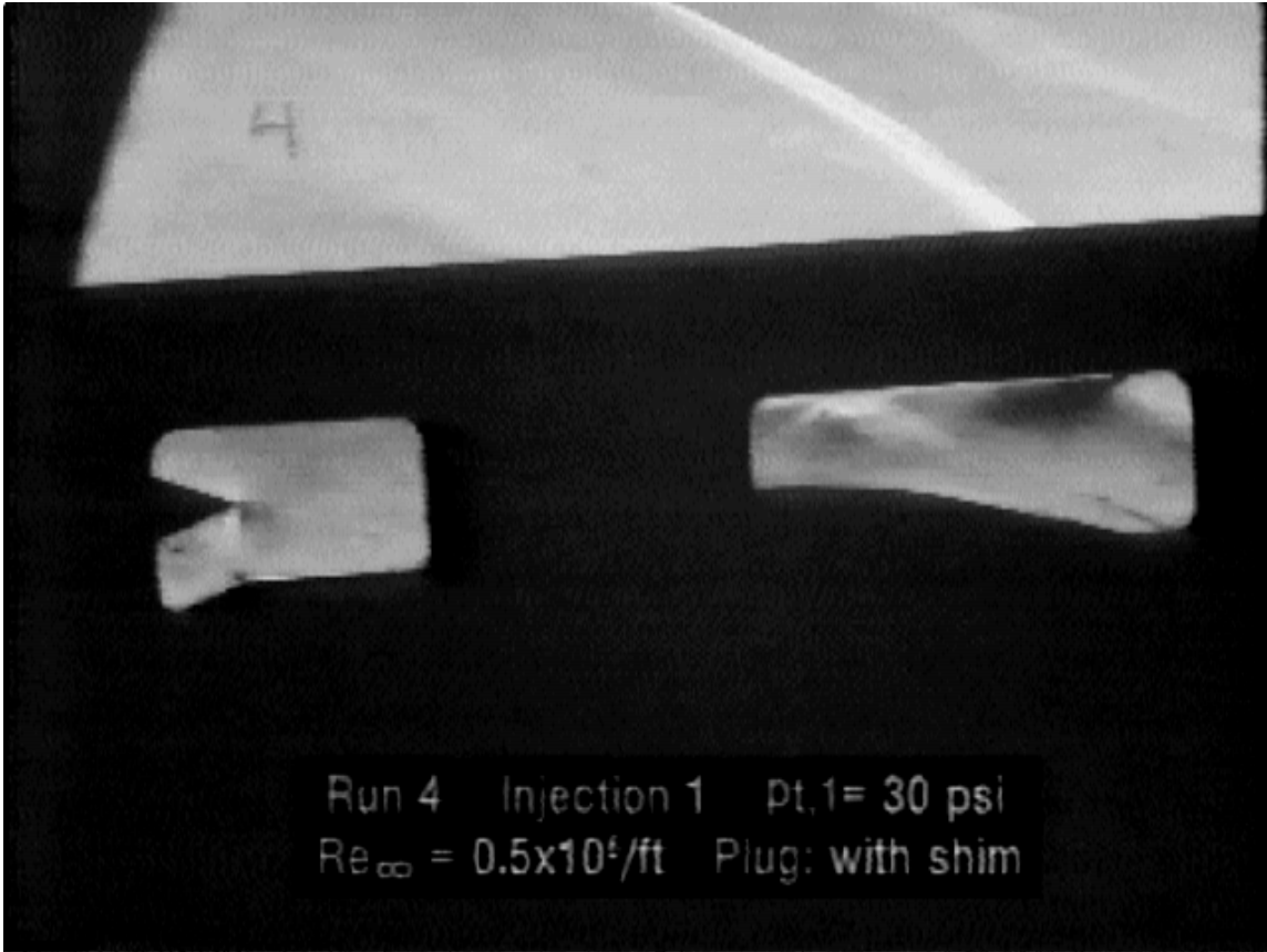
Figure 10: Still Frame from Schlieren Video of Unstarted Inlet in Run 4, Injection 1 Re_{\infty}=0.5 million/ft, pt,1=30 psi, Plug Configuration: with Shim Inlet Configuration: Cowl Down, Plug Forward.
