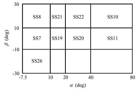
Figure 8 Lateral/Directional Subspaces, Power Off
