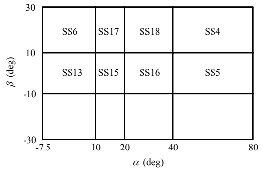
Figure 6 Longitudinal Subspaces, Power Off
