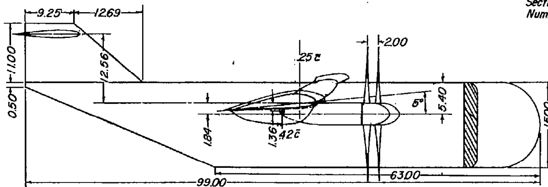
Figure 2.- Drawing of model. All dimensions are in inches.
