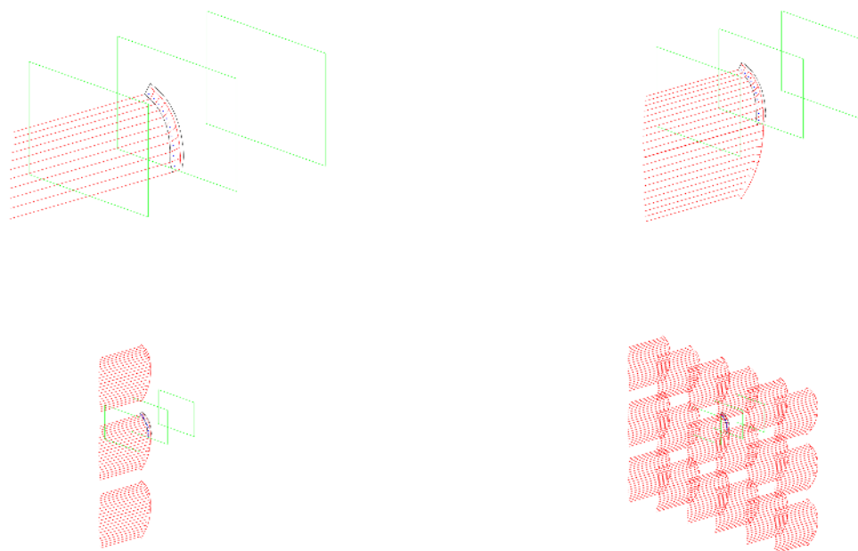
Figure 7. Illustration of the use of mirror images model walls. Upper left: Vortex system of physical wing only. The tunnel is outlined in green. Upper right: Vortex system of physical wing and mounting wall vortex systems. This corresponds to what is modelled in all other codes. Lower left: Vortex system of the nearest mirror images from two parallel walls. Lower right: Vortex system from the nearest mirror images due to all four tunnel walls.
