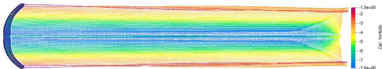
Figure 6. MIRAS simulation of the c-shape configuration with the free filament wake model.
