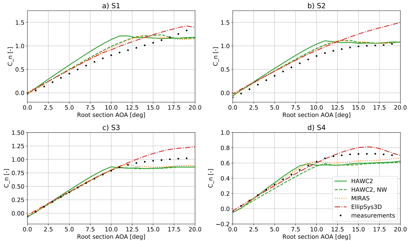
Figure 14. Comparison of measured and simulated c_n at the four instrumented sections, tripped airfoils.
