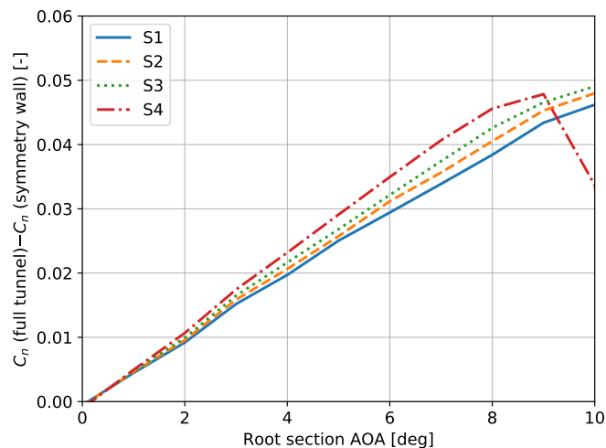
Figure 10. The difference in C_n between the full tunnel configuration and the symmetry wall condition. Computed by the LLTunnel code using clean polars.
