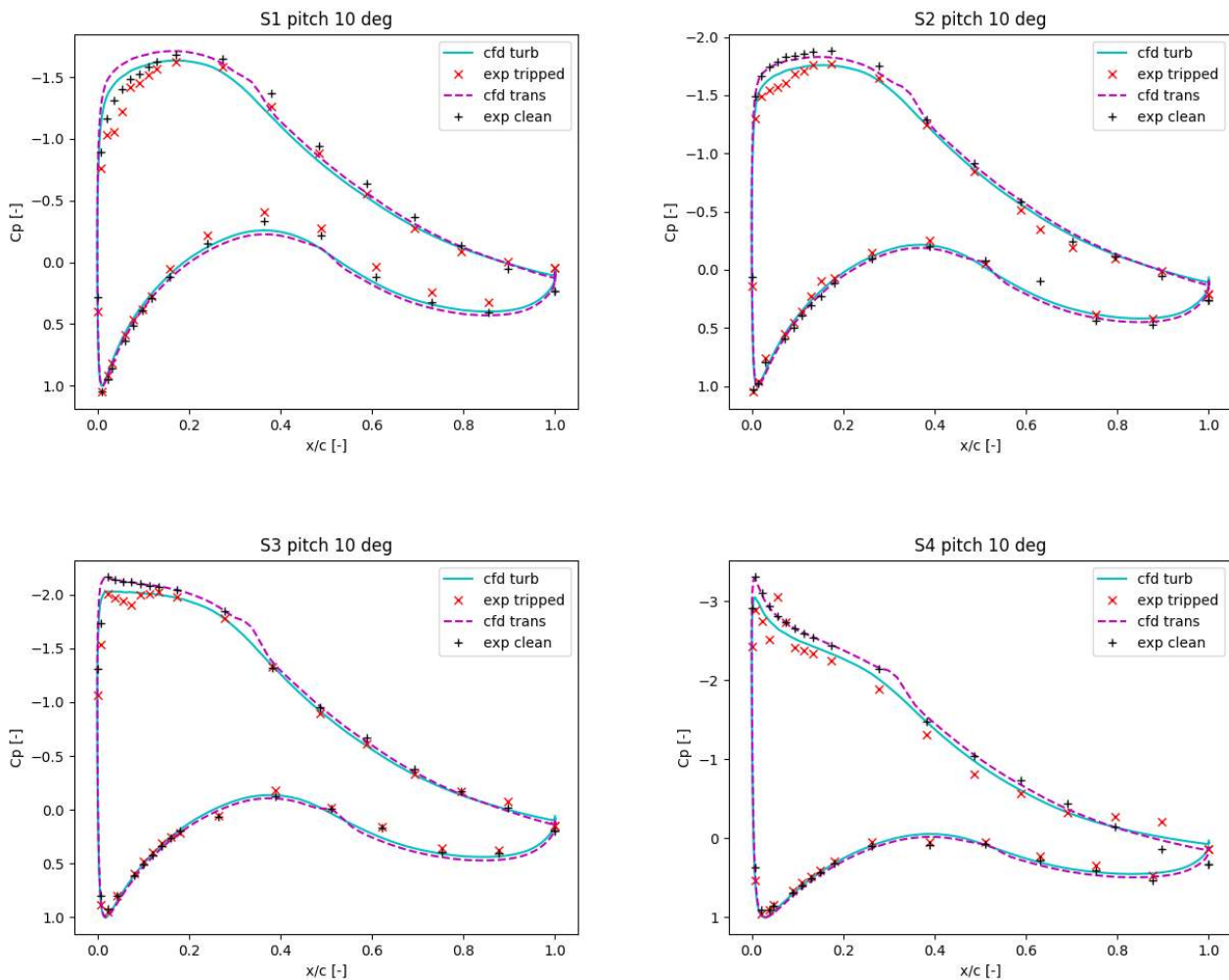
Figure 12. Pressure coefficient C_p distribution, as a function of the normalized chordwise coordinate x/c . Each graph corresponds to a different section of the tip shape (see Figure 4). EllipSys3D fully turbulent results cfd turb , and with transition model cfd trans . For the experimental tests, both clean configuration exp clean and tripped exp tripped are included.
