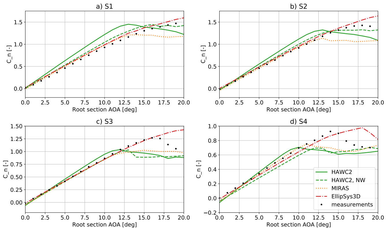
Figure 13. Comparison of measured and simulated c_n at the four instrumented sections, clean airfoils.
