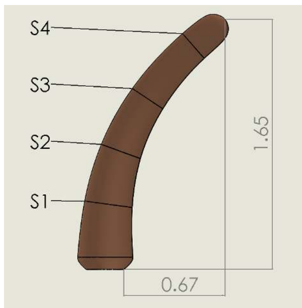
Figure 4. 3D geometry of the tip (in meters), indicating the 4 sections where pressure taps are located.
