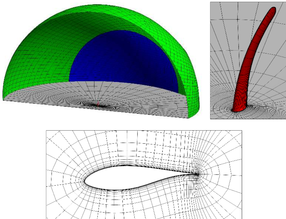
Figure 8. Visualization of the EllipSys3D mesh. For clarity, only one out of every four grid lines is shown, and half of the semi-spherical domain is not depicted. Upper row: overview and detail of the boundary conditions distribution (green for inlet, blue for outlet, grey for symmetry and red for wall). Lower row: cross-sectional mesh around the tip shape, taken at one third of its total projected length (starting from the root).
