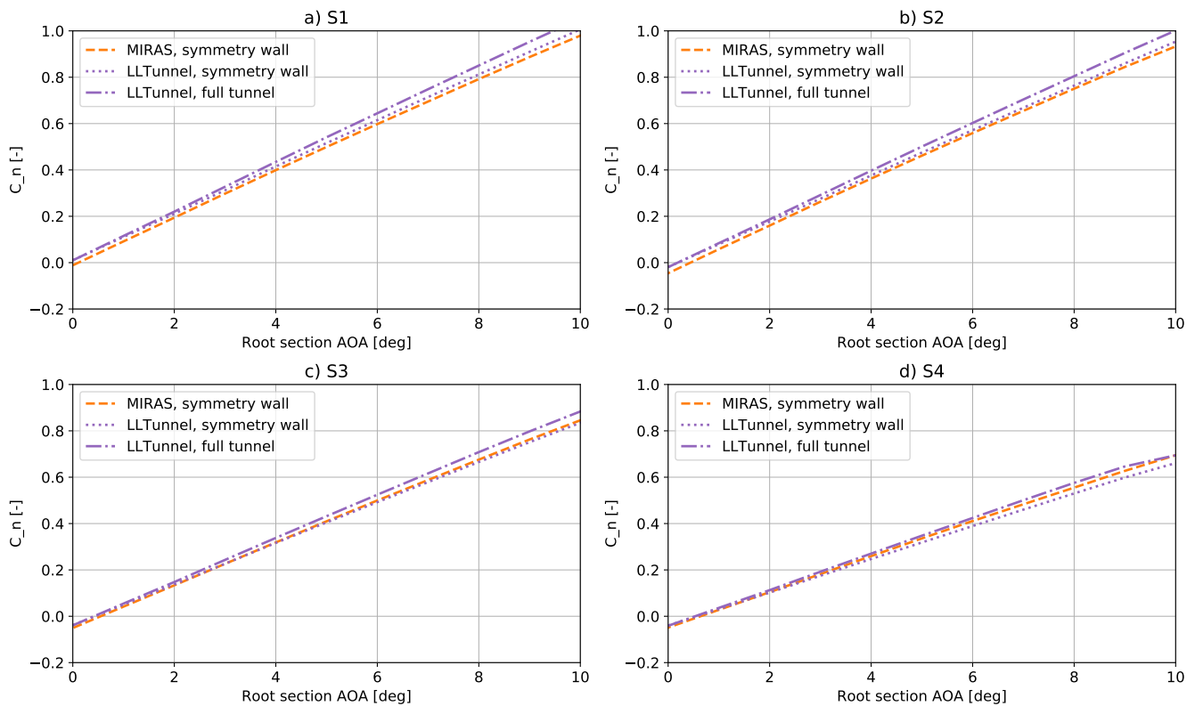
Figure 9. The graphs show MIRAS and LLTunnel C_n values as function of root section AOA for blade sections corresponding to the measurement locations on the wing. Upper left: section 1. Upper right: section 2. Lower left: section 3. Lower right: section 4. MIRAS models the wing on a symmetry wall while LLTunnel models both that configuration and the full tunnel configuration.
