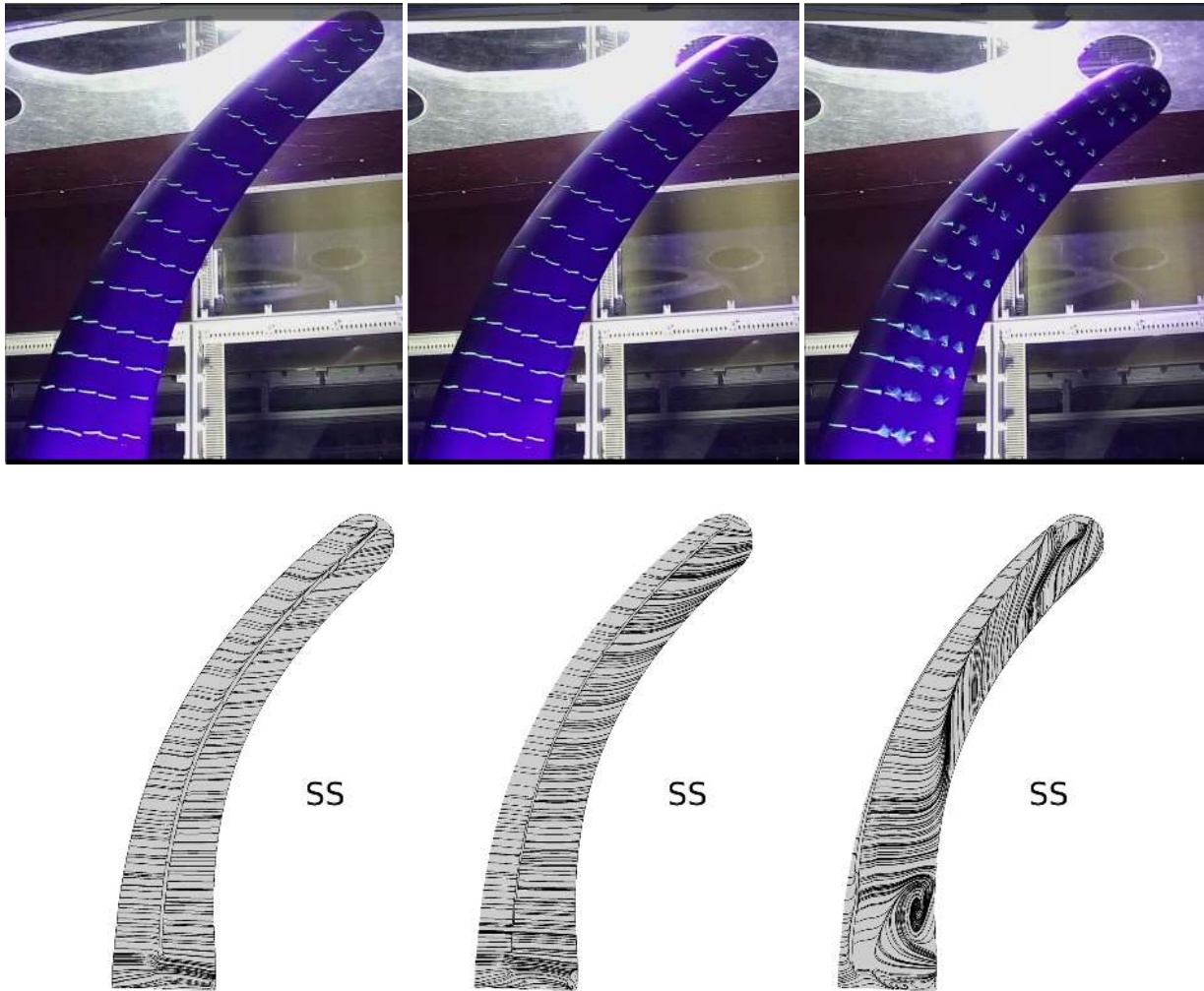
Figure 11. Surface flow visualization. Left column: 0^\circ AOA. Middle column: 10^\circ AOA. Right column: 20^\circ AOA. Upper row: experimental results. Lower row: EllipSys3D.
