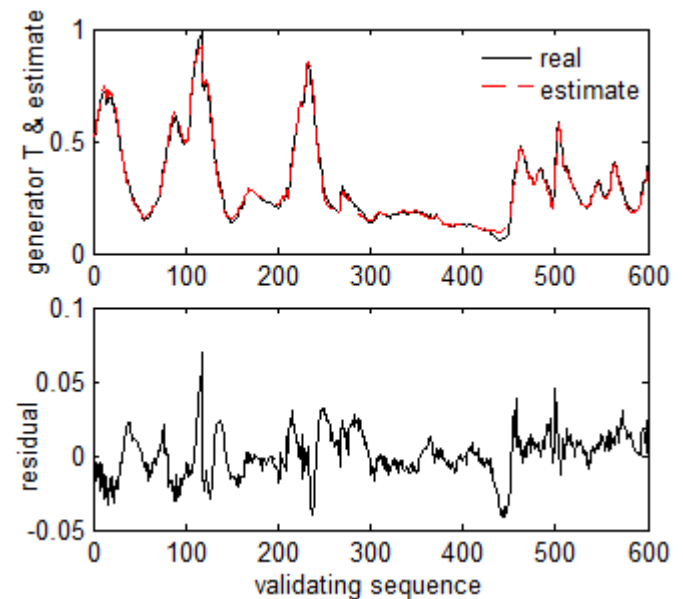
Fig.8 Validation result for artificial neural network
