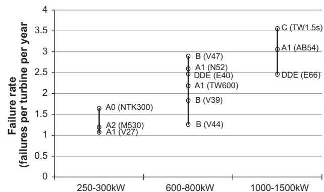
Fig. 12. Distribution of failure rates for WTs of different type and power.
