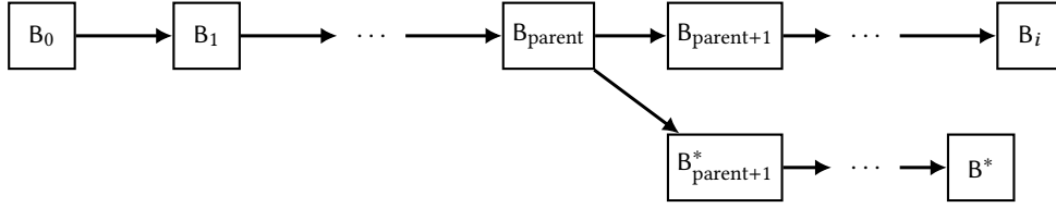
Figure 4: Illustration of an adversarial fork in an attempt to perform a long-range attack
