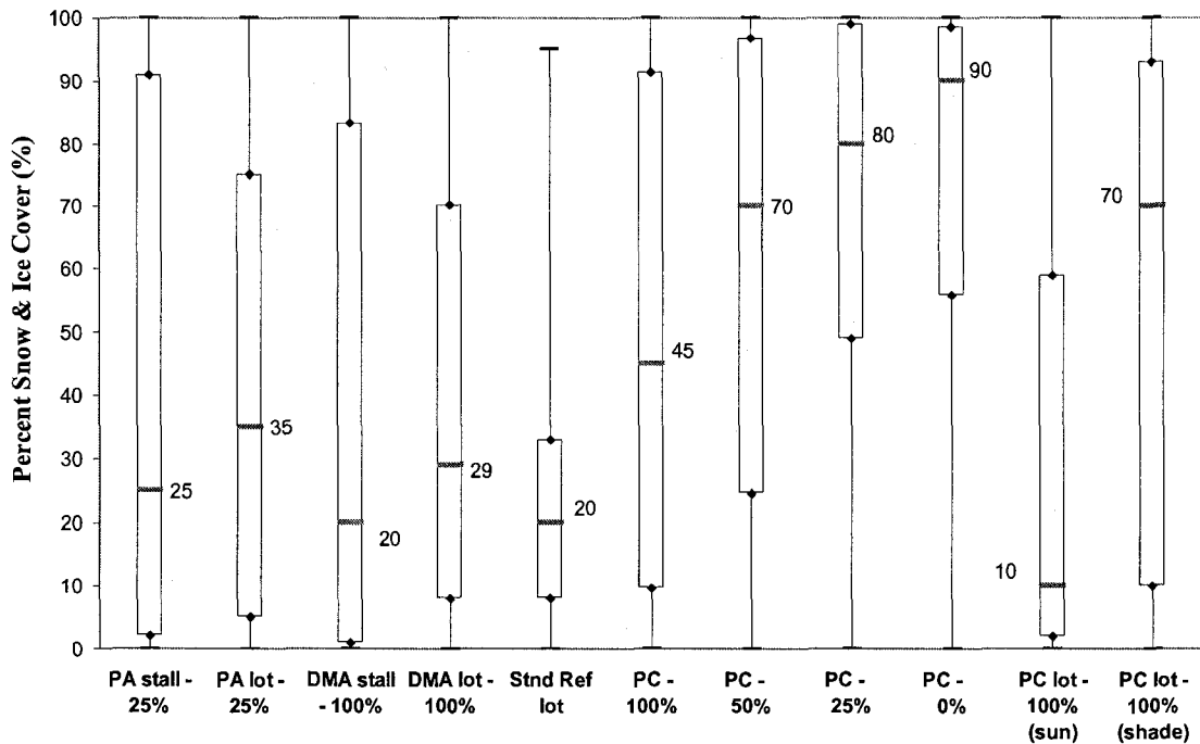
Figure 21: Comparison of snow & ice percent cover for all study areas ('07-'08) (Pavement type and salt application rate as percentage of 3-lbs/sf shown on x-axis)
